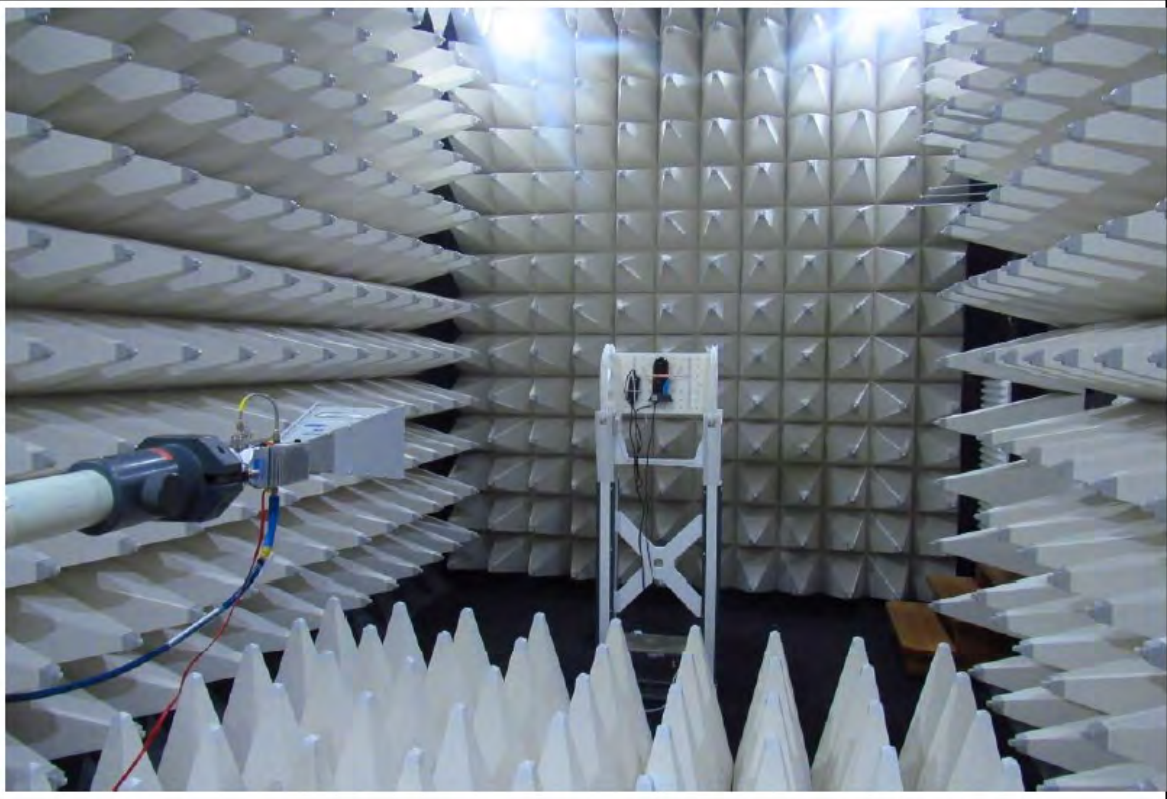
Setup 6.5-18 GHz
