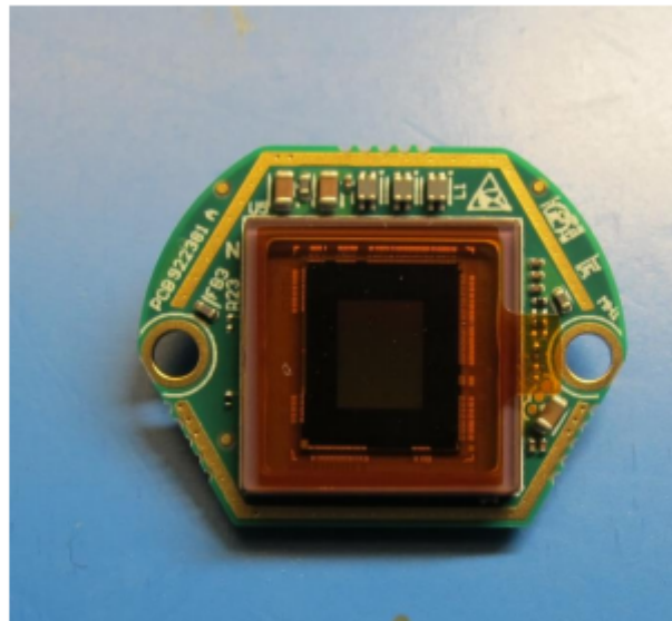
922381_Camera-Board_Portrait_TOP
