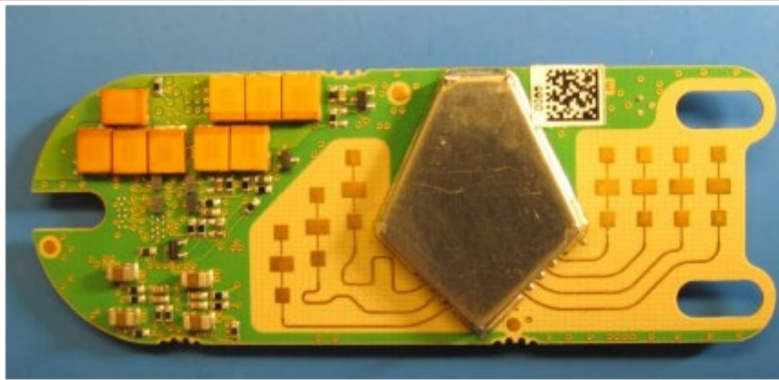
880870_Slave_Radar-Board_TOP
