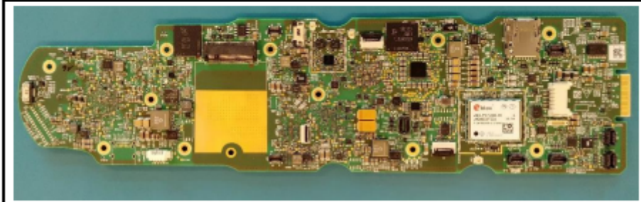
892583_mainboard_top
