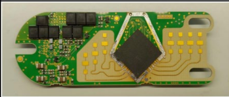
880870_Slave_Radar-Board_TOP without shielding plate
