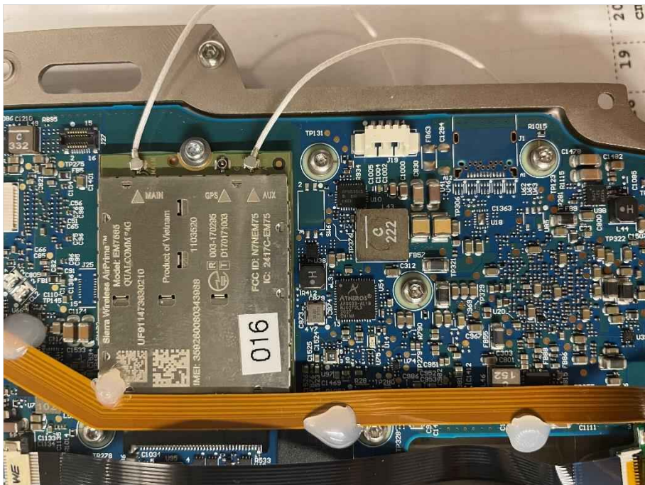
Photograph 4: EUT_Inside view 4
