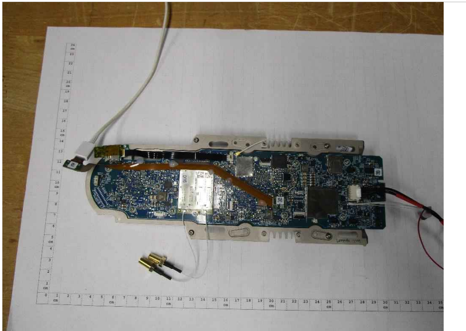
Photograph 1: EUT_Inside view 1
