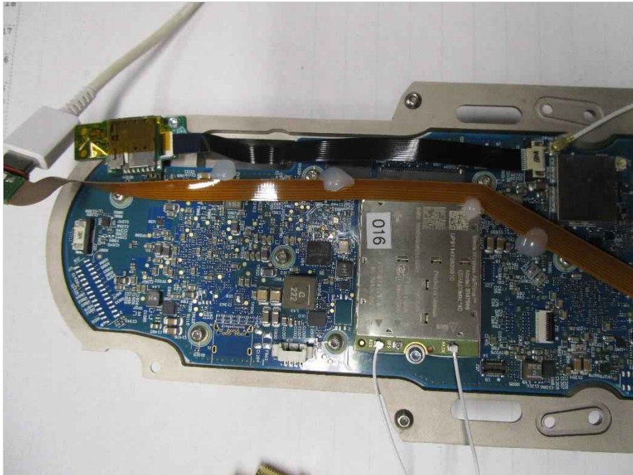
Photograph 3: EUT_Inside view 3
