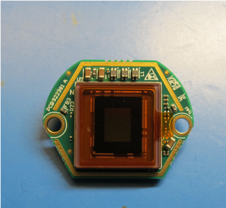
922381_Camera-Board_Portrait_TOP
