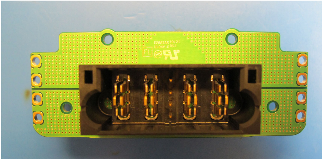
906419_Battery-Connector-Board_TOP
