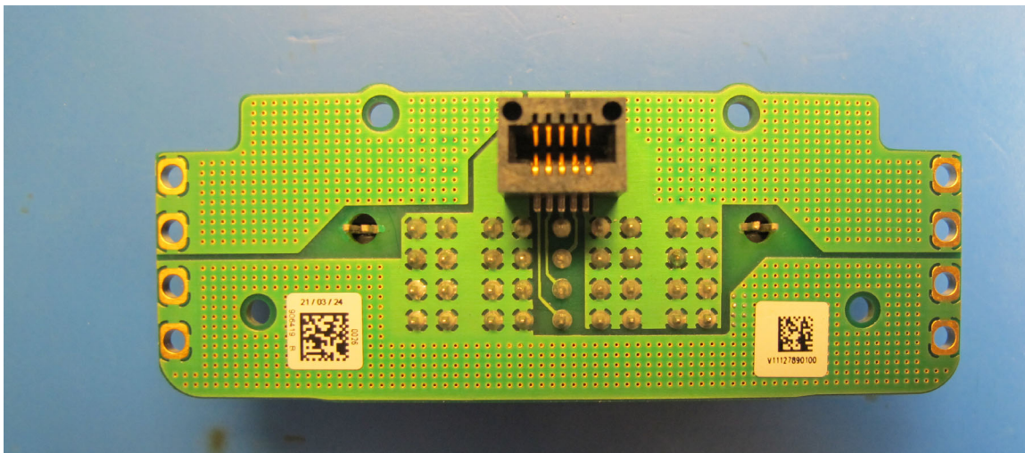
906419_Battery-Connector-Board_BOTTOM
