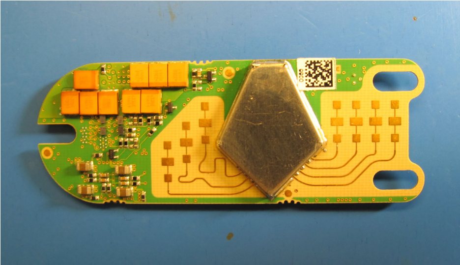
880870_Slave_Radar-Board_TOP-w/o shielding
