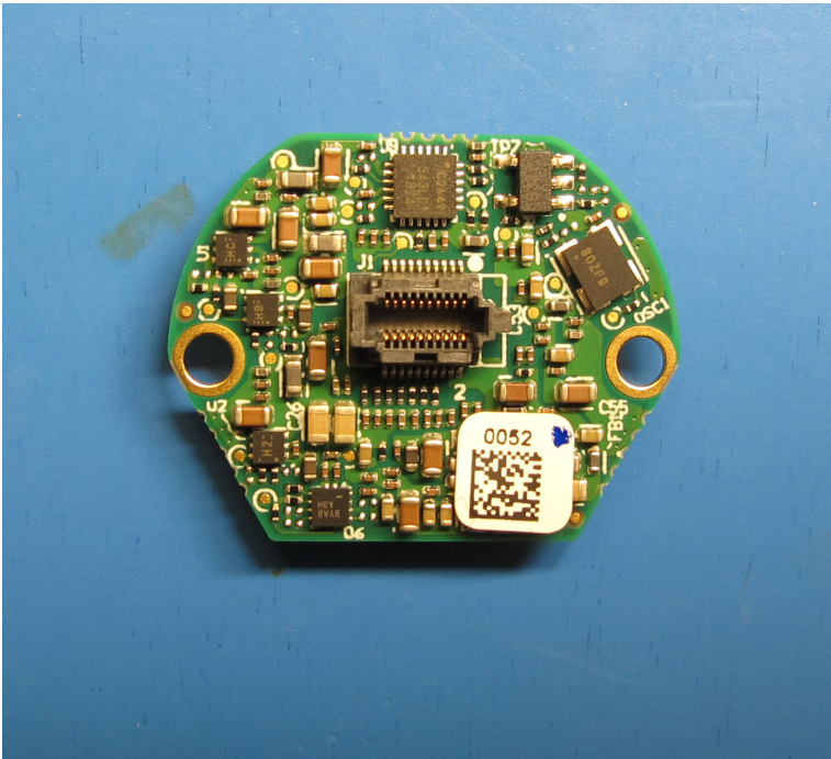
922381_Camera-Board_Portrait_BOTTOM
