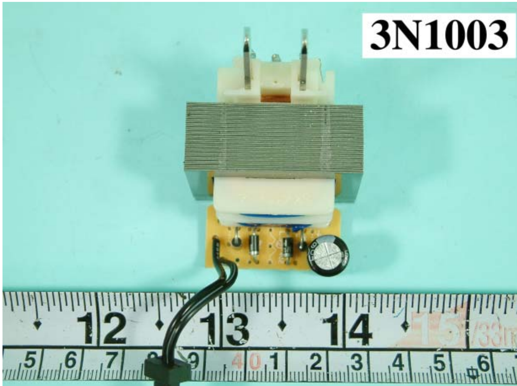
FRONT SIDE OF MAIN BOARD OF ADAPTER
