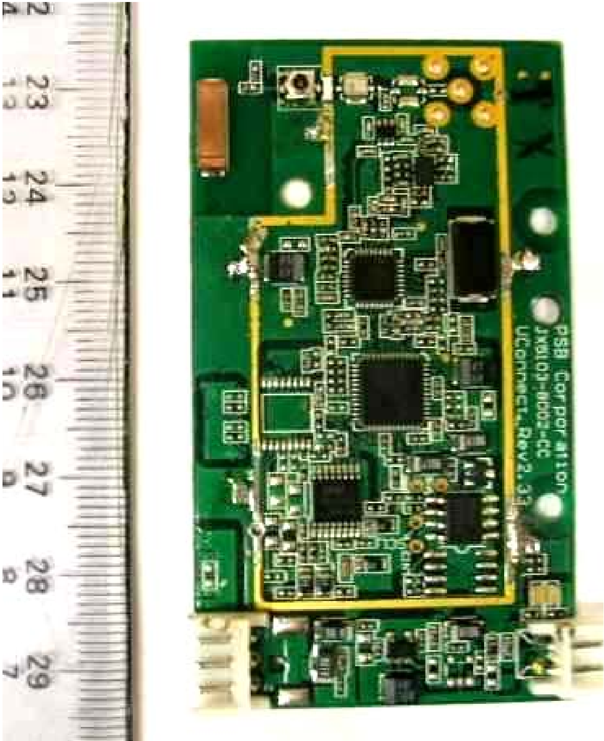
PCB PHOTOGRAPHS FOR SUBWOOFER RF MODULE (RF SHIELD REMOVED)
