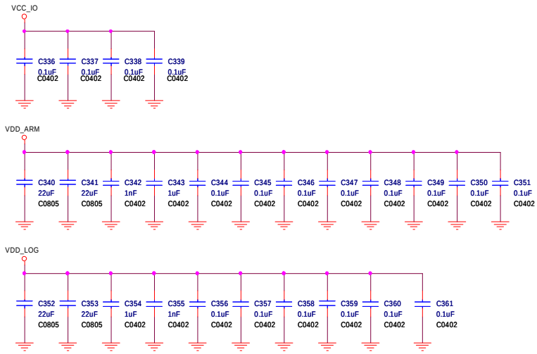
RK3066 CORE POWER FILTER
