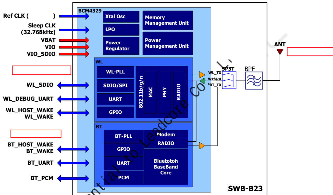
Figure 1-1 SWB-B23 Hardware Block Diagram
