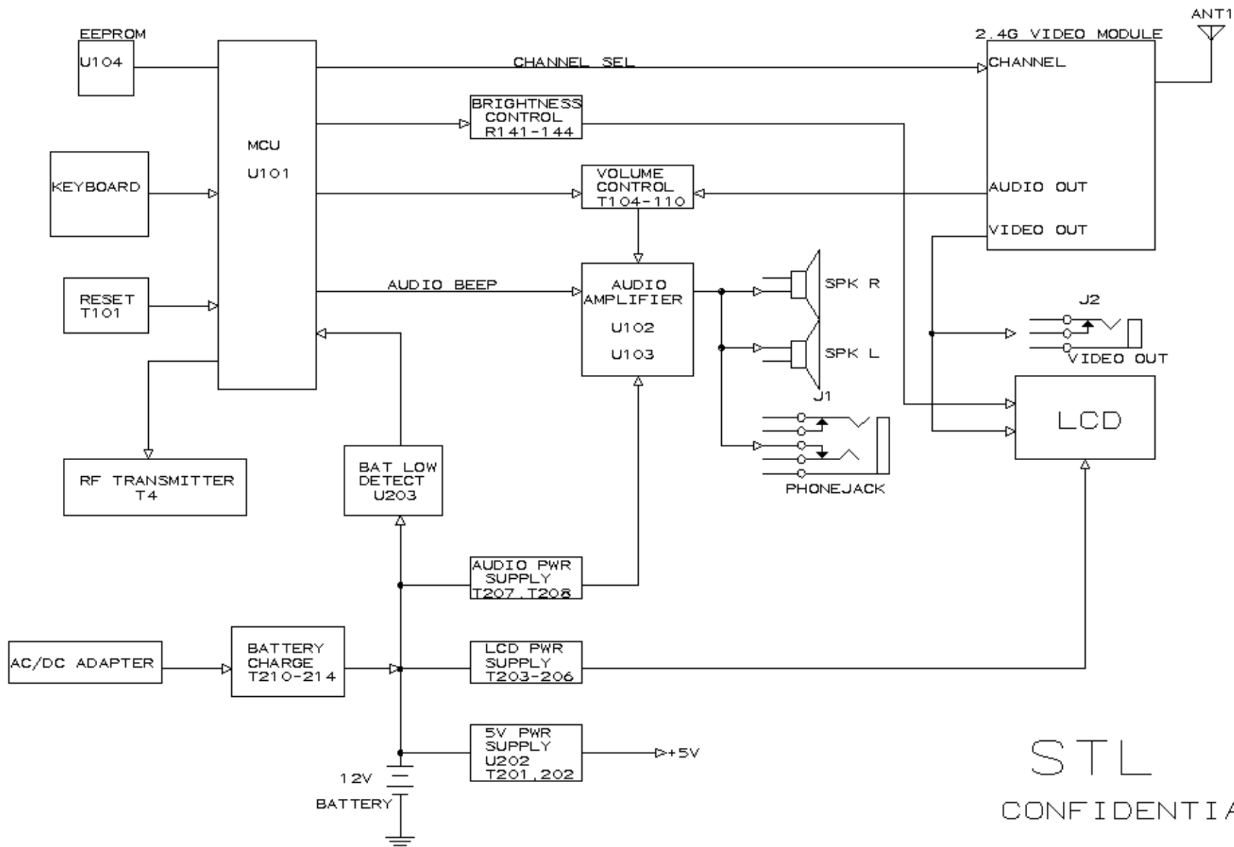
SI654 REMOTE UNIT BLOCK DIAGRAM
