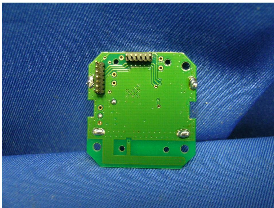
2.4GHz Transceiver Module Main PCB rear side
