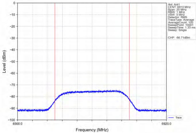
11AX160SISO-Ant 1-6985-Center-6910-Minimal
