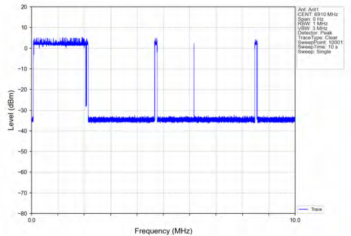
11AX160SISO-Ant 1-6985-Center-6910-Minimal
