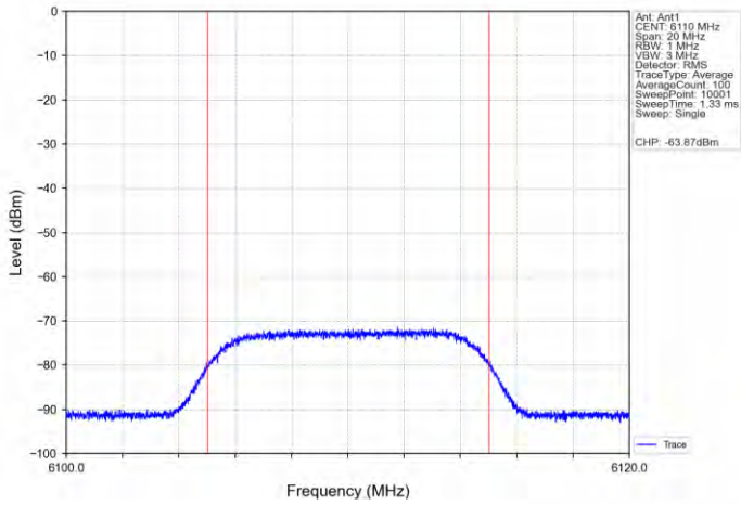
11AX160SISO-Ant 1-6185-Center-6110-Minimal
