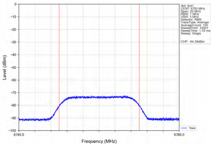
11AX160SISO-Ant 1-6825-Center-6750-Minimal
