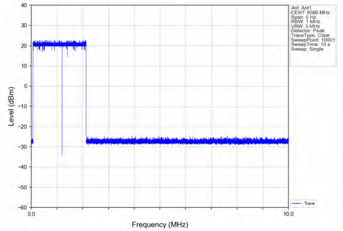
11AX160SISO-Ant 1-6505-Center-6580-Minimal
