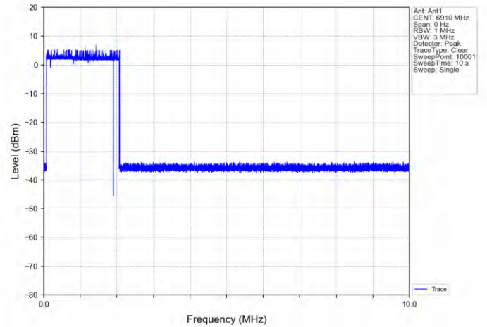
11AX160SISO-Ant 1-6985-Center-6910-Minimal
