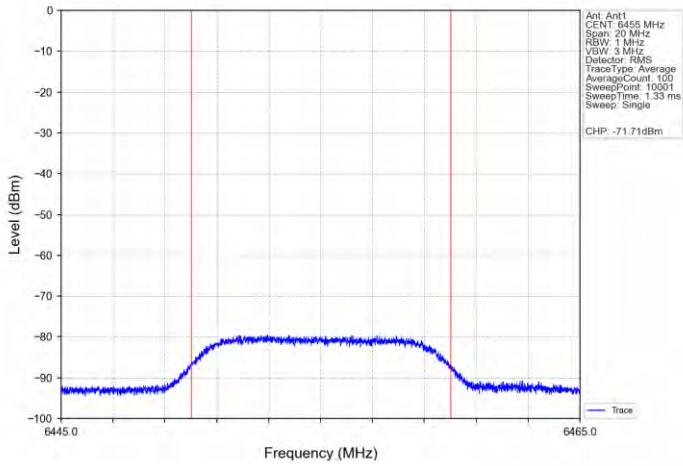
11AX20SISO-Ant 1-6455-Center-6455-Minimal
