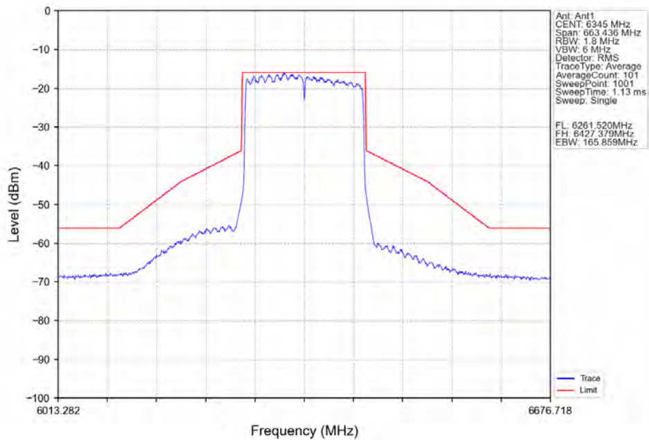
802.11ax(HEW160)_HCH_6345MHz_2xRU996_Left_Ant1_NTNV
