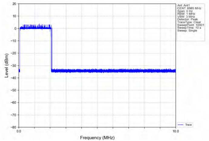
11AX160SISO-Ant 1-6985-Center-6985-Minimal
