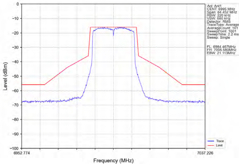
802.11ax(HEW20)_MCH_6995MHz_RU242_Left_Ant5_NTNV
