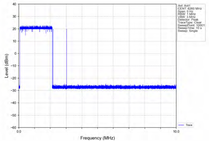
11AX160SISO-Ant 1-6185-Center-6260-Minimal
