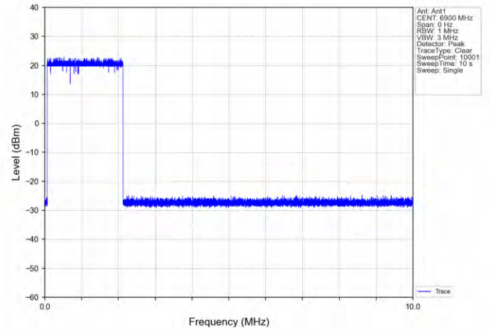
11AX160SISO-Ant 1-6825-Center-6900-Minimal
