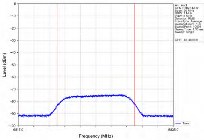
11AX160SISO-Ant 1-6825-Center-6825-Minimal
