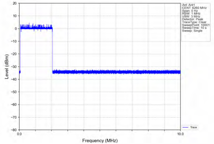
11AX160SISO-Ant 1-6185-Center-6260-Minimal
