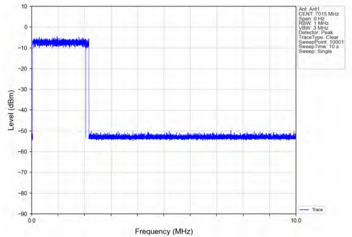
11AX20SISO-Ant 1-7015-Center-7015-Minimal
