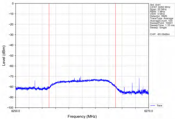
11AX160SISO-Ant 1-6185-Center-6260-Minimal
