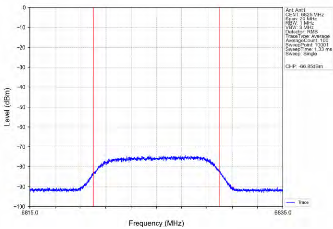
11AX160SISO-Ant 1-6825-Center-6825-Minimal
