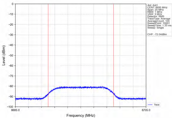
11AX20SISO-Ant 1-6695-Center-6695-Minimal
