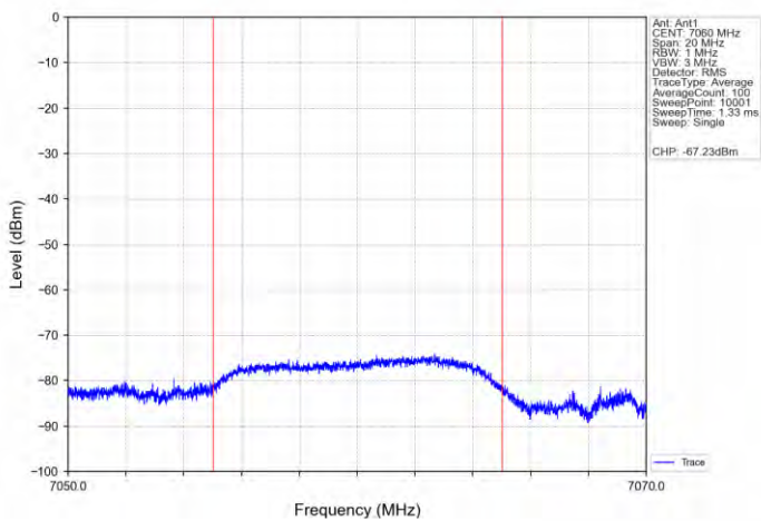
11AX160SISO-Ant 1-6985-Center-7060-Minimal
