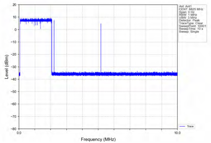
11AX160SISO-Ant 1-6825-Center-6825-Minimal
