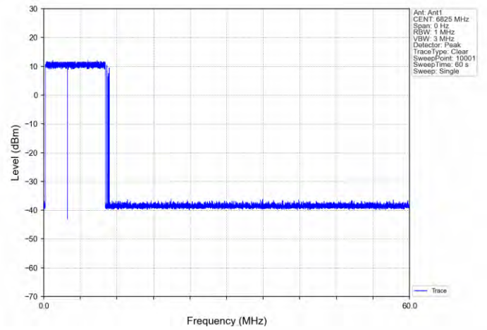
11AX160SISO-Ant 1-6825-Center-6825-Minimal
