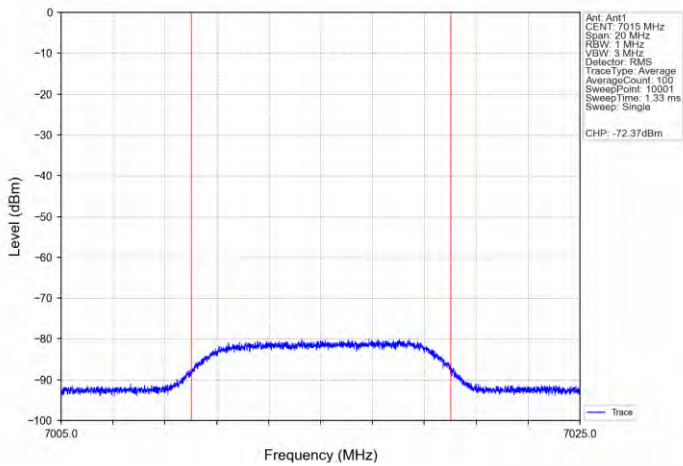
11AX20SISO-Ant 1-7015-Center-7015-Minimal
