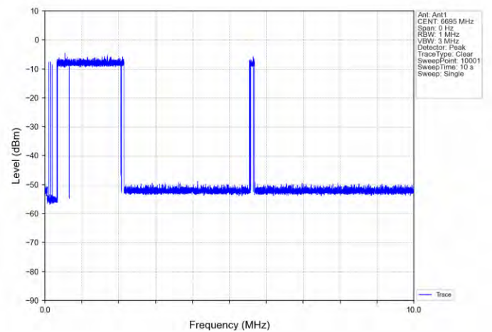
11AX20SISO-Ant 1-6695-Center-6695-Minimal
