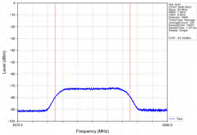
11AX160SISO-Ant 1-6505-Center-6580-Minimal
