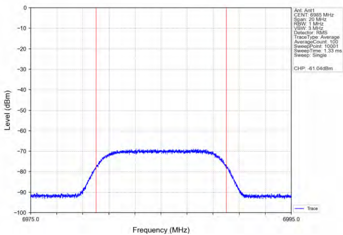
11AX160SISO-Ant 1-6985-Center-6985-Minimal
