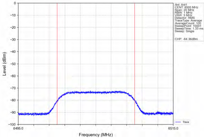
11AX160SISO-Ant 1-6505-Center-6505-Minimal
