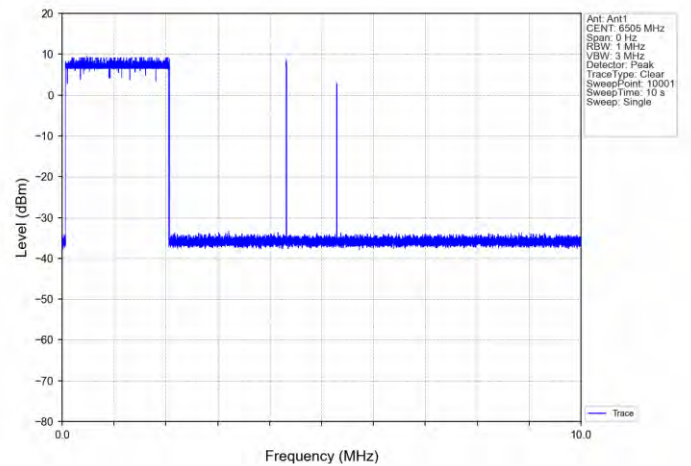
11AX160SISO-Ant 1-6505-Center-6505-Minimal
