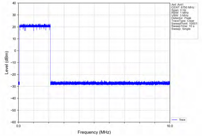
11AX160SISO-Ant 1-6825-Center-6750-Minimal
