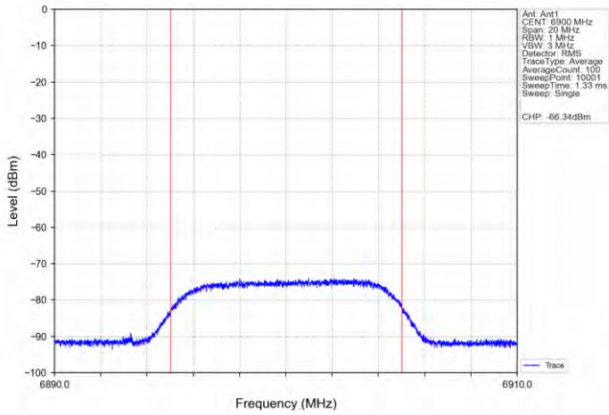
11AX160SISO-Ant 1-6825-Center-6900-Minimal
