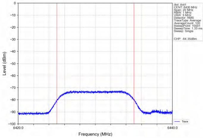
11AX160SISO-Ant 1-6505-Center-6430-Minimal
