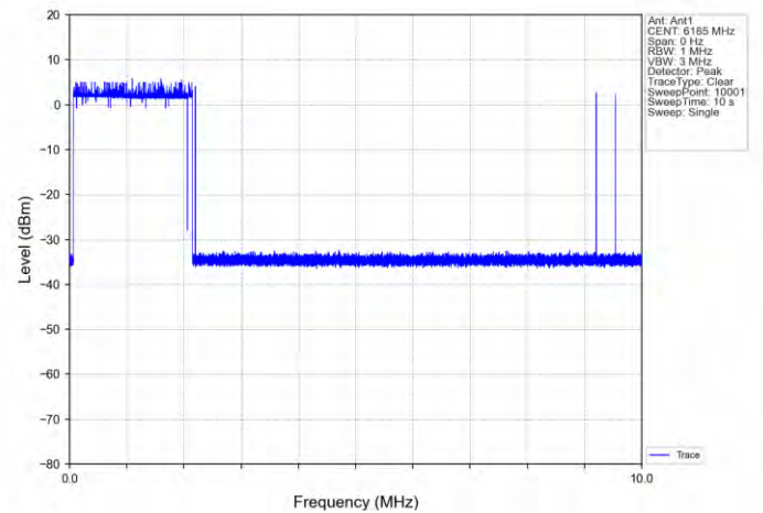
11AX160SISO-Ant 1-6185-Center-6185-Minimal
