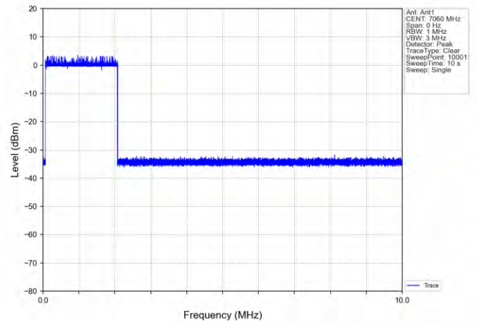
11AX160SISO-Ant 1-6985-Center-7060-Minimal
