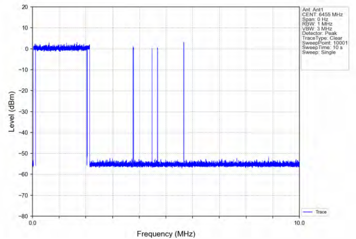
11AX20SISO-Ant 1-6455-Center-6455-Minimal
