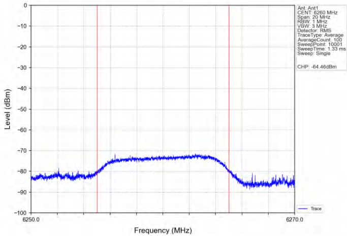
11AX160SISO-Ant 1-6185-Center-6260-Minimal
