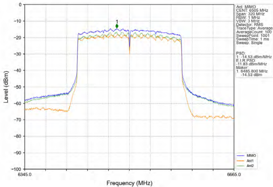
802.11ax(HEW160)_HCH_6505MHz_2xRU996_Left_MIMO_NTNV
