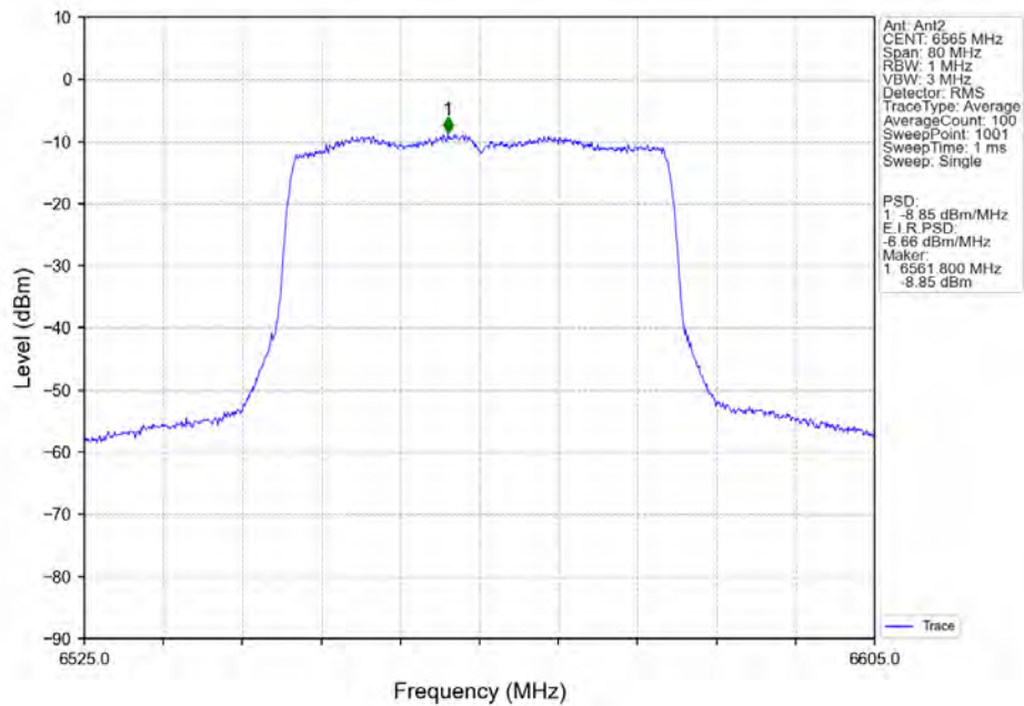
802.11ax(HEW40)_LCH_6565MHz_RU484_Left_MIMO_NTNV
