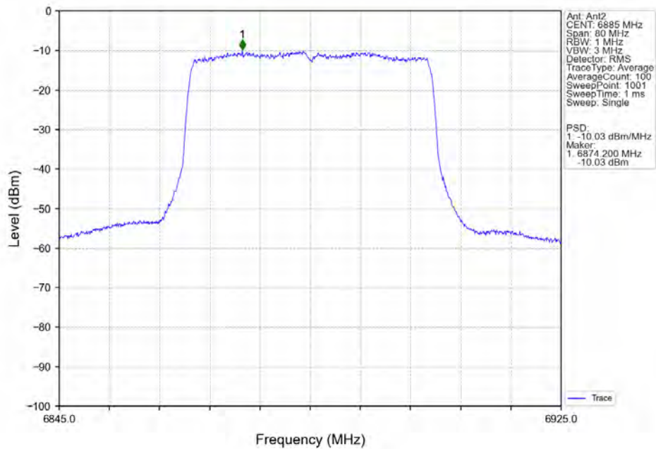
802.11ax(HEW40)_HCH_6885MHz_RU484_Left_MIMO_NTNV
