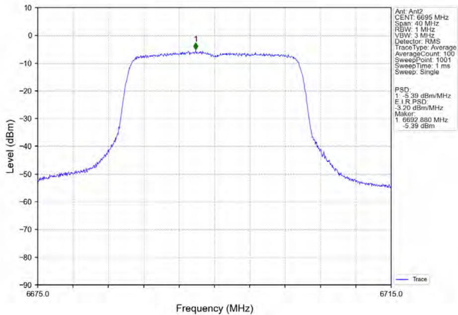
802.11ax(HEW20)_MCH_6695MHz_RU242_Left_MIMO_NTNV
