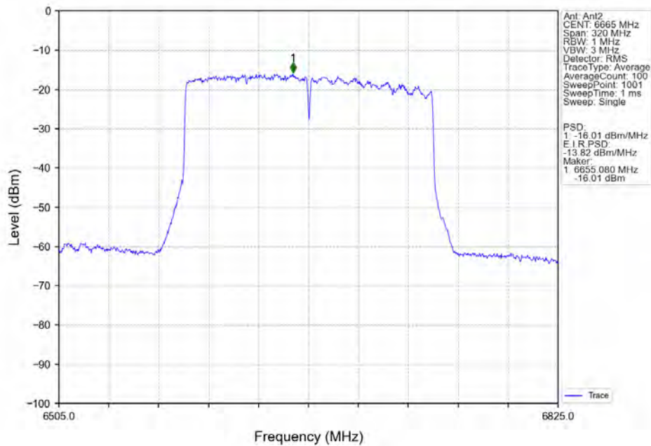
802.11ax(HEW160)_MCH_6665MHz_2xRU996_Left_MIMO_NTNV
