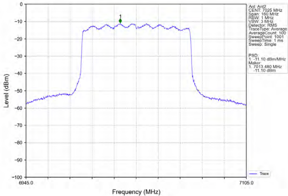
802.11ax(HEW80)_HCH_7025MHz_RU996_Left_MIMO_NTNV
