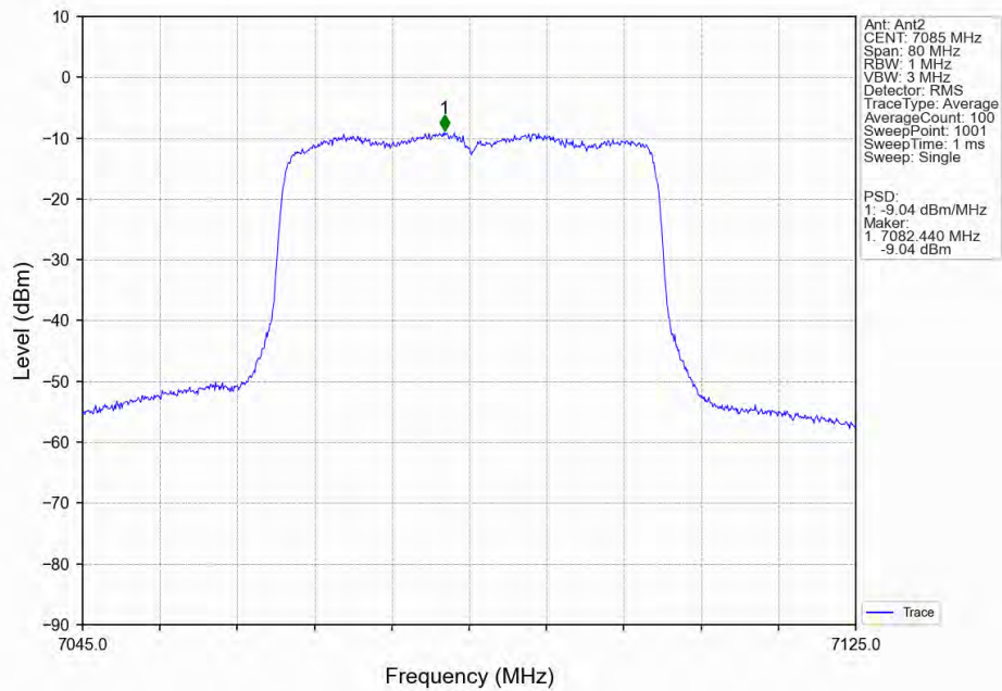
802.11ax(HEW40)_HCH_7085MHz_RU484_Left_MIMO_NTNV
