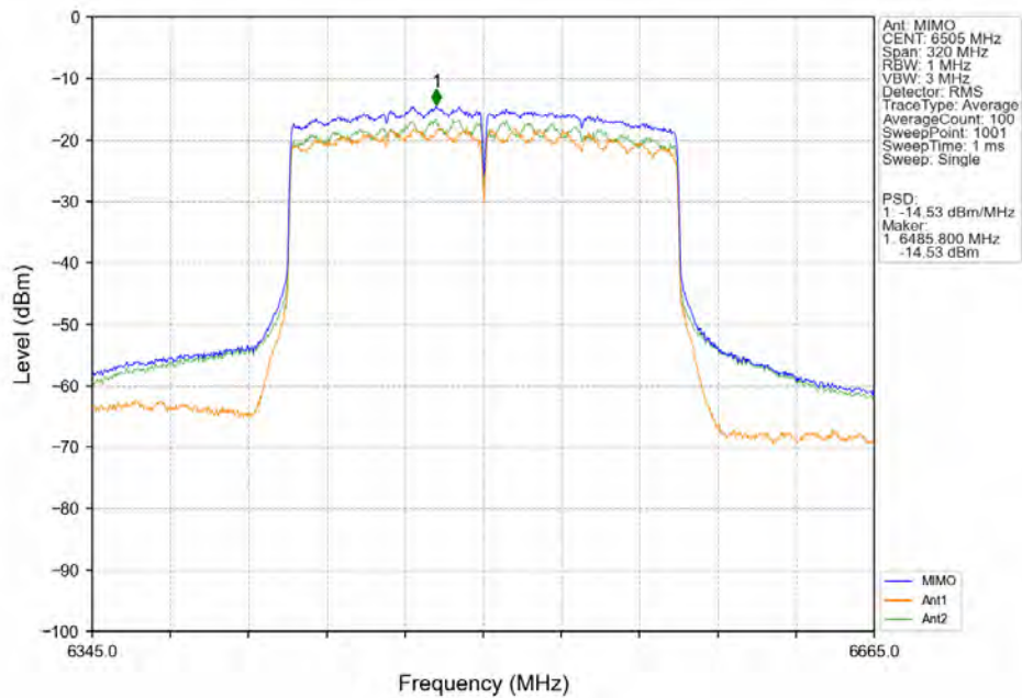
802.11ax(HEW160)_HCH_6505MHz_2xRU996_Left_MIMO_NTNV
