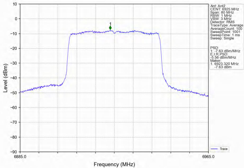
802.11ax(HEW40)_LCH_6925MHz_RU484_Left_MIMO_NTNV
