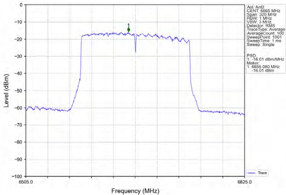
802.11ax(HEW160)_MCH_6665MHz_2xRU996_Left_MIMO_NTNV
