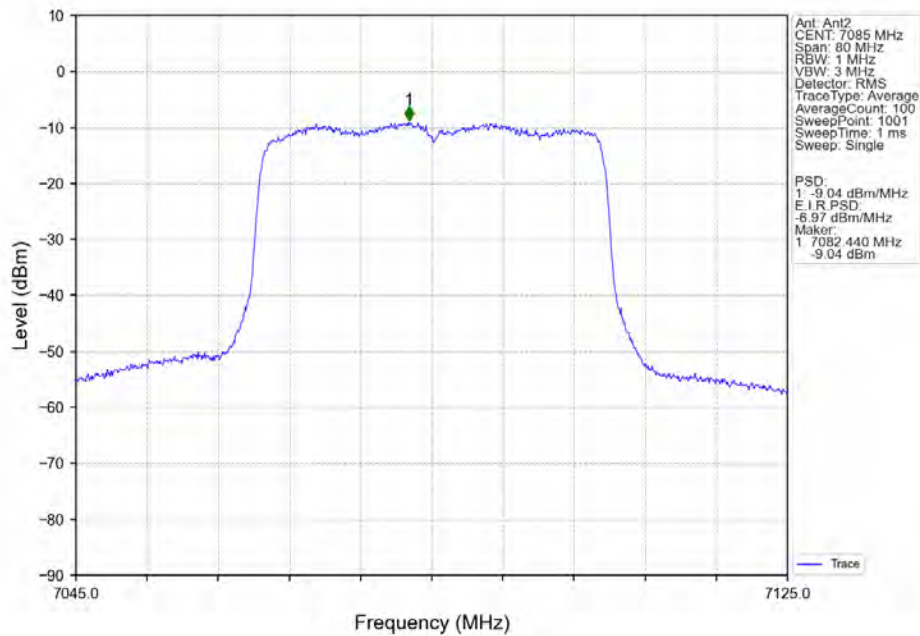
802.11ax(HEW40)_HCH_7085MHz_RU484_Left_MIMO_NTNV
