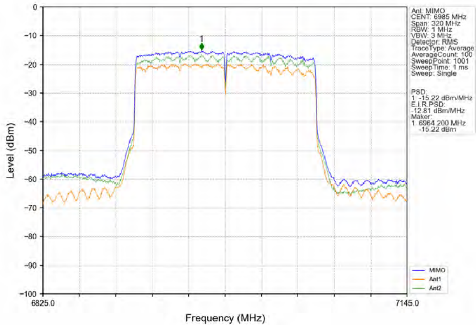
802.11ax(HEW160)_MCH_6985MHz_2xRU996_Left_MIMO_NTNV
