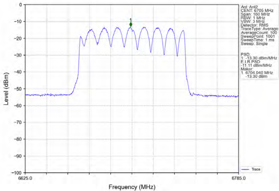
802.11ax(HEW80)_MCH_6705MHz_RU996_Left_MIMO_NTNV
