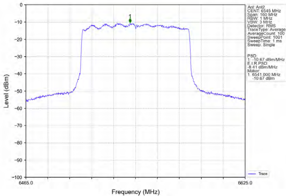
802.11ax(HEW80)_HCH_6545MHz_RU996_Left_MIMO_NTNV
