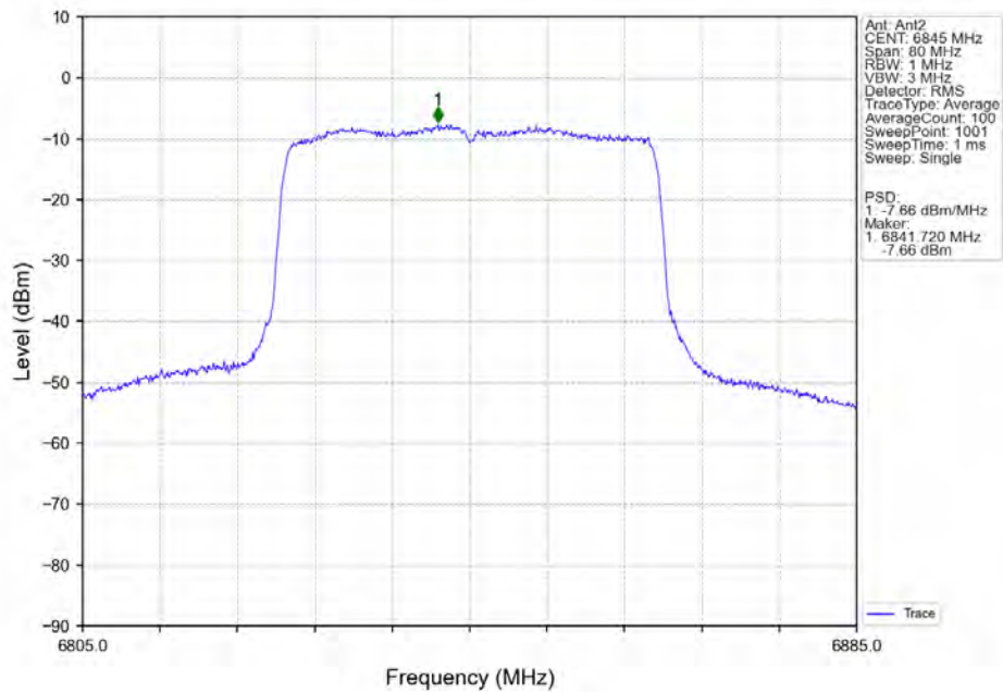
802.11ax(HEW40)_HCH_6845MHz_RU484_Left_MIMO_NTNV
