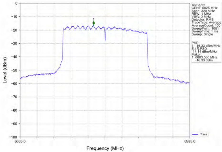
802.11ax(HEW160)_HCH_6825MHz_2xRU996_Left_MIMO_NTNV
