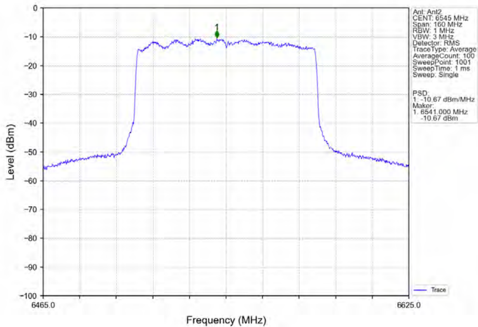
802.11ax(HEW80)_HCH_6545MHz_RU996_Left_MIMO_NTNV
