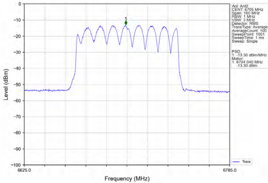
802.11ax(HEW80)_MCH_6705MHz_RU996_Left_MIMO_NTNV
