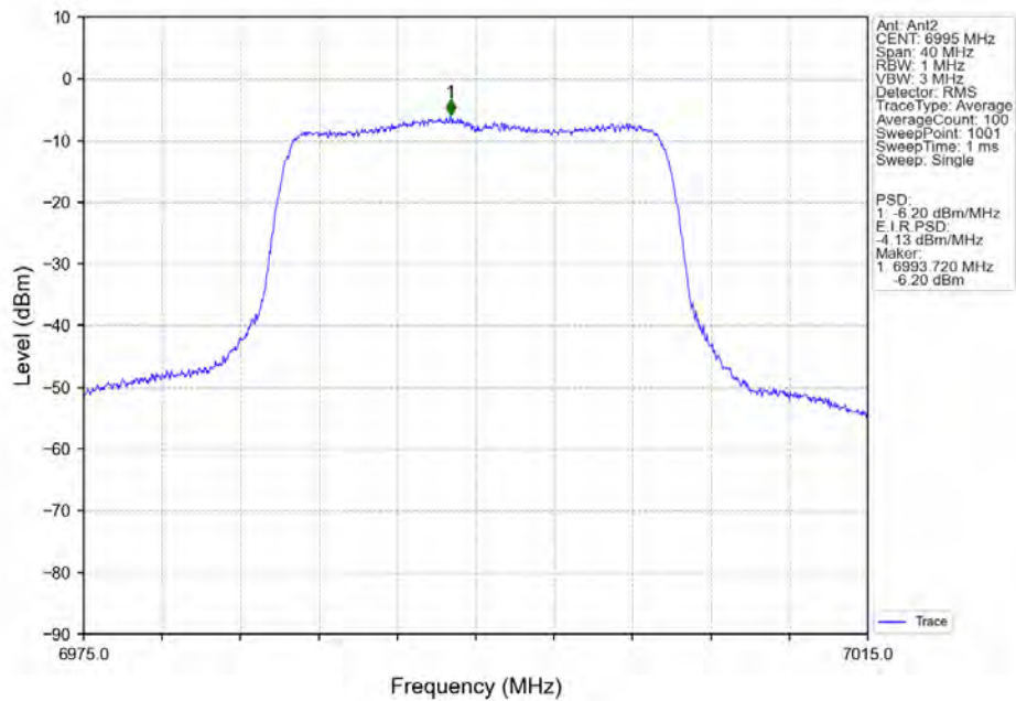
802.11ax(HEW20)_MCH_6995MHz_RU242_Left_MIMO_NTNV
