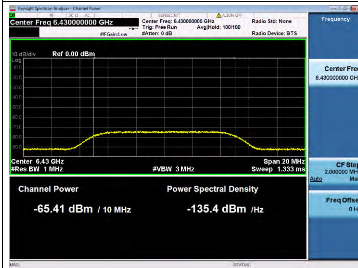
11AX160SISO-Ant 1-6505-Center-6430-Minimal
