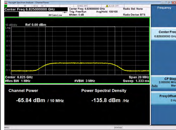
11AX160SISO-Ant 1-6825-Center-6825-Minimal
