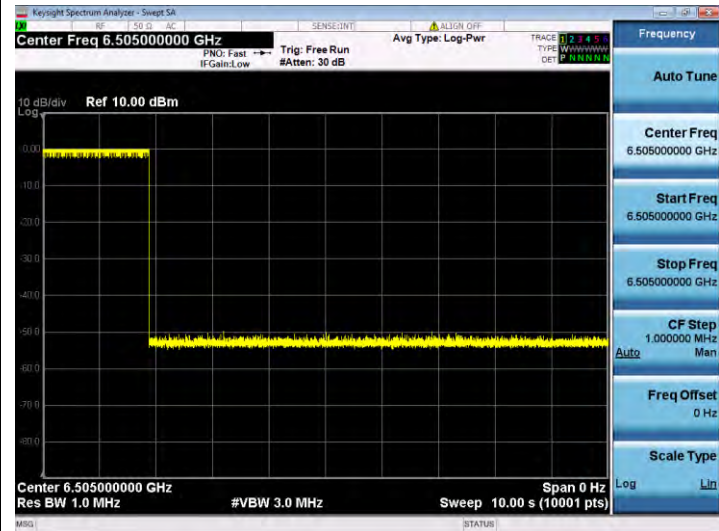
11AX160SISO-Ant 1-6505-Center-6505-Minimal
