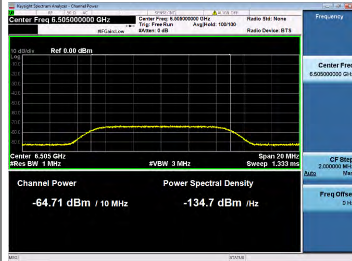
11AX160SISO-Ant 1-6505-Center-6505-Minimal
