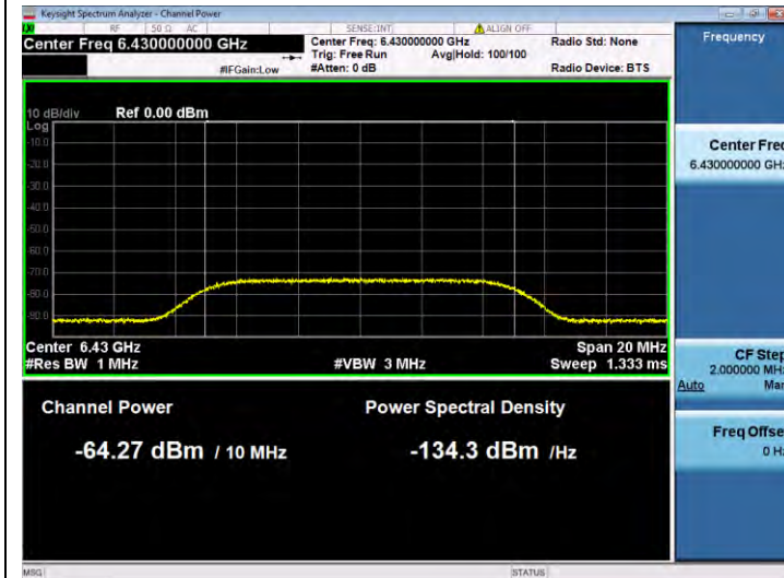
11AX160SISO-Ant 1-6505-Center-6430-Minimal
