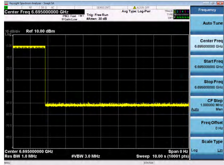
11AX20SISO-Ant 1-6695-Center-6695-Minimal
