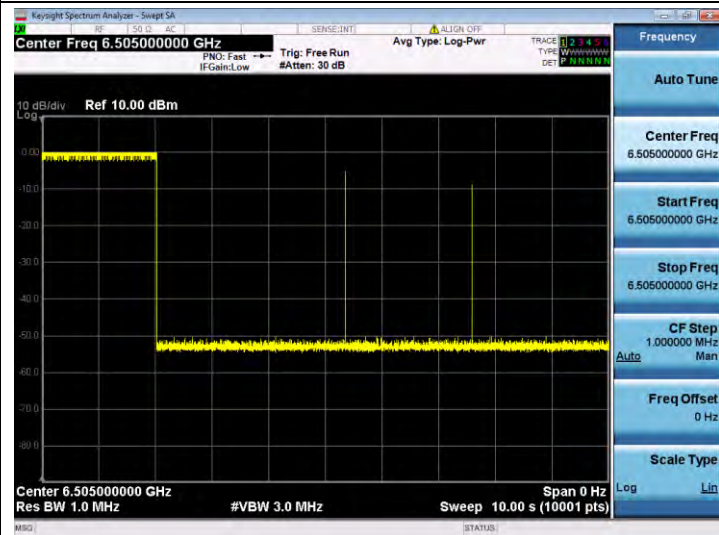
11AX160SISO-Ant 1-6505-Center-6505-Minimal
