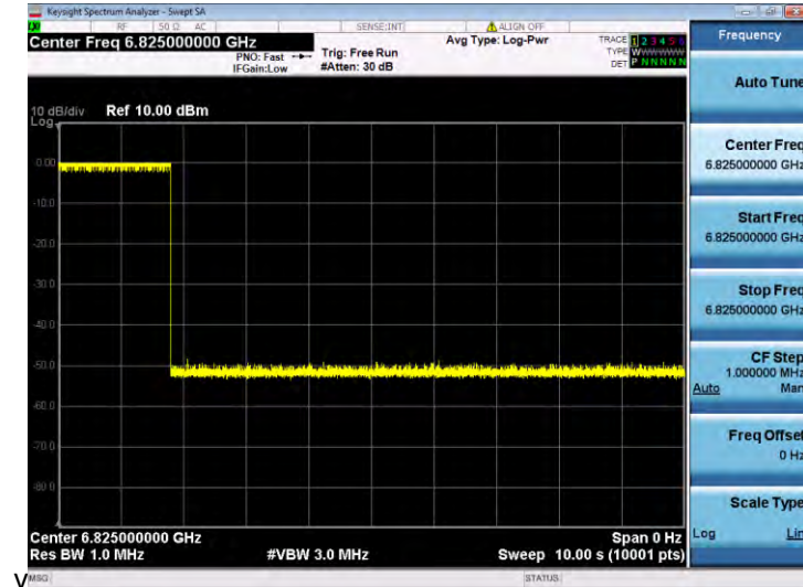
11AX160SISO-Ant 1-6825-Center-6825-Minimal
