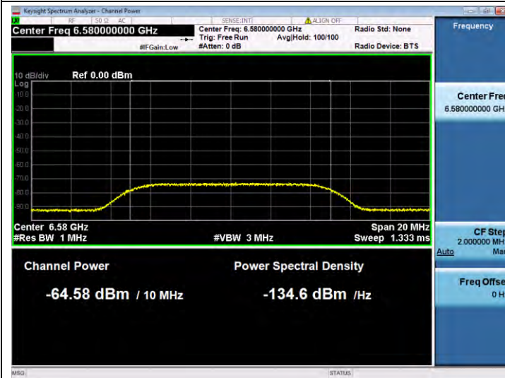
11AX160SISO-Ant 1-6505-Center-6580-Minimal
