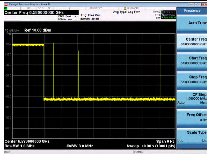
11AX160SISO-Ant 1-6505-Center-6580-Minimal
