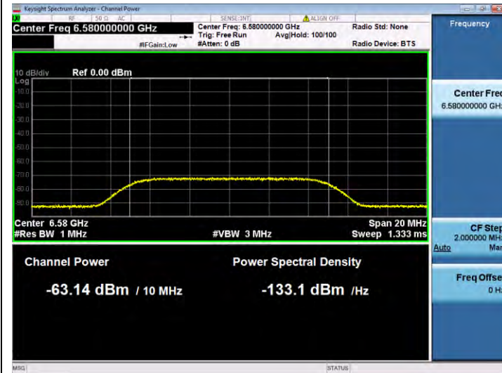
11AX160SISO-Ant 1-6505-Center-6580-Minimal
