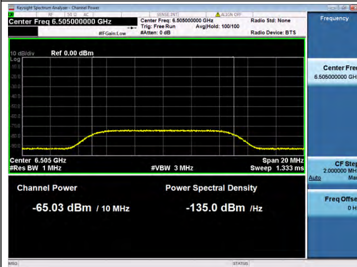
11AX160SISO-Ant 1-6505-Center-6505-Minimal
