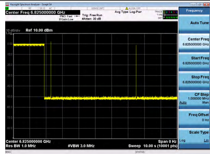
11AX160SISO-Ant 1-6825-Center-6825-Minimal
