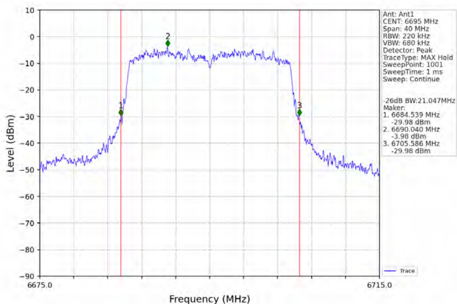
802.11ax(HEW20)_MCH_6695MHz_RU242_Left_Ant1_NTNV
