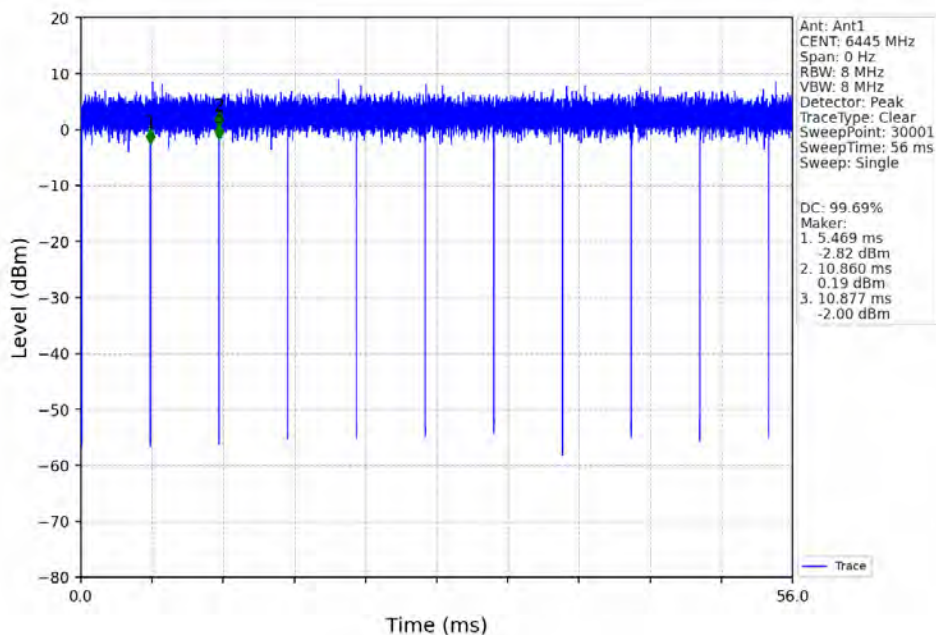
802.11ax(HEW40)_LCH_6445MHz_RU484_Left_Ant1_NTNV
