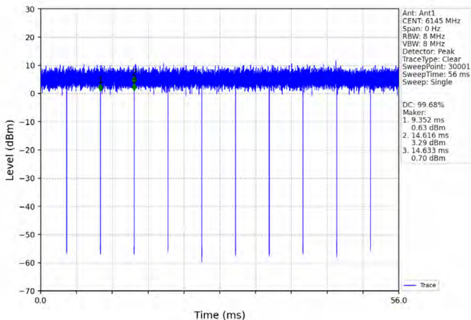
802.11ax(HEW80)_MCH_6145MHz_RU996_Left_Ant1_NTNV
