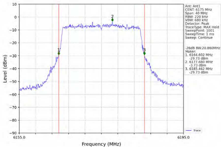
802.11ax(HEW20)_MCH_6175MHz_RU242_Left_Ant1_NTNV
