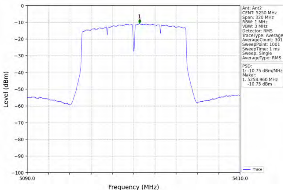
802.11ac(VHT160)_MCH_5250MHz_MIMO_NTNV
