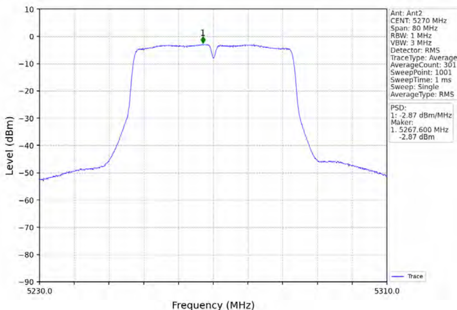
802.11ac(VHT40)_LCH_5270MHz_MIMO_NTNV
