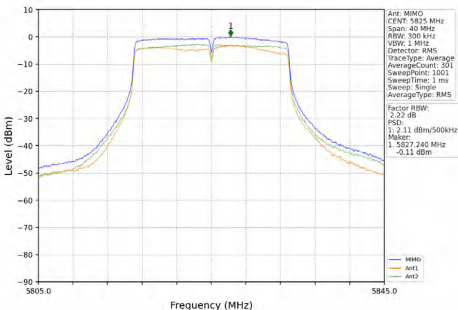
802.11ac(VHT20)_HCH_5825MHz_MIMO_NTNV
