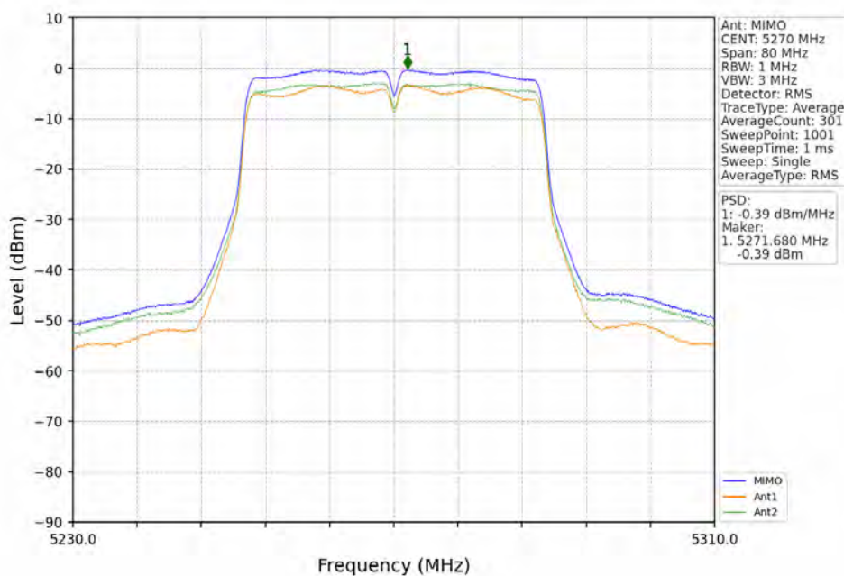
802.11ac(VHT40)_LCH_5270MHz_MIMO_NTNV
