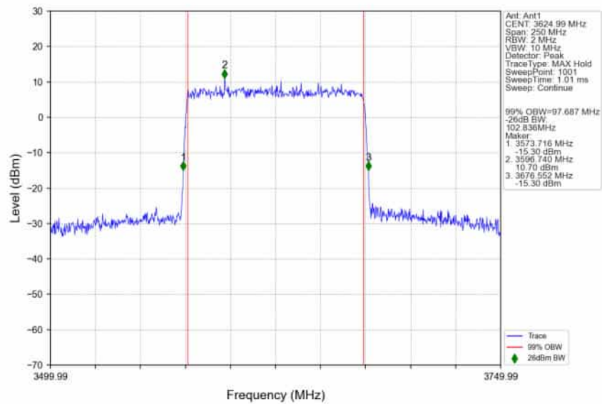
n78d_30kHz_SISO_NTNV_100MHz_CP-OFDM_256_QAM_3624.99MHz_Outer_Full_Ant1
