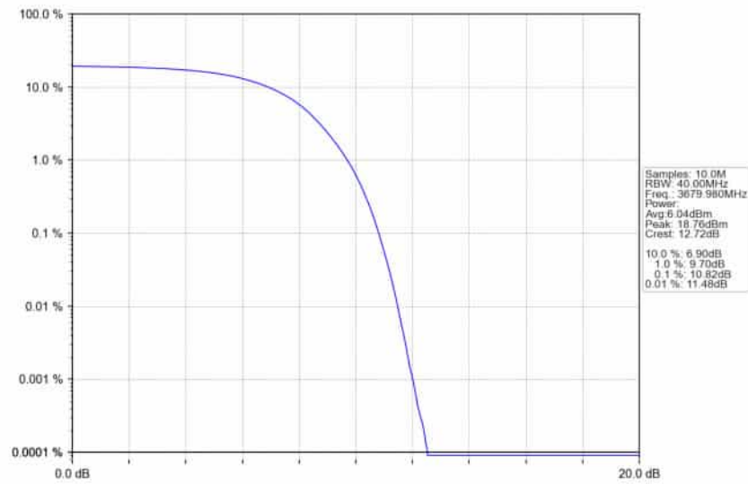
n78d_30kHz_SISO_NTNV_40MHz_DFT-s-OFDM_64_QAM_3679.98MHz_Outer_Full_Ant1
