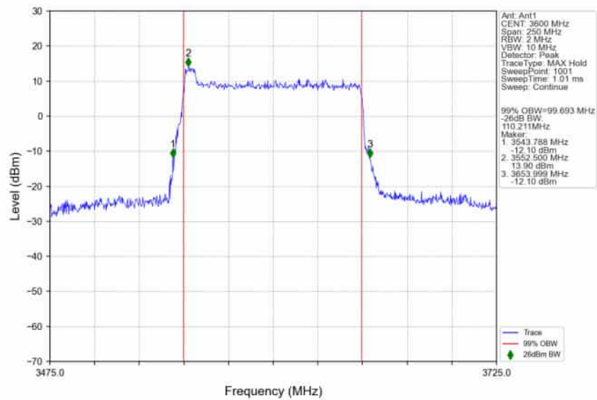
n78d_30kHz_SISO_NTNV_100MHz_CP-OFDM 64 QAM_3600MHz_Outer_Full_Ant1
