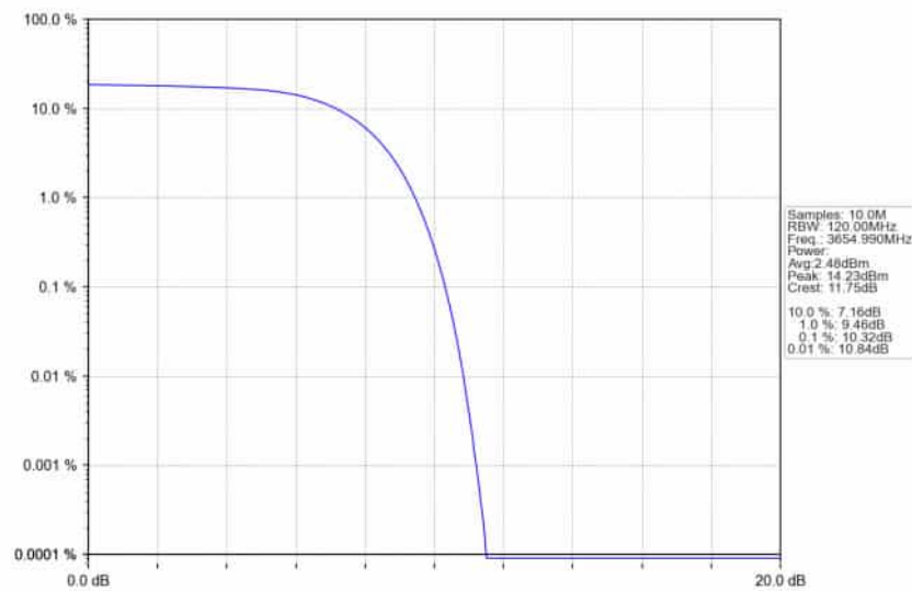
n78d_30kHz_SISO_NTNV_90MHz_CP-OFDM_QPSK_3654.99MHz_Outer_Full_Ant1
