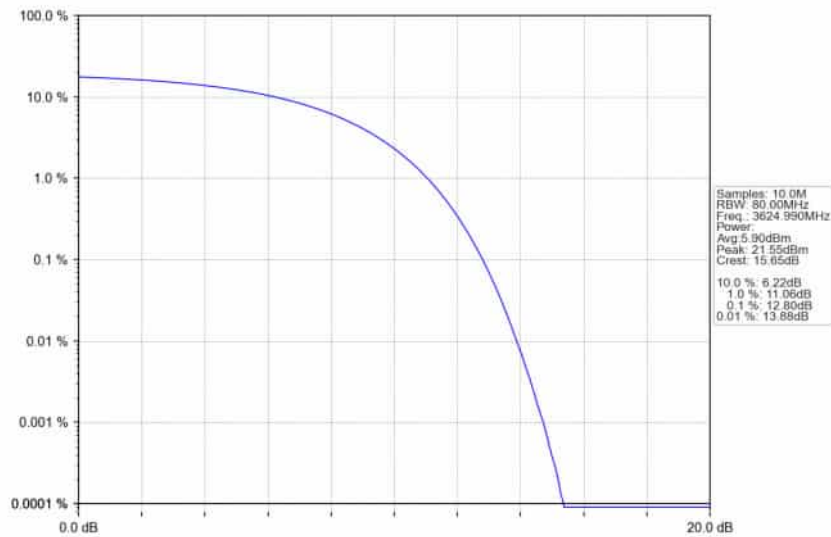
n78d_30kHz_SISO_NTNV_80MHz_CP-OFDM_256_QAM_3624.99MHz_Outer_Full_Ant1
