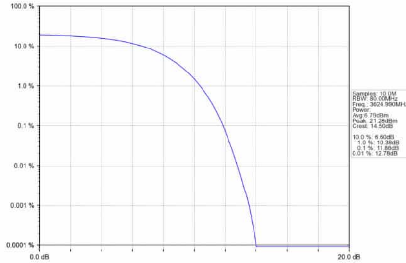
n78d_30kHz_SISO_NTNV_50MHz_DFT-s-OFDM_QPSK_3624.99MHz_Outer_Full_Ant1
