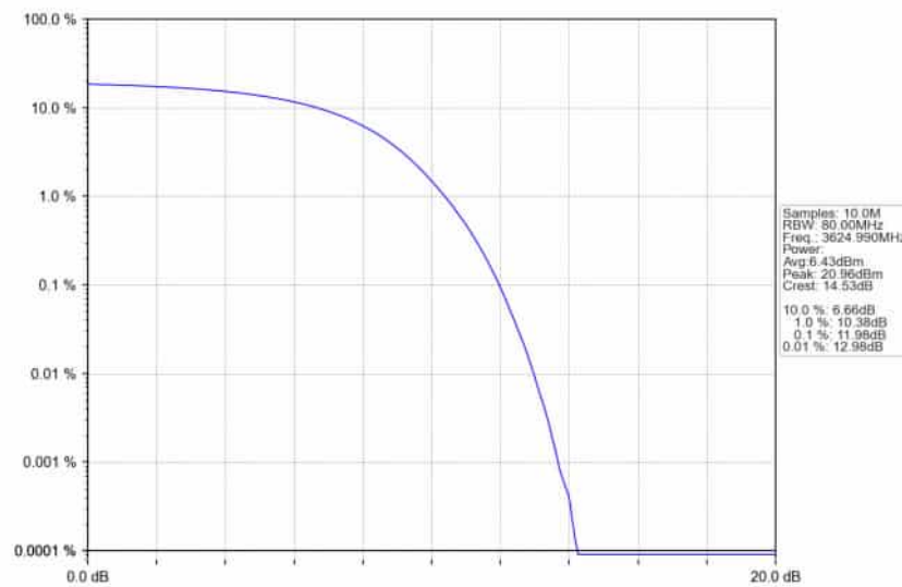
n78d_30kHz_SISO_NTNV_60MHz_DFT-s-OFDM_256_QAM_3624.99MHz_Outer_Full_Ant1
