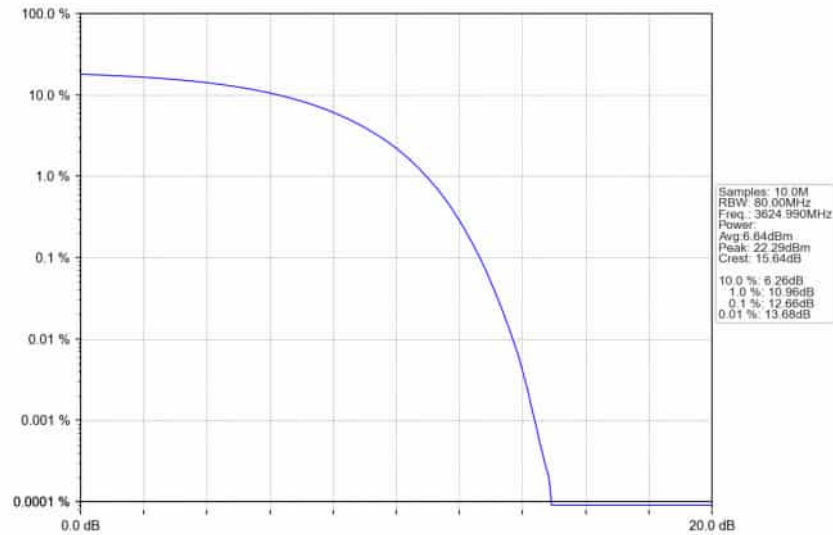
n78d_30kHz_SISO_NTNV_80MHz_DFT-s-OFDM_16_QAM_3624.99MHz_Outer_Full_Ant1
