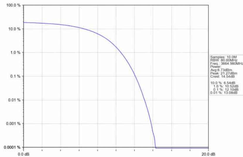
n78d_30kHz_SISO_NTNV_70MHz_DFT-s-OFDM_QPSK_3664.98MHz_Outer_Full_Ant1
