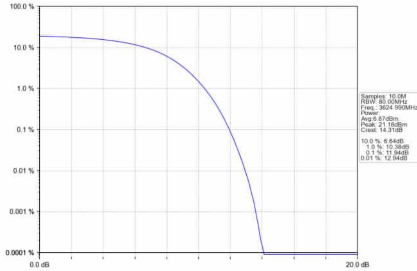
n78d_30kHz_SISO_NTNV_60MHz_DFT-s-OFDM_QPSK_3624.99MHz_Outer_Full_Ant1
