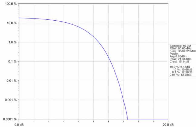
n78d_30kHz_SISO_NTNV_60MHz_CP-OFDM_QPSK_3580.02MHz_Outer_Full_Ant1
