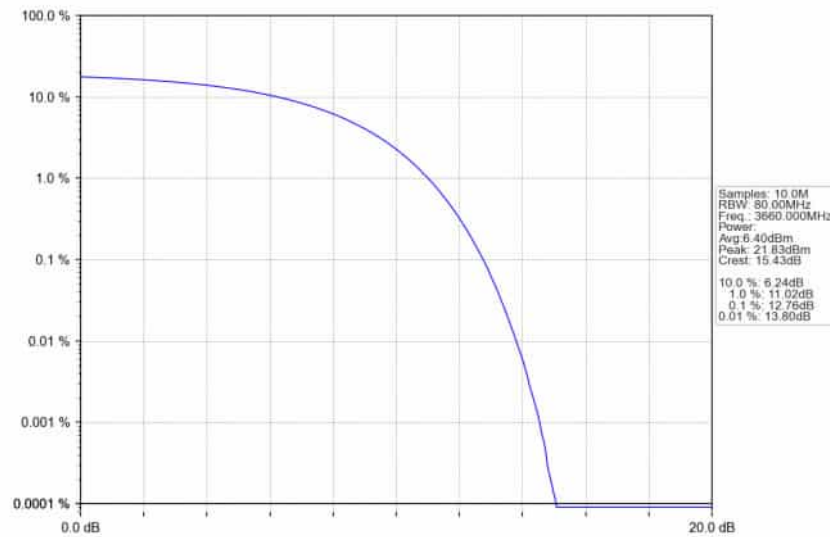
n78d_30kHz_SISO_NTNV_80MHz_CP-OFDM_QPSK_3660MHz_Outer_Full_Ant1
