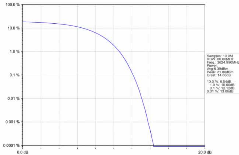
n78d_30kHz_SISO_NTNV_70MHz_DFT-s-OFDM_256_QAM_3624.99MHz_Outer_Full_Ant1
