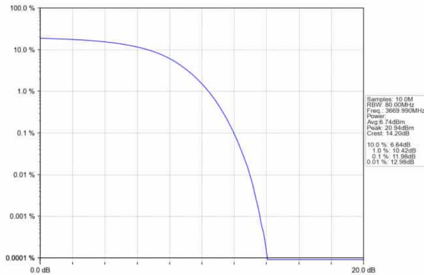
n78d_30kHz_SISO_NTNV_60MHz_DFT-s-OFDM_QPSK_3669.99MHz_Outer_Full_Ant1
