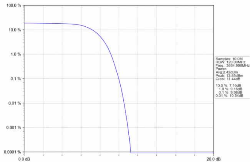
n78d_30kHz_SISO_NTNV_90MHz_DFT-s-OFDM_QPSK_3654.99MHz_Outer_Full_Ant1
