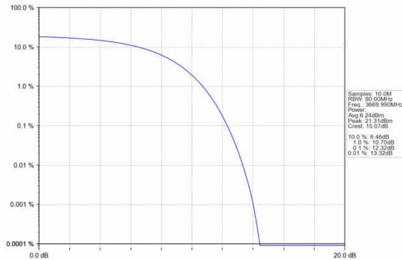
n78d_30kHz_SISO_NTNV_60MHz_CP-OFDM_QPSK_3669.99MHz_Outer_Full_Ant1
