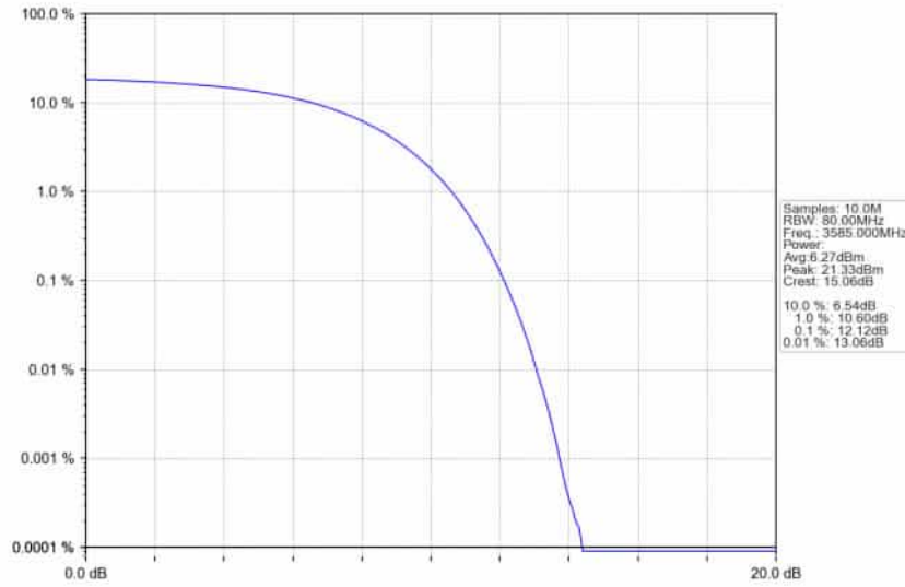
n78d_30kHz_SISO_NTNV_70MHz_DFT-s-OFDM_256_QAM_3585MHz_Outer_Full_Ant1
