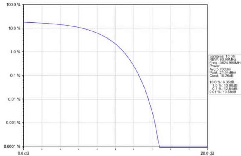
n78d_30kHz_SISO_NTNV_70MHz_CP-OFDM 256 QAM_3624.99MHz_Outer_Full_Ant1
