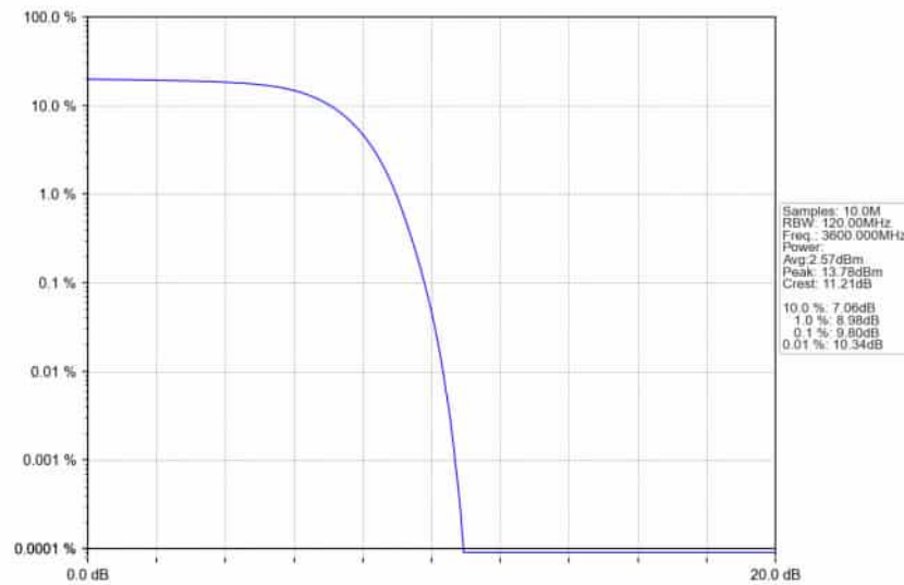
n78d_30kHz_SISO_NTNV_100MHz_DFT-s-OFDM QPSK_3600MHz_Outer_Full_Ant1
