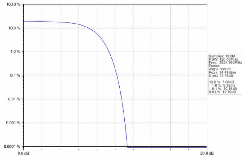
n78d_30kHz_SISO_NTNV_90MHz_CP-OFDM_QPSK_3624.99MHz_Outer_Full_Ant1
