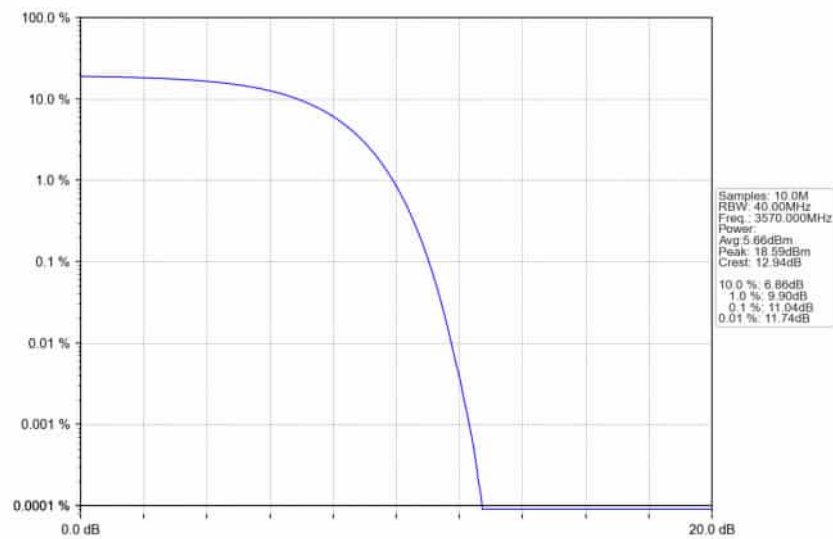
n78d_30kHz_SISO_NTNV_40MHz_CP-OFDM_QPSK_3570MHz_Outer_Full_Ant1
