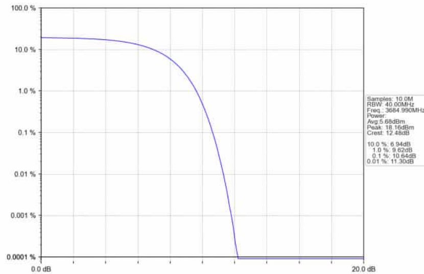
n78d_30kHz_SISO_NTNV_30MHz_CP-OFDM_QPSK_3684.99MHz_Outer_Full_Ant1
