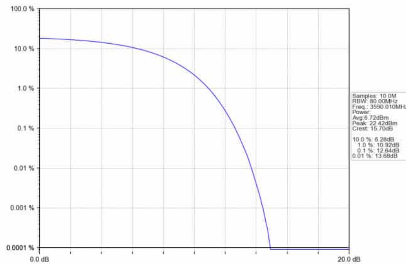
n78d_30kHz_SISO_NTNV_80MHz_DFT-s-OFDM QPSK_3590.01MHz_Outer_Full_Ant1
