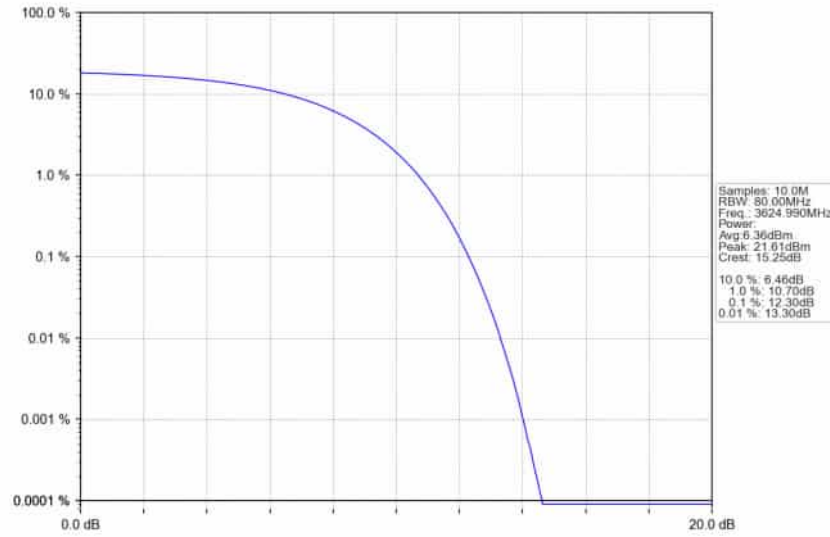
n78d_30kHz_SISO_NTNV_60MHz_CP-OFDM_QPSK_3624.99MHz_Outer_Full_Ant1
