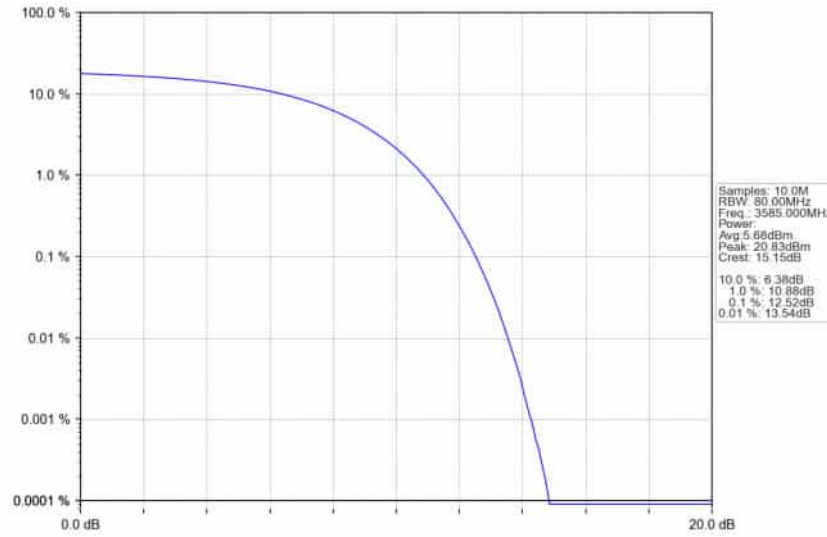
n78d_30kHz_SISO_NTNV_70MHz_CP-OFDM 256 QAM_3585MHz_Outer_Full_Ant1
