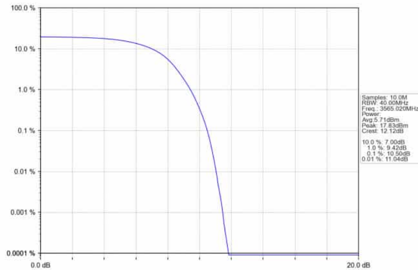
n78d_30kHz_SISO_NTNV_30MHz_DFT-s-OFDM_64_QAM_3565.02MHz_Outer_Full_Ant1
