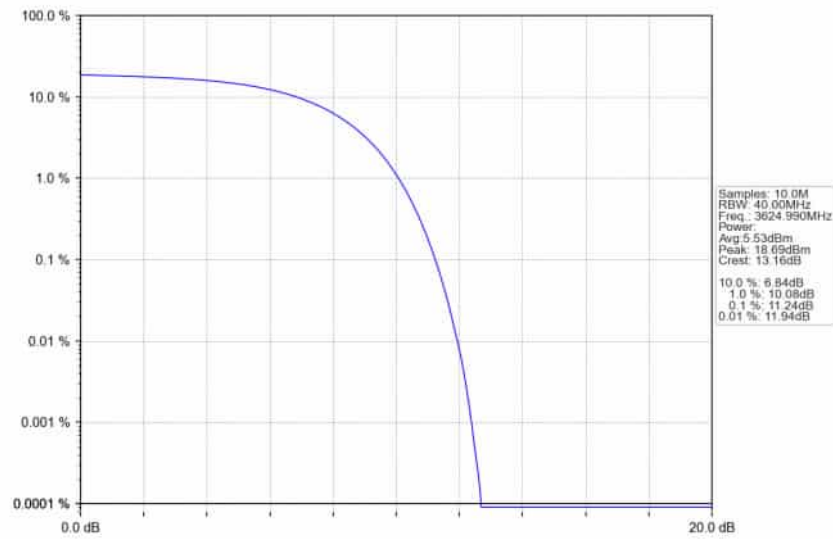
n78d_30kHz_SISO_NTNV_40MHz_CP-OFDM_256_QAM_3624.99MHz_Outer_Full_Ant1
