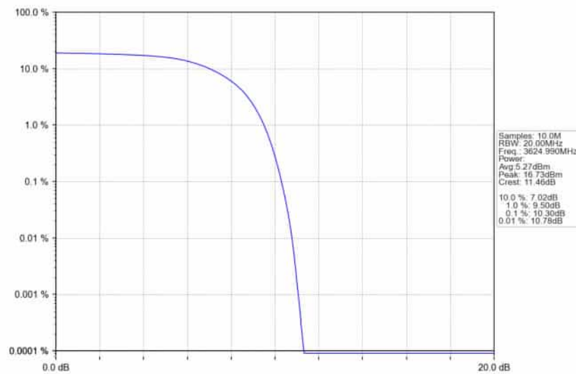
n78d_30kHz_SISO_NTNV_20MHz_DFT-s-OFDM_256_QAM_3624.99MHz_Outer_Full_Ant1
