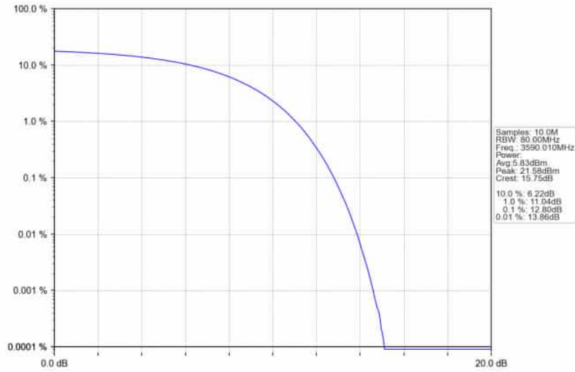
n78d_30kHz_SISO_NTNV_80MHz_CP-OFDM_256_QAM_3590.01MHz_Outer_Full_Ant1
