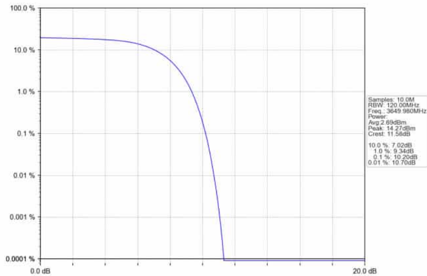
n78d_30kHz_SISO_NTNV_100MHz_CP-OFDM 64 QAM_3649.98MHz_Outer_Full_Ant1
