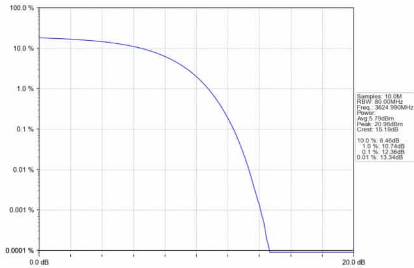
n78d_30kHz_SISO_NTNV_60MHz_CP-OFDM_256_QAM_3624.99MHz_Outer_Full_Ant1
