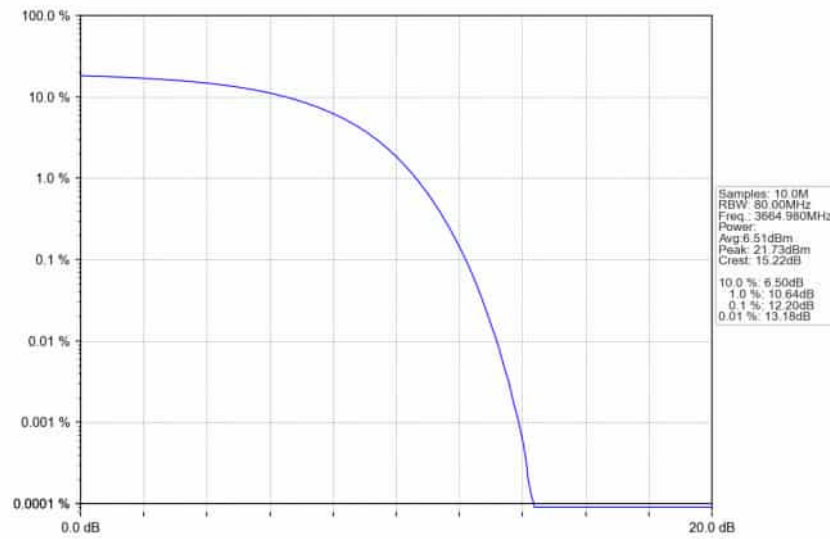
n78d_30kHz_SISO_NTNV_70MHz_DFT-s-OFDM_64_QAM_3664.98MHz_Outer_Full_Ant1
