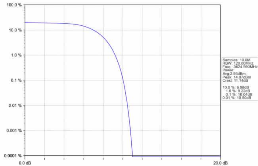
n78d_30kHz_SISO_NTNV_90MHz_DFT-s-OFDM_256_QAM_3624.99MHz_Outer_Full_Ant1
