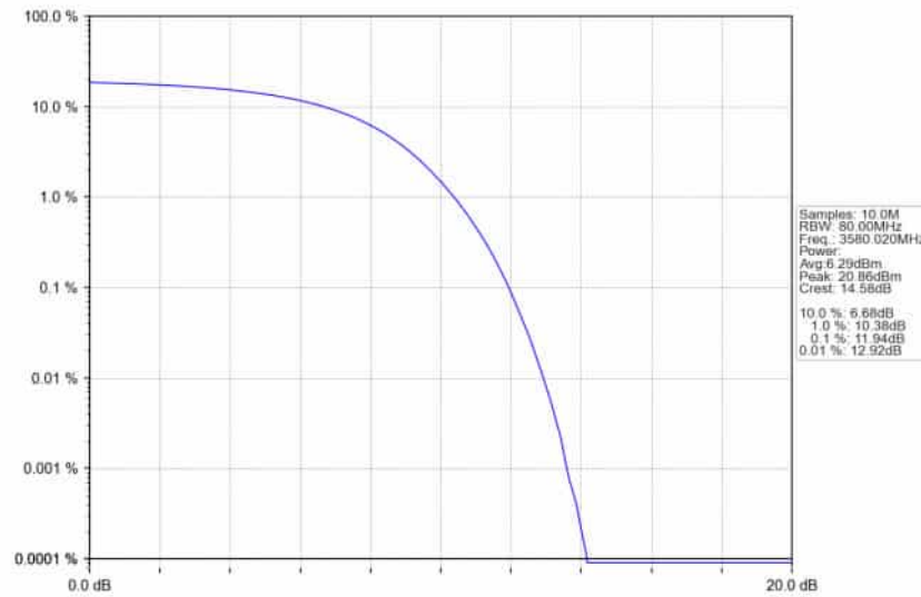
n78d_30kHz_SISO_NTNV_60MHz_DFT-s-OFDM_256_QAM_3580.02MHz_Outer_Full_Ant1
