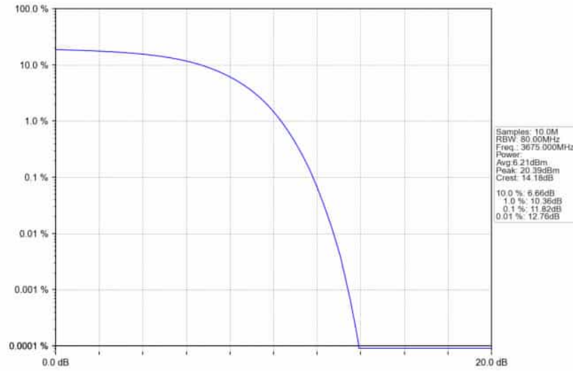
n78d_30kHz_SISO_NTNV_50MHz_DFT-s-OFDM_256_QAM_3675MHz_Outer_Full_Ant1
