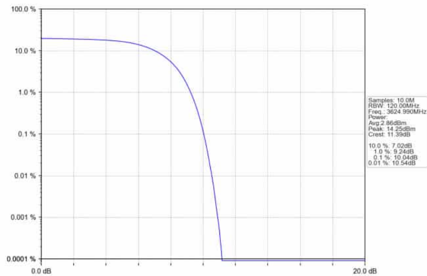
n78d_30kHz_SISO_NTNV_100MHz_DFT-s-OFDM_256_QAM_3624.99MHz_Outer_Full_Ant1
