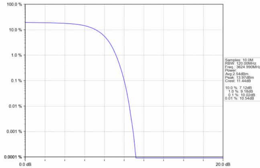
n78d_30kHz_SISO_NTNV_100MHz_DFT-s-OFDM_16_QAM_3624.99MHz_Outer_Full_Ant1
