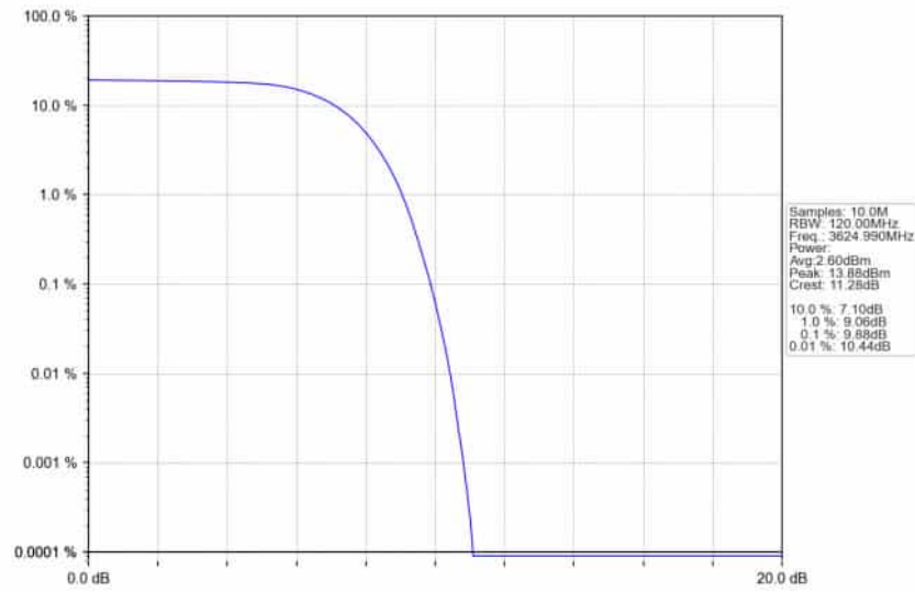
n78d_30kHz_SISO_NTNV_90MHz_DFT-s-OFDM_QPSK_3624.99MHz_Outer_Full_Ant1
