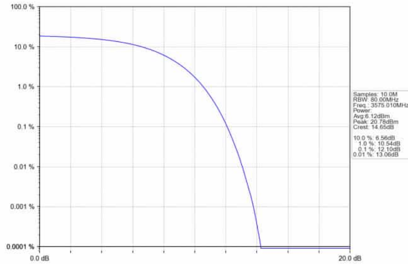
n78d_30kHz_SISO_NTNV_50MHz_CP-OFDM_QPSK_3575.01MHz_Outer_Full_Ant1
