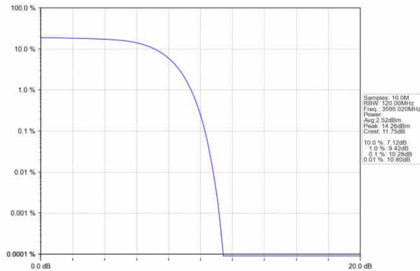
n78d_30kHz_SISO_NTNV_90MHz_CP-OFDM QPSK_3595.02MHz_Outer_Full_Ant1
