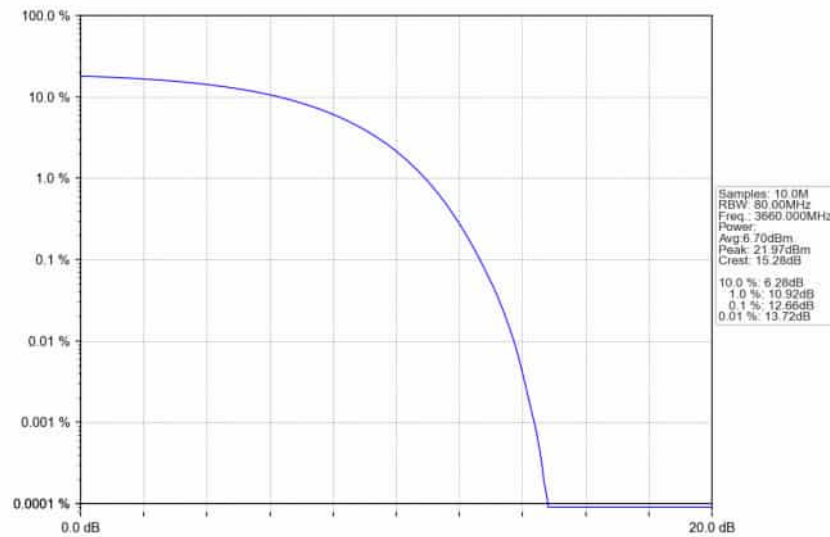
n78d_30kHz_SISO_NTNV_80MHz_DFT-s-OFDM_QPSK_3660MHz_Outer_Full_Ant1
