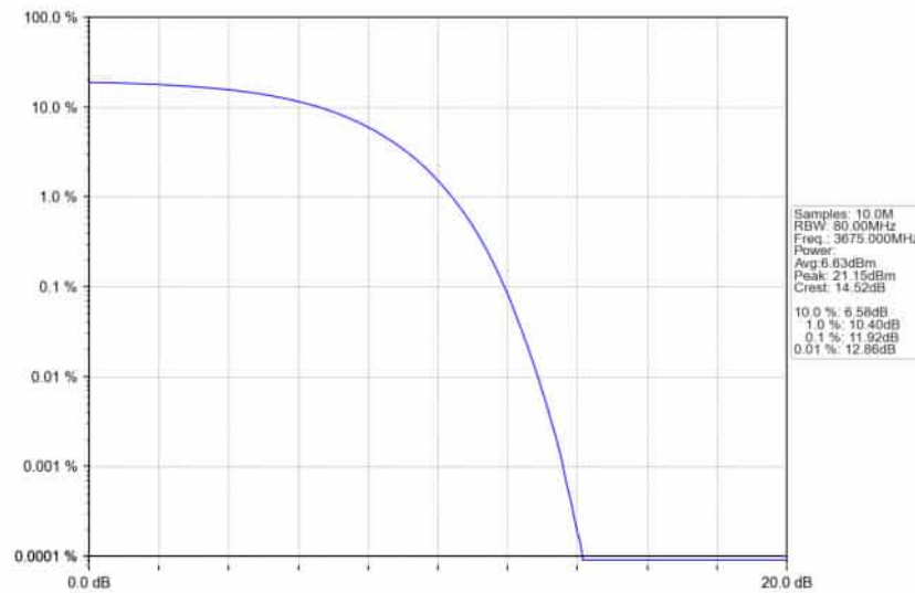
n78d_30kHz_SISO_NTNV_50MHz_DFT-s-OFDM_QPSK_3675MHz_Outer_Full_Ant1
