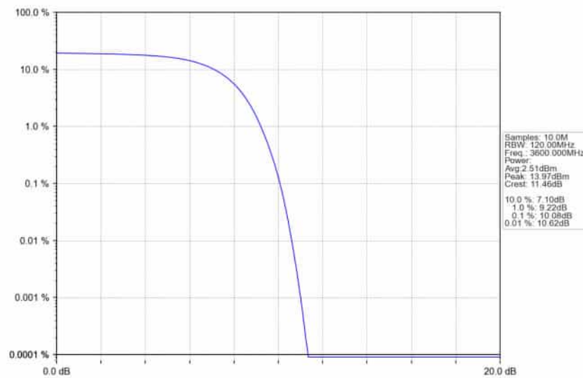
n78d_30kHz_SISO_NTNV_100MHz_DFT-s-OFDM 64 QAM_3600MHz_Outer_Full_Ant1
