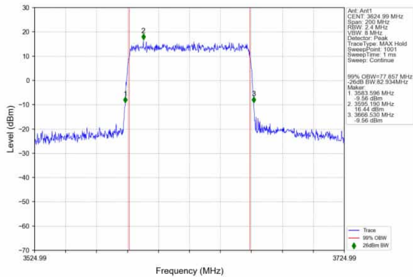
n78d_30kHz_SISO_NTNV_80MHz_DFT-s-OFDM_16_QAM_3624.99MHz_Outer_Full_Ant1
