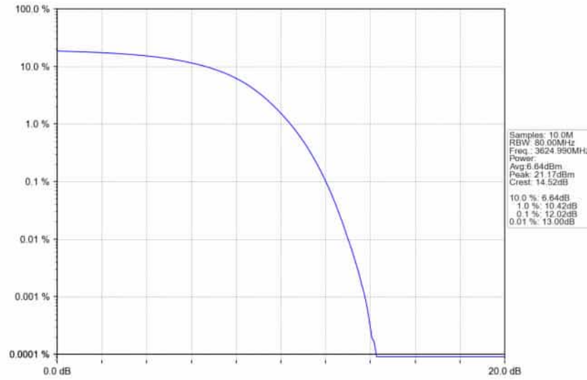
n78d_30kHz_SISO_NTNV_60MHz_DFT-s-OFDM_64_QAM_3624.99MHz_Outer_Full_Ant1
