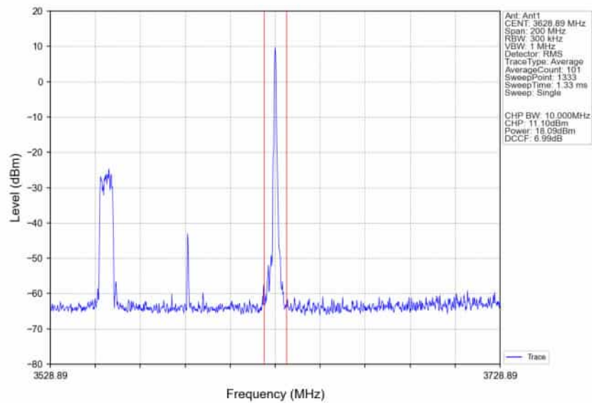
n78d_30kHz_SISO_NTNV_80MHz_CP-OFDM_16_QAM_3590.01MHz_Edge_1RB_Right_Ant1
