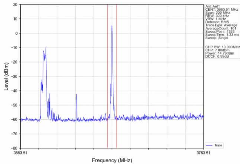
n78d_30kHz_SISO_NTNV_80MHz_CP-OFDM_256_QAM_3624.99MHz_Inner_1RB_Right_Ant1
