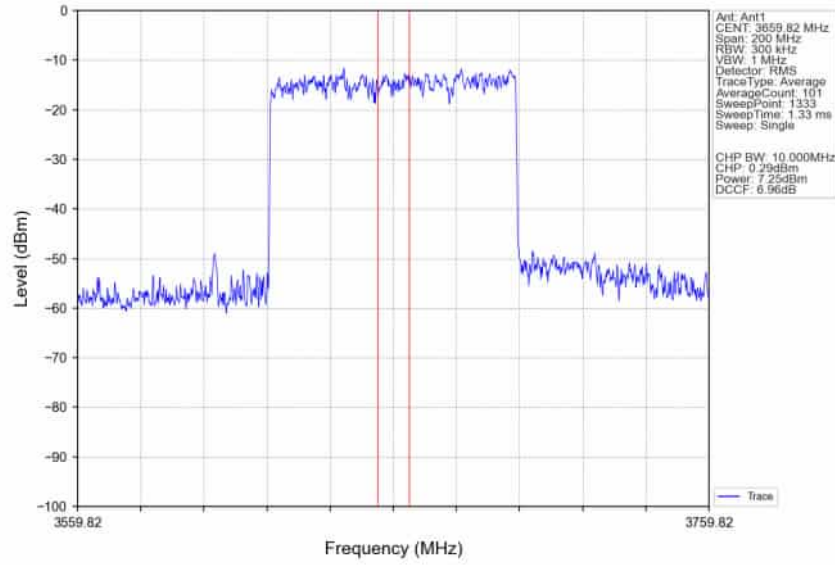
n78d_30kHz_SISO_NTNV_80MHz_DFT-s-OFDM_256_QAM_3660MHz_Inner_Full_Ant1
