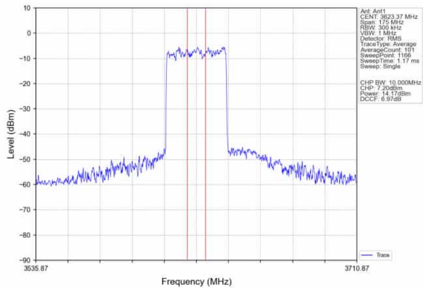
n78d_30kHz_SISO_NTNV_70MHz_DFT-s-OFDM_64_QAM_3624.99MHz_Inner_Full_Ant1
