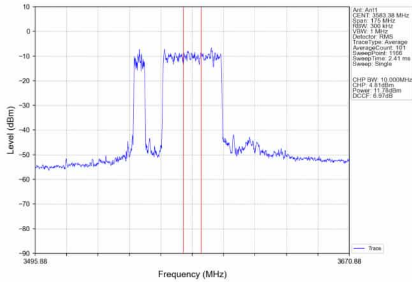
n78d_30kHz_SISO_NTNV_70MHz_DFT-s-OFDM PI/2 BPSK_3585MHz_Inner_Full_Ant1
