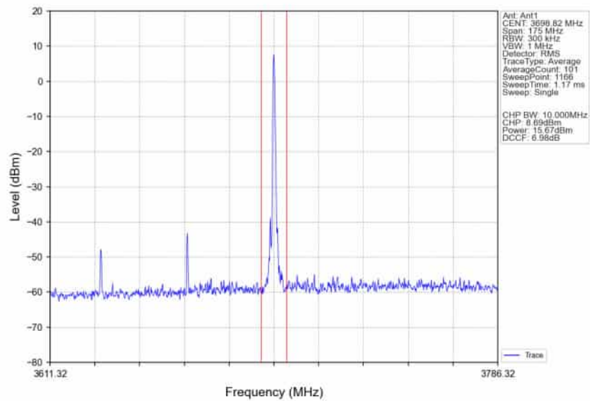
n78d_30kHz_SISO_NTNV_70MHz_DFT-s-OFDM_256_QAM_3664.98MHz_Edge_1RB_Right_Ant1
