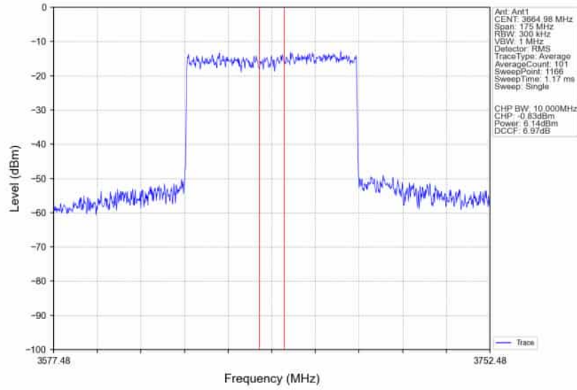
n78d_30kHz_SISO_NTNV_70MHz_CP-OFDM_256_QAM_3664.98MHz_Inner_Full_Ant1
