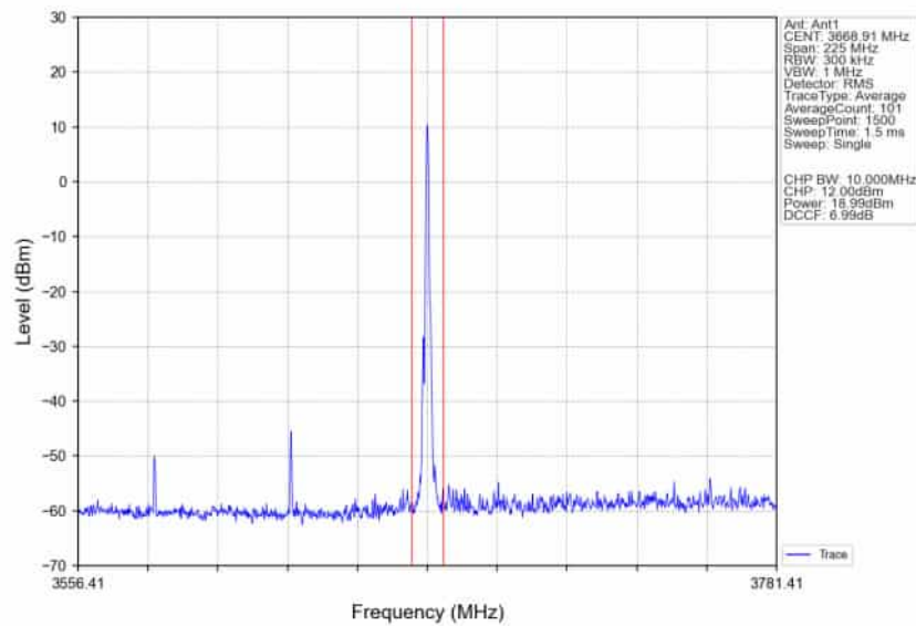
n78d_30kHz_SISO_NTNV_90MHz_DFT-s-OFDM QPSK_3624.99MHz_Edge_1RB_Right_Ant1
