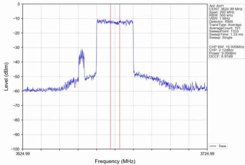
n78d_30kHz_SISO_NTNV_80MHz_CP-OFDM_256_QAM_3624.99MHz_Inner_Full_Ant1
