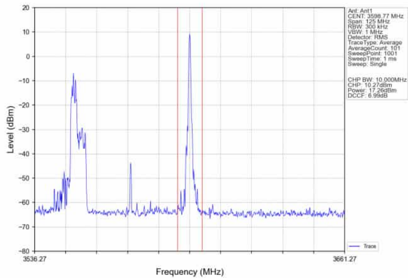
n78d_30kHz_SISO_NTNV_50MHz_CP-OFDM_64_QAM_3575.01MHz_Edge_1RB_Right_Ant1
