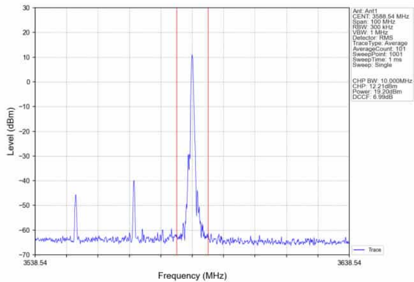
n78d_30kHz_SISO_NTNV_40MHz_CP-OFDM 64 QAM_3570MHz_Inner_1RB_Right_Ant1
