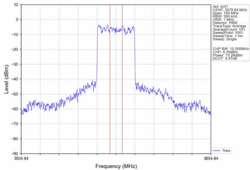
n78d_30kHz_SISO_NTNV_60MHz_DFT-s-OFDM_QPSK_3580.02MHz_Inner_Full_Ant1
