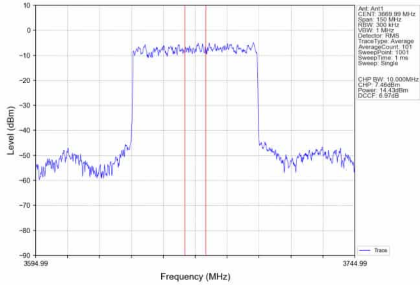
n78d_30kHz_SISO_NTNV_60MHz_DFT-s-OFDM PI/2 BPSK_3669.99MHz_Inner_Full_Ant1
