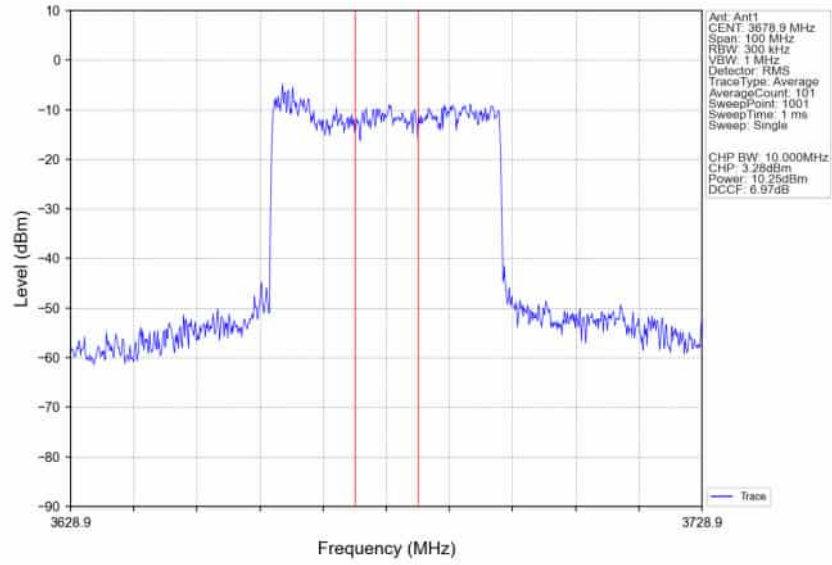
n78d_30kHz_SISO_NTNV_40MHz_DFT-s-OFDM_16_QAM_3679.98MHz_Inner_Full_Ant1
