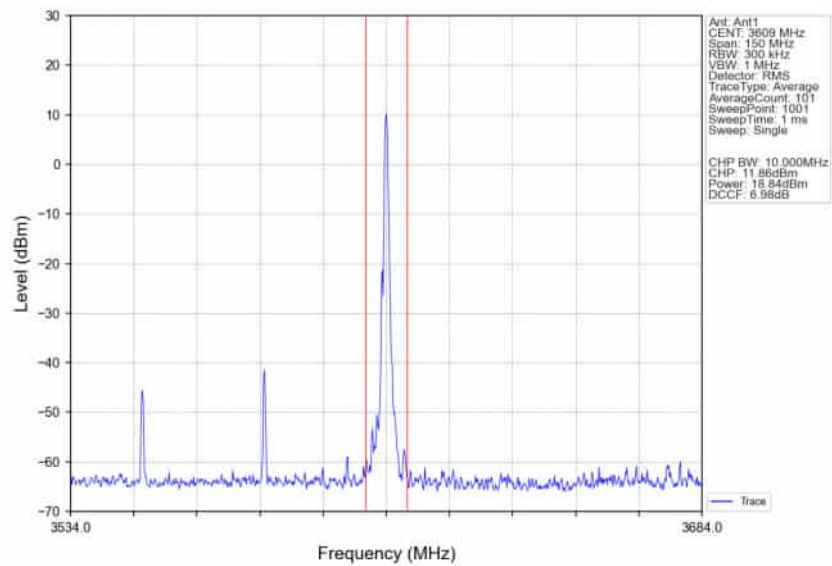
n78d_30kHz_SISO_NTNV_60MHz_CP-OFDM_QPSK_3580.02MHz_Edge_1RB_Right_Ant1
