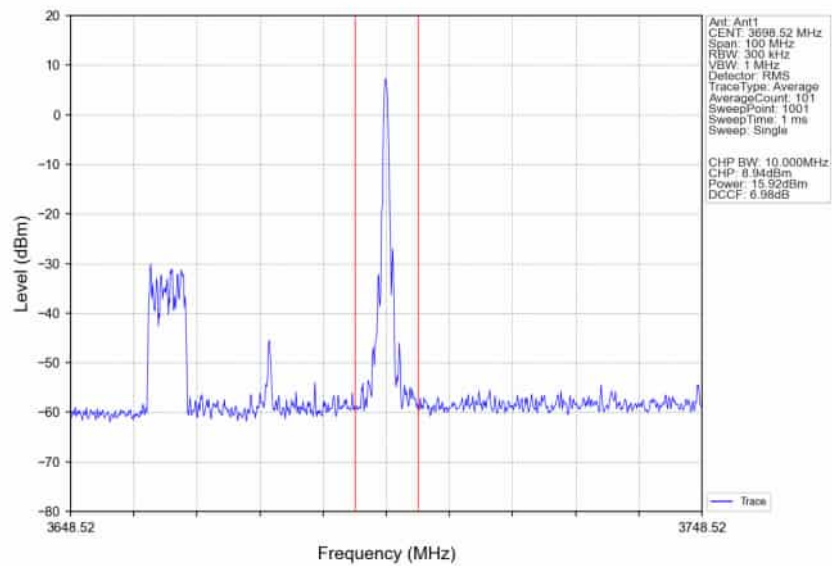
n78d_30kHz_SISO_NTNV_40MHz_CP-OFDM_QPSK_3679.98MHz_Inner_1RB_Right_Ant1
