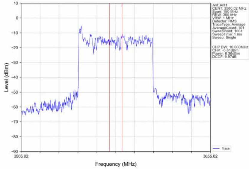
n78d_30kHz_SISO_NTNV_60MHz_DFT-s-OFDM_16_QAM_3580.02MHz_Inner_Full_Ant1
