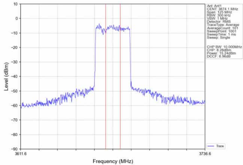
n78d_30kHz_SISO_NTNV_50MHz_DFT-s-OFDM 64 QAM 3675MHz_Inner_Full_Ant1
