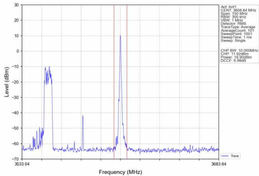
n78d_30kHz_SISO_NTNV_60MHz_CP-OFDM 64 QAM_3580.02MHz_Inner_1RB_Right_Ant1
