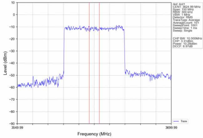
n78d_30kHz_SISO_NTNV_60MHz_DFT-s-OFDM_64_QAM_3624.99MHz_Inner_Full_Ant1
