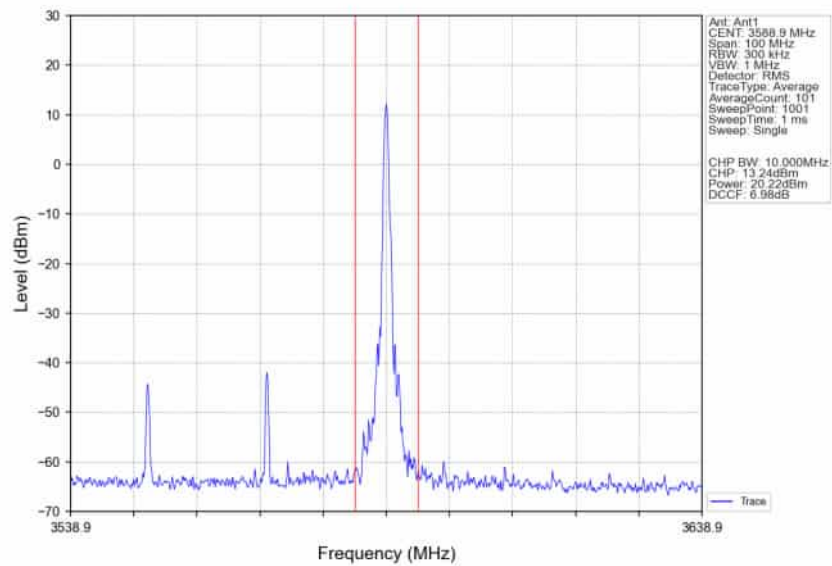
n78d_30kHz_SISO_NTNV_40MHz_DFT-s-OFDM_QPSK_3570MHz_Edge_1RB_Right_Ant1
