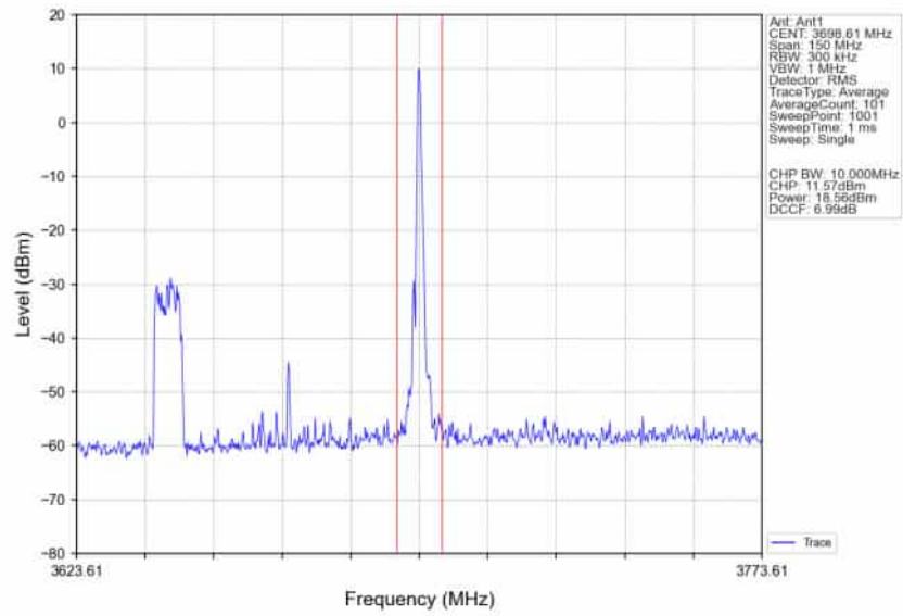
n78d_30kHz_SISO_NTNV_60MHz_CP-OFDM_QPSK_3669.99MHz_Inner_1RB_Right_Ant1
