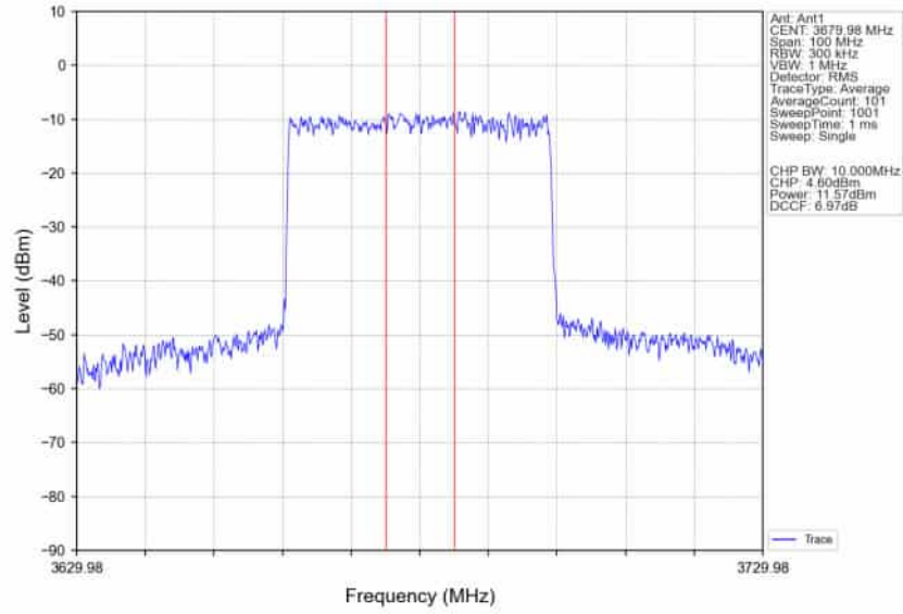
n78d_30kHz_SISO_NTNV_40MHz_CP-OFDM 64 QAM 3679.98MHz_Inner_Full_Ant1
