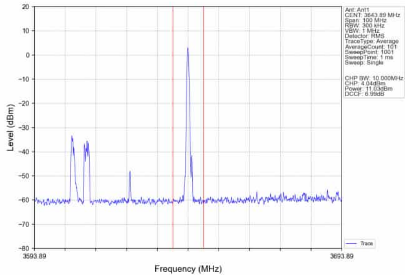
n78d_30kHz_SISO_NTNV_40MHz_DFT-s-OFDM_256_QAM_3624.99MHz_Edge_1RB_Right_Ant1
