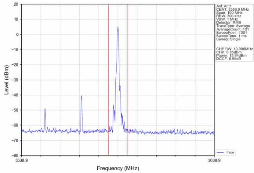
n78d_30kHz_SISO_NTNV_40MHz_CP-OFDM_256_QAM_3570MHz_Edge_1RB_Right_Ant1
