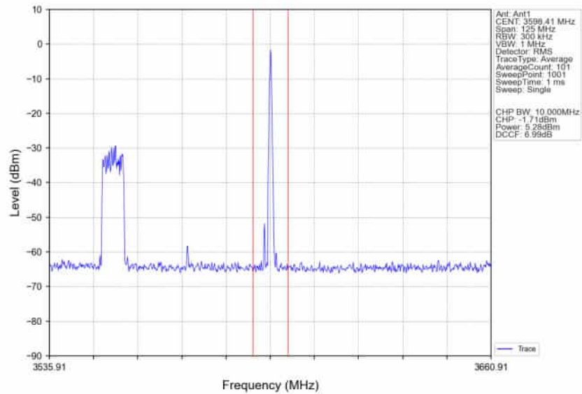
n78d_30kHz_SISO_NTNV_50MHz_DFT-s-OFDM_256_QAM_3575.01MHz_Inner_1RB_Right_Ant1
