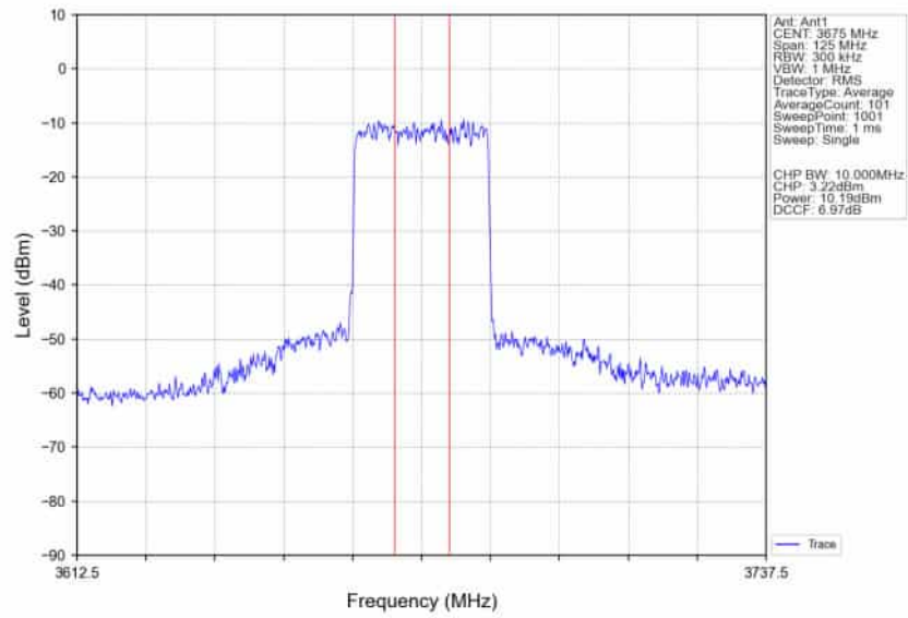
n78d_30kHz_SISO_NTNV_50MHz_CP-OFDM_256_QAM_3675MHz_Inner_Full_Ant1
