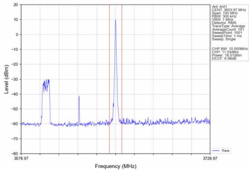
n78d_30kHz_SISO_NTNV_60MHz_CP-OFDM_16_QAM_3624.99MHz_Edge_1RB_Right_Ant1
