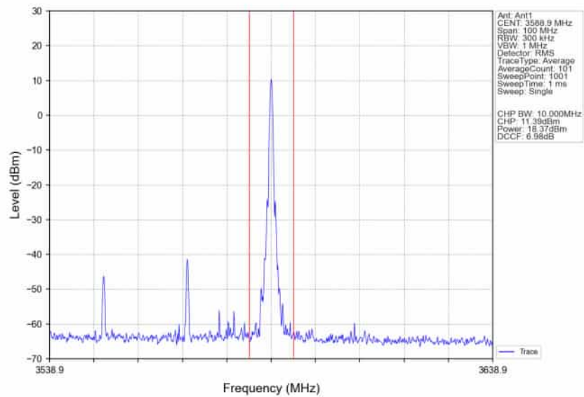
n78d_30kHz_SISO_NTNV_40MHz_CP-OFDM_64_QAM_3570MHz_Edge_1RB_Right_Ant1
