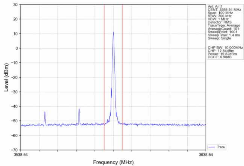
n78d_30kHz_SISO_NTNV_40MHz_DFT-s-OFDM_QPSK_3570MHz_Inner_1RB_Right_Ant1
