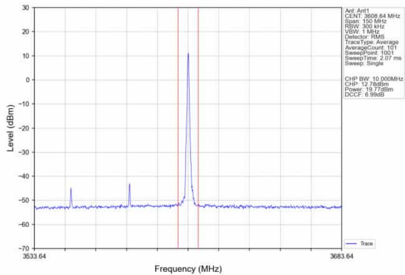
n78d_30kHz_SISO_NTNV_60MHz_DFT-s-OFDM_16_QAM_3580.02MHz_Inner_1RB_Right_Ant1
