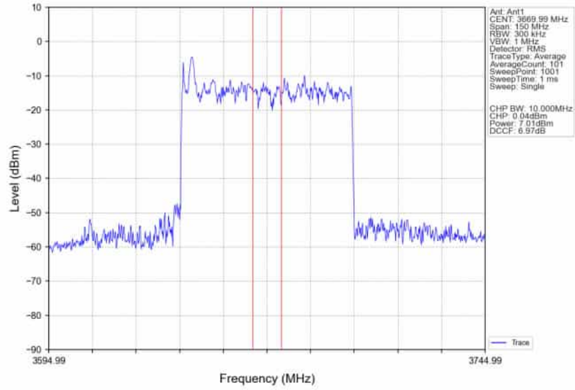
n78d_30kHz_SISO_NTNV_60MHz_DFT-s-OFDM_64_QAM_3669.99MHz_Inner_Full_Ant1
