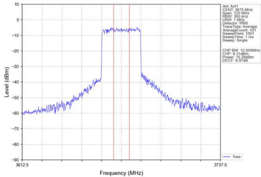
n78d_30kHz_SISO_NTNV_50MHz_CP-OFDM 16 QAM 3675MHz_Inner_Full_Ant1
