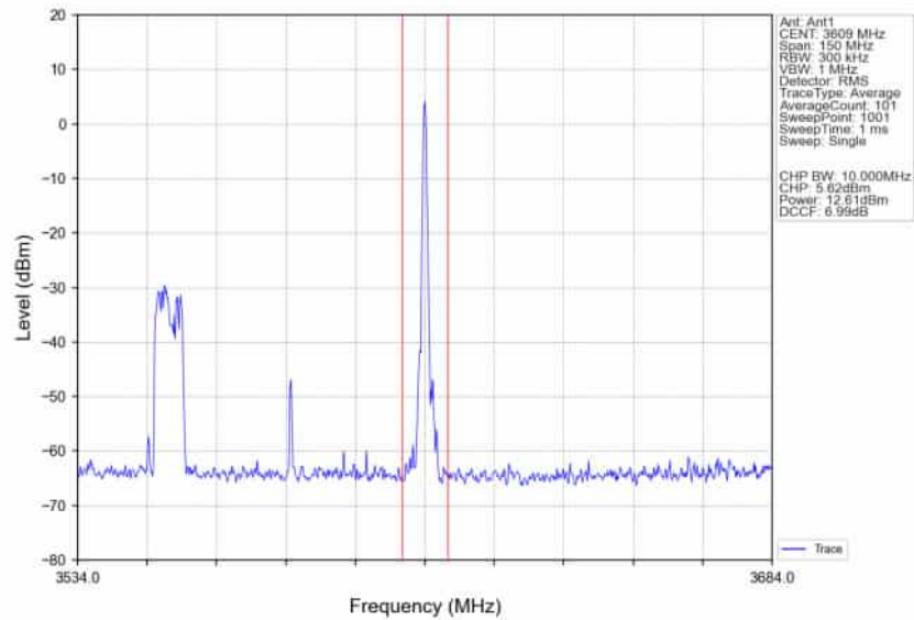
n78d_30kHz_SISO_NTNV_60MHz_CP-OFDM_64_QAM_3580.02MHz_Edge_1RB_Right_Ant1
