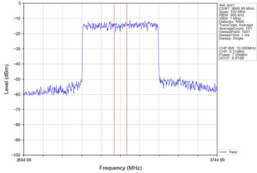
n78d_30kHz_SISO_NTNV_60MHz_CP-OFDM_QPSK_3669.99MHz_Inner_Full_Ant1
