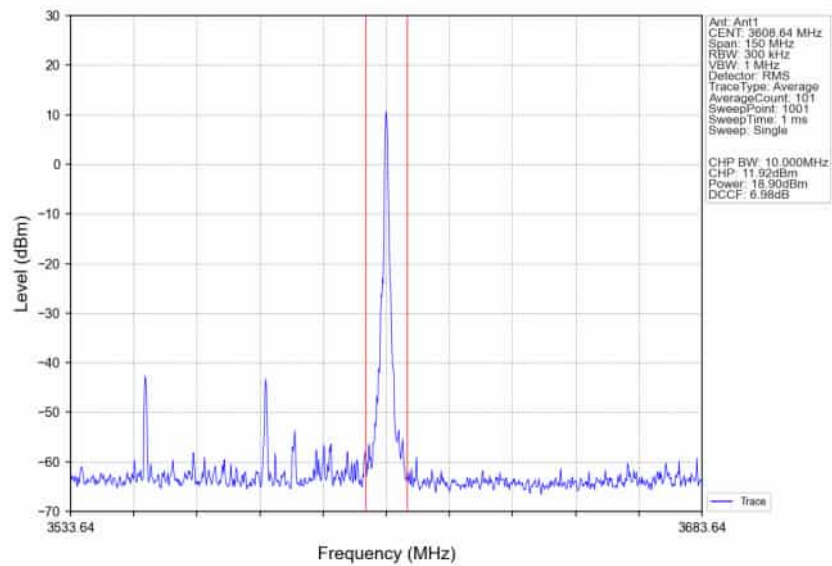
n78d_30kHz_SISO_NTNV_60MHz_CP-OFDM_QPSK_3580.02MHz_Inner_1RB_Right_Ant1
