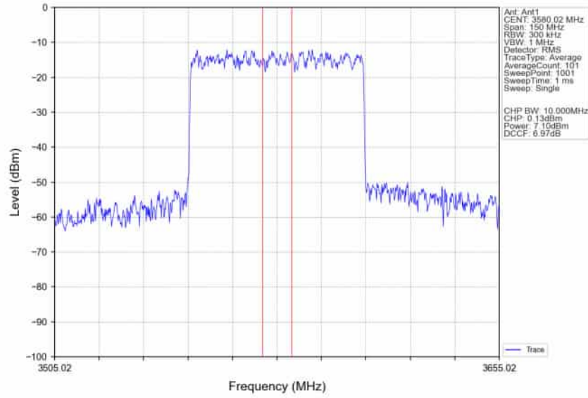
n78d_30kHz_SISO_NTNV_60MHz_DFT-s-OFDM_256_QAM_3580.02MHz_Inner_Full_Ant1
