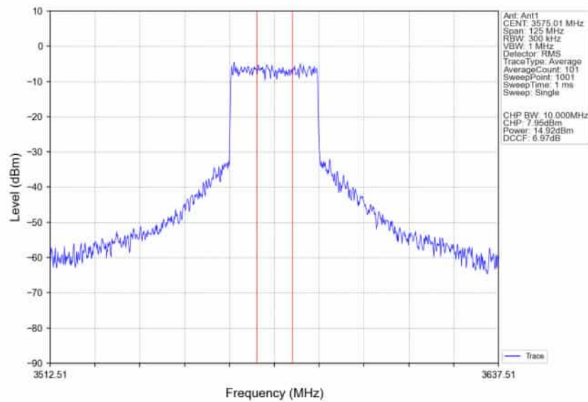
n78d_30kHz_SISO_NTNV_50MHz_CP-OFDM_QPSK_3575.01MHz_Inner_Full_Ant1
