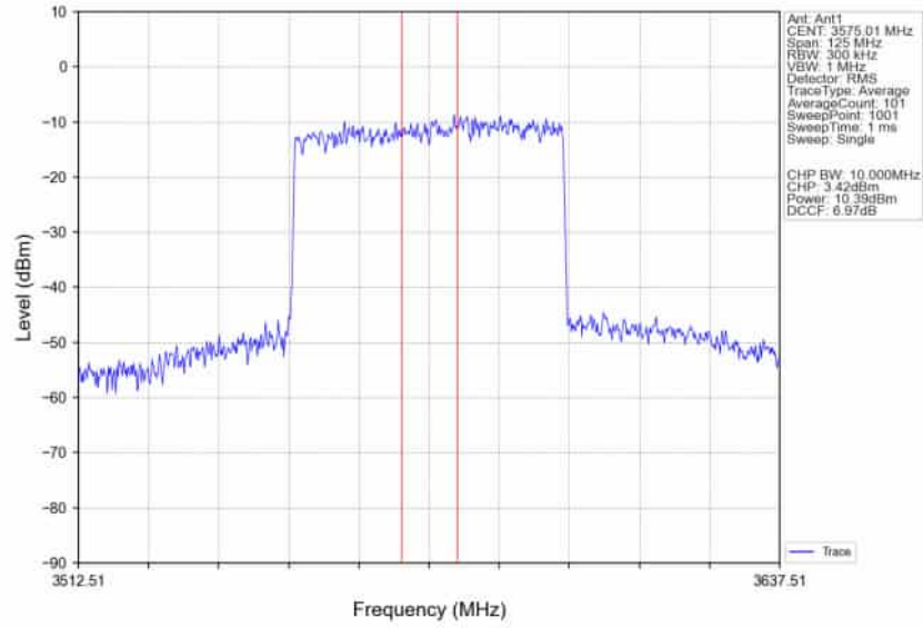
n78d_30kHz_SISO_NTNV_50MHz_CP-OFDM 64 QAM 3575.01MHz_Inner_Full_Ant1
