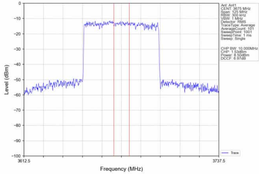
n78d_30kHz_SISO_NTNV_50MHz_CP-OFDM_256_QAM_3675MHz_Inner_Full_Ant1
