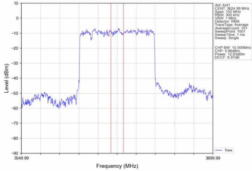
n78d_30kHz_SISO_NTNV_60MHz_DFT-s-OFDM PI/2 BPSK_3624.99MHz_Inner_Full_Ant1
