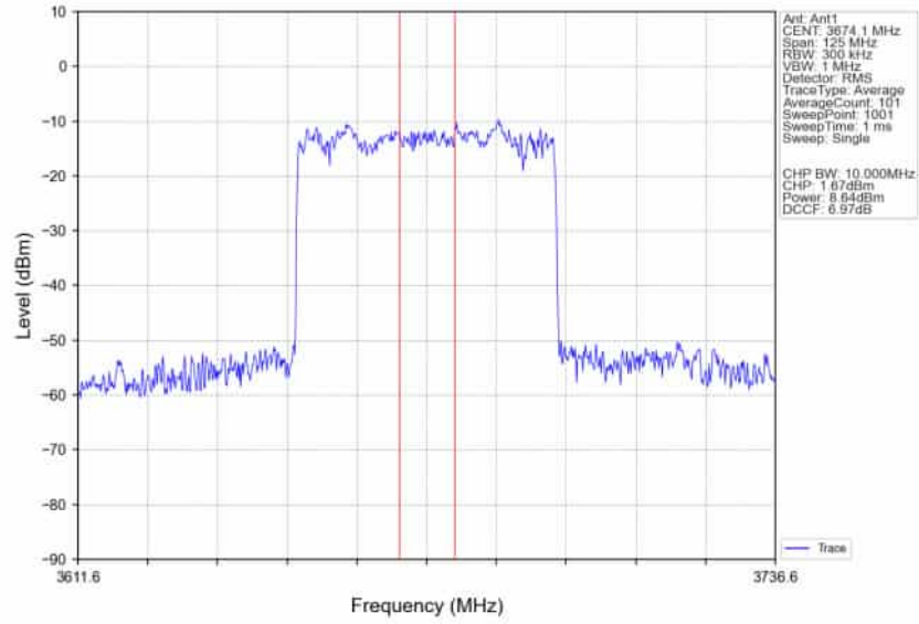
n78d_30kHz_SISO_NTNV_50MHz_DFT-s-OFDM_256_QAM_3675MHz_Inner_Full_Ant1
