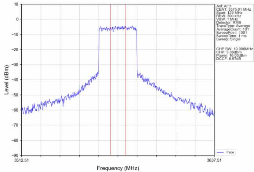
n78d_30kHz_SISO_NTNV_50MHz_CP-OFDM 16 QAM 3575.01MHz_Inner_Full_Ant1
