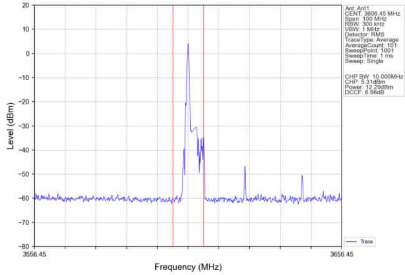
n78d_30kHz_SISO_NTNV_40MHz_DFT-s-OFDM_256_QAM_3624.99MHz_Inner_1RB_Right_Ant1
