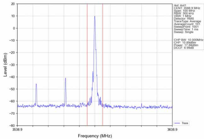
n78d_30kHz_SISO_NTNV_40MHz_CP-OFDM_16_QAM_3570MHz_Edge_1RB_Right_Ant1
