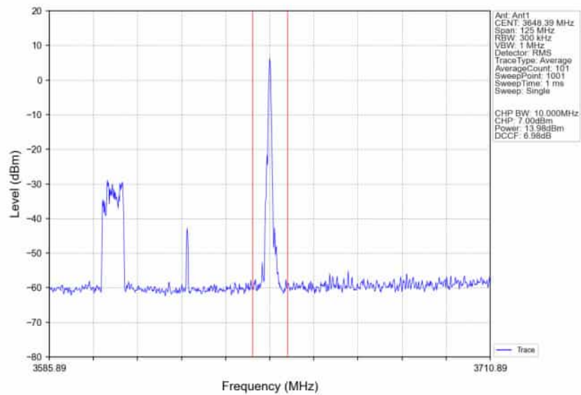
n78d_30kHz_SISO_NTNV_50MHz_CP-OFDM_256_QAM_3624.99MHz_Inner_1RB_Right_Ant1
