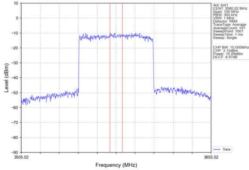
n78d_30kHz_SISO_NTNV_60MHz_CP-OFDM 16 QAM 3580.02MHz_Inner_Full_Ant1
