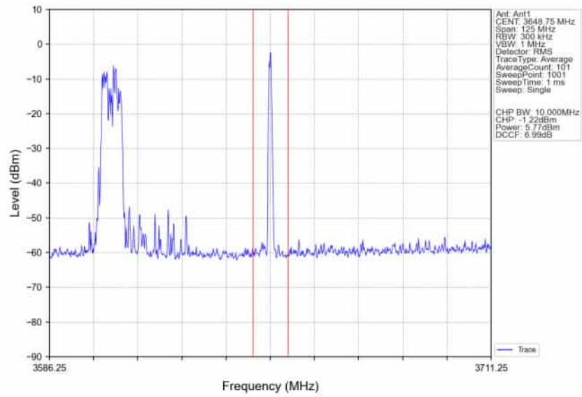
n78d_30kHz_SISO_NTNV_50MHz_DFT-s-OFDM_64_QAM_3624.99MHz_Edge_1RB_Right_Ant1
