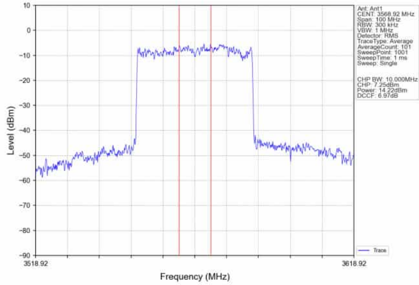
n78d_30kHz_SISO_NTNV_40MHz_DFT-s-OFDM_16_QAM_3570MHz_Inner_Full_Ant1
