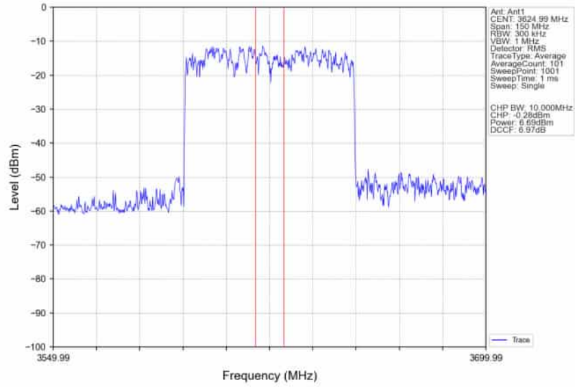
n78d_30kHz_SISO_NTNV_60MHz_DFT-s-OFDM_16_QAM_3624.99MHz_Inner_Full_Ant1
