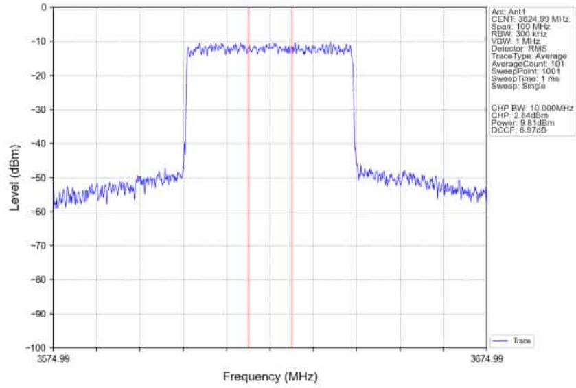
n78d_30kHz_SISO_NTNV_40MHz_CP-OFDM_256_QAM_3624.99MHz_Inner_Full_Ant1
