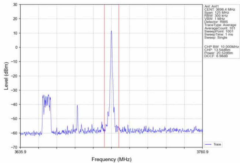
n78d_30kHz_SISO_NTNV_50MHz_CP-OFDM_16_QAM_3675MHz_Inner_1RB_Right_Ant1
