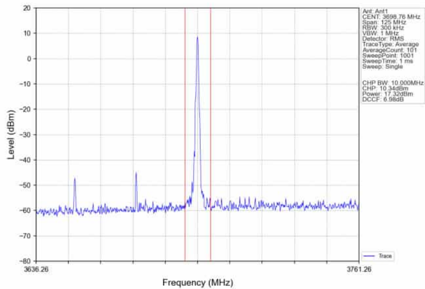
n78d_30kHz_SISO_NTNV_50MHz_DFT-s-OFDM PI/2 BPSK_3675MHz_Edge_1RB_Right_Ant1
