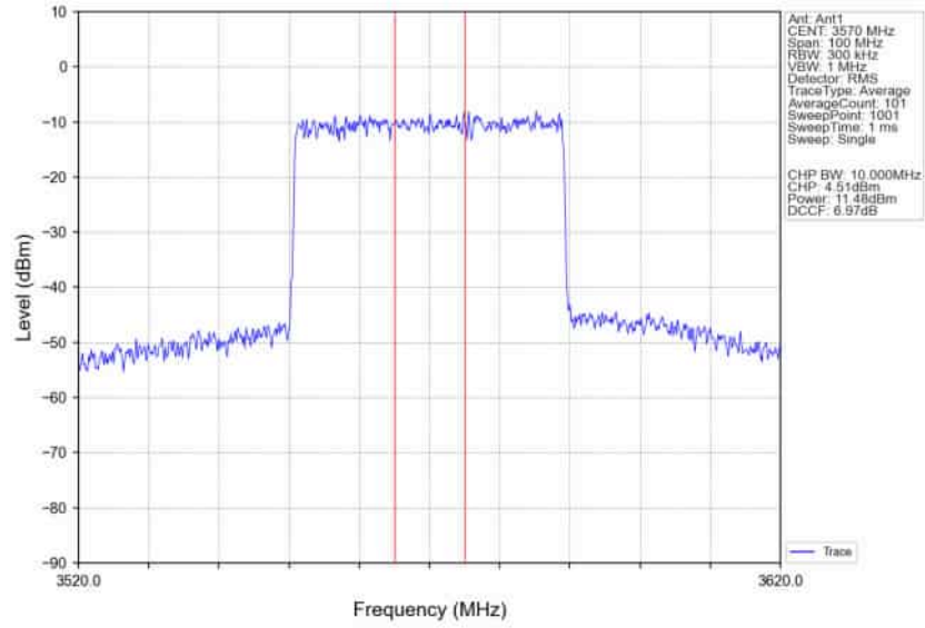
n78d_30kHz_SISO_NTNV_40MHz_CP-OFDM 64 QAM 3570MHz_Inner_Full_Ant1
