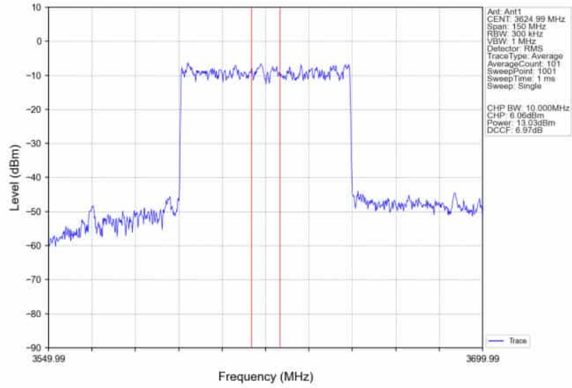
n78d_30kHz_SISO_NTNV_60MHz_DFT-s-OFDM_QPSK_3624.99MHz_Inner_Full_Ant1
