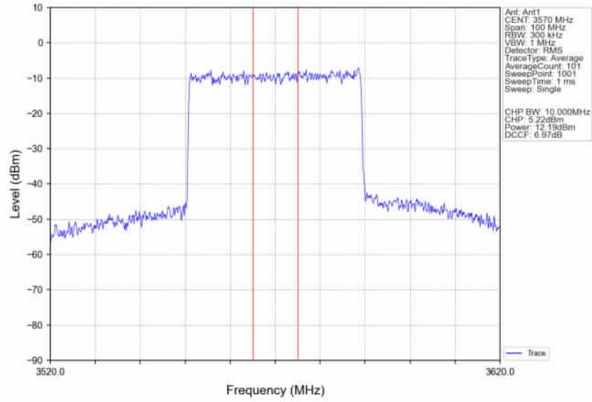
n78d_30kHz_SISO_NTNV_40MHz_CP-OFDM_16_QAM_3570MHz_Inner_Full_Ant1
