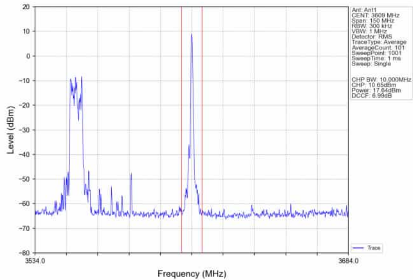
n78d_30kHz_SISO_NTNV_60MHz_DFT-s-OFDM_QPSK_3580.02MHz_Edge_1RB_Right_Ant1
