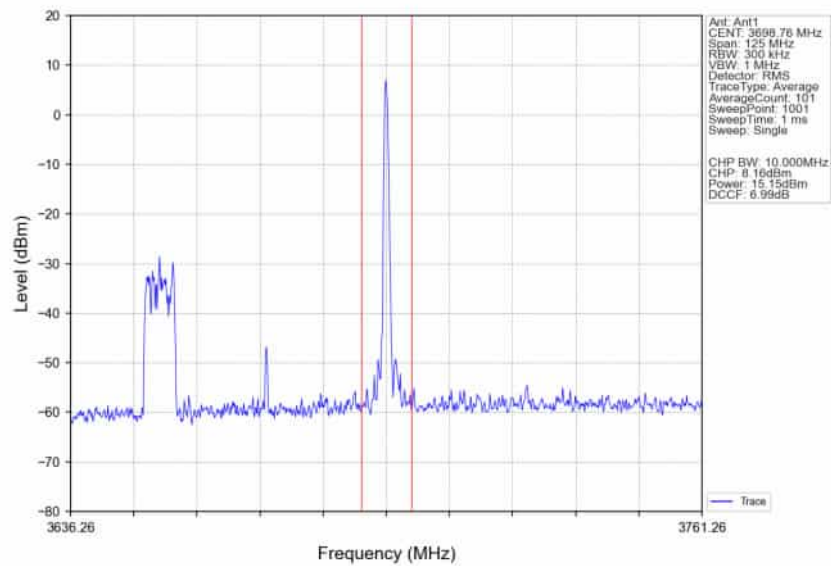
n78d_30kHz_SISO_NTNV_50MHz_DFT-s-OFDM_64_QAM_3675MHz_Edge_1RB_Right_Ant1
