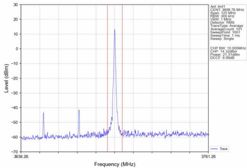
n78d_30kHz_SISO_NTNV_50MHz_DFT-s-OFDM_QPSK_3675MHz_Edge_1RB_Right_Ant1
