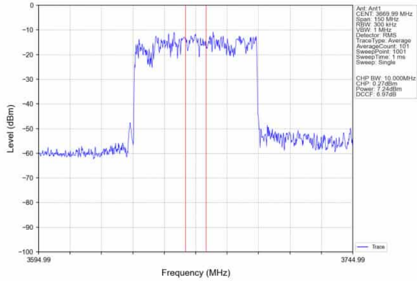
n78d_30kHz_SISO_NTNV_60MHz_DFT-s-OFDM_QPSK_3669.99MHz_Inner_Full_Ant1
