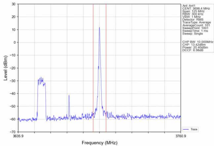
n78d_30kHz_SISO_NTNV_50MHz_DFT-s-OFDM_16_QAM_3675MHz_Inner_1RB_Right_Ant1
