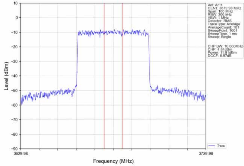
n78d_30kHz_SISO_NTNV_40MHz_CP-OFDM_QPSK_3679.98MHz_Inner_Full_Ant1
