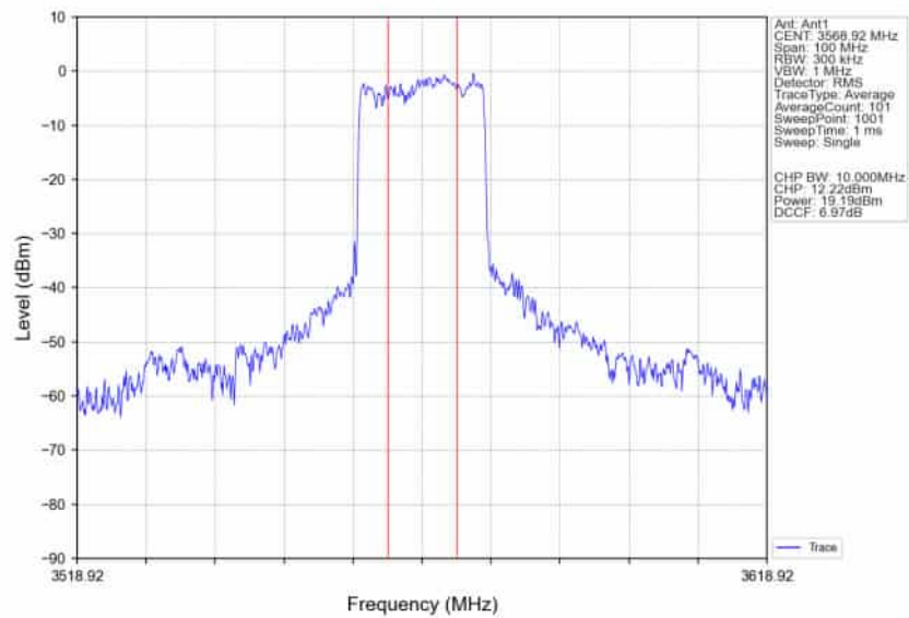
n78d_30kHz_SISO_NTNV_40MHz_DFT-s-OFDM_QPSK_3570MHz_Inner_Full_Ant1
