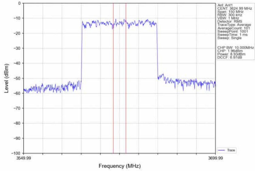
n78d_30kHz_SISO_NTNV_60MHz_DFT-s-OFDM_256_QAM_3624.99MHz_Inner_Full_Ant1
