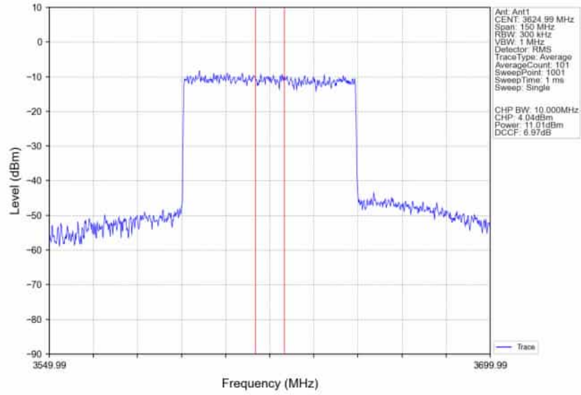
n78d_30kHz_SISO_NTNV_60MHz_CP-OFDM 16 QAM 3624.99MHz_Inner_Full_Ant1
