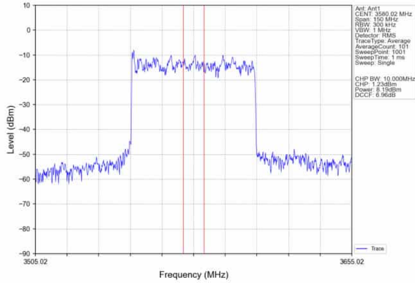
n78d_30kHz_SISO_NTNV_60MHz_DFT-s-OFDM_64_QAM_3580.02MHz_Inner_Full_Ant1
