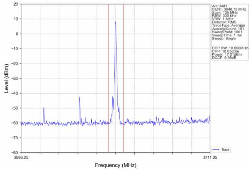
n78d_30kHz_SISO_NTNV_50MHz_CP-OFDM_QPSK_3624.99MHz_Edge_1RB_Right_Ant1
