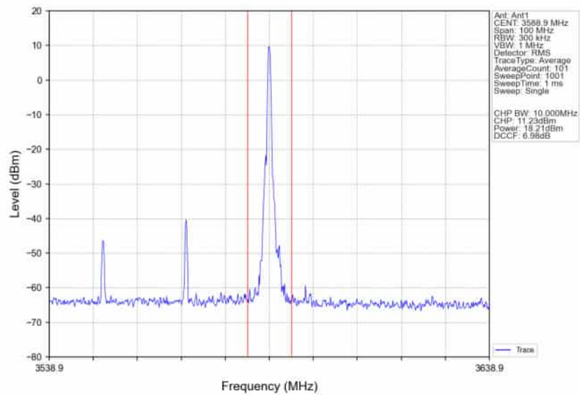
n78d_30kHz_SISO_NTNV_40MHz_DFT-s-OFDM_256_QAM_3570MHz_Edge_1RB_Right_Ant1
