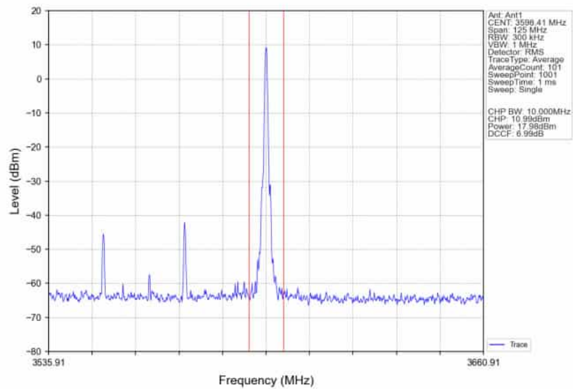
n78d_30kHz_SISO_NTNV_50MHz_CP-OFDM 64 QAM_3575.01MHz_Inner_1RB_Right_Ant1
