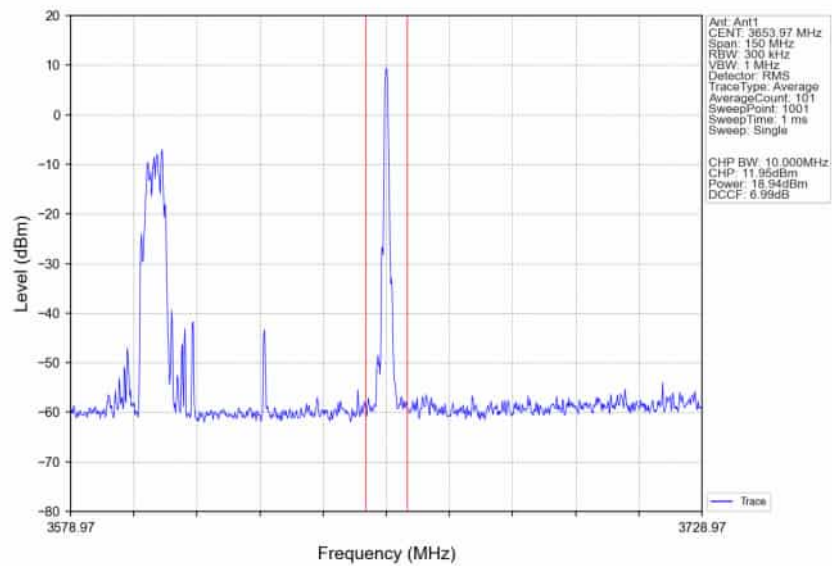
n78d_30kHz_SISO_NTNV_60MHz_DFT-s-OFDM PI/2 BPSK_3624.99MHz_Edge_1RB_Right_Ant1
