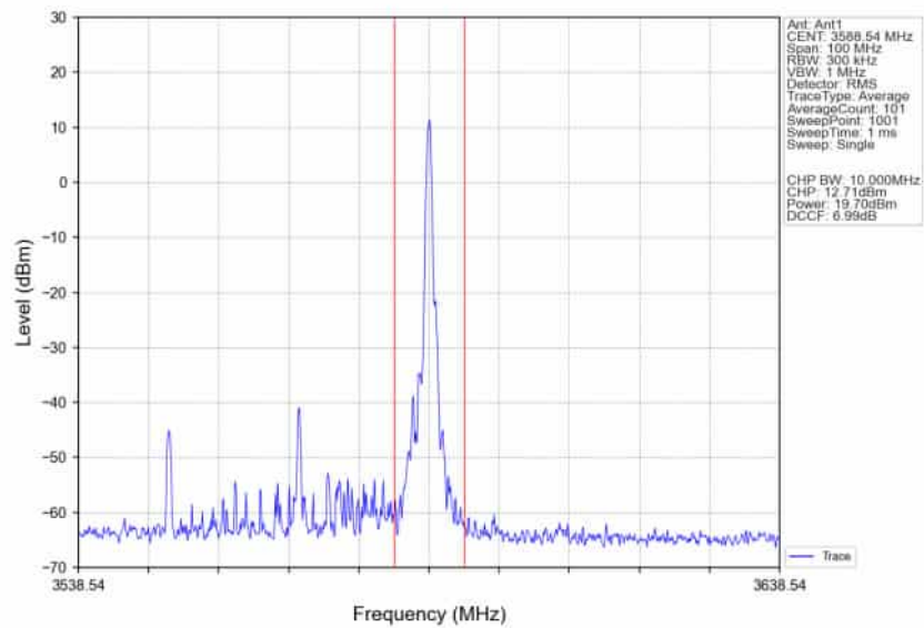
n78d_30kHz_SISO_NTNV_40MHz_CP-OFDM_QPSK_3570MHz_Inner_1RB_Right_Ant1
