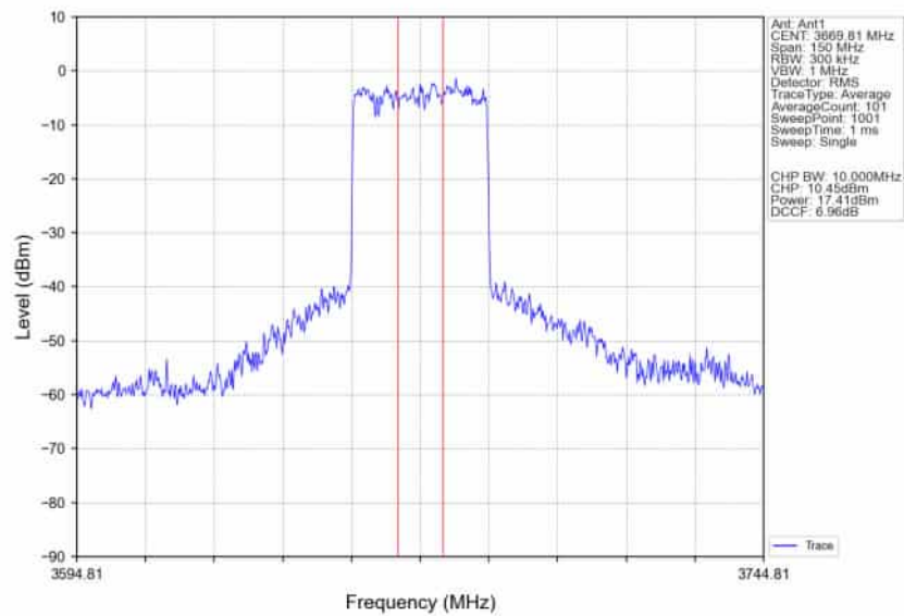
n78d_30kHz_SISO_NTNV_60MHz_DFT-s-OFDM_QPSK_3669.99MHz_Inner_Full_Ant1
