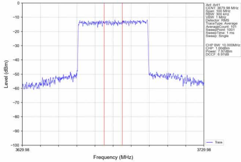
n78d_30kHz_SISO_NTNV_40MHz_CP-OFDM_256_QAM_3679.98MHz_Inner_Full_Ant1
