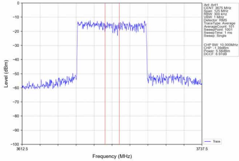
n78d_30kHz_SISO_NTNV_50MHz_CP-OFDM_QPSK_3675MHz_Inner_Full_Ant1
