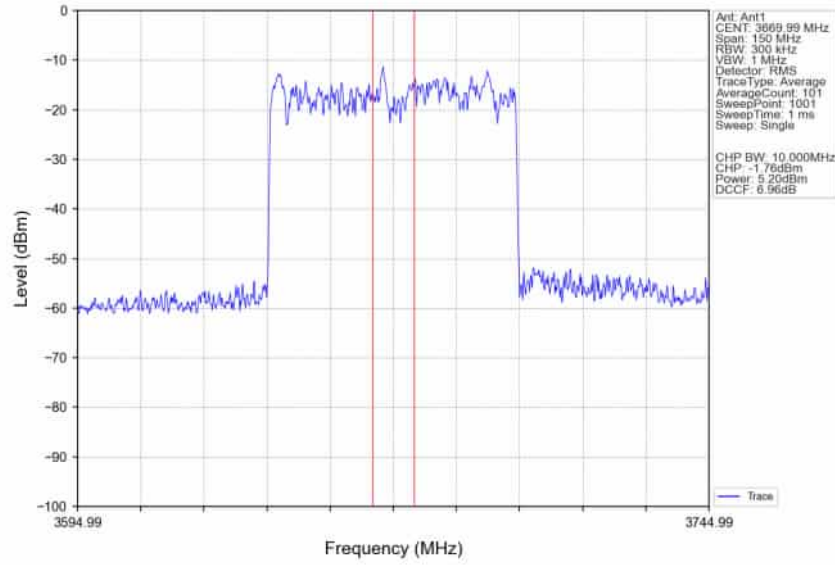
n78d_30kHz_SISO_NTNV_60MHz_DFT-s-OFDM_256_QAM_3669.99MHz_Inner_Full_Ant1
