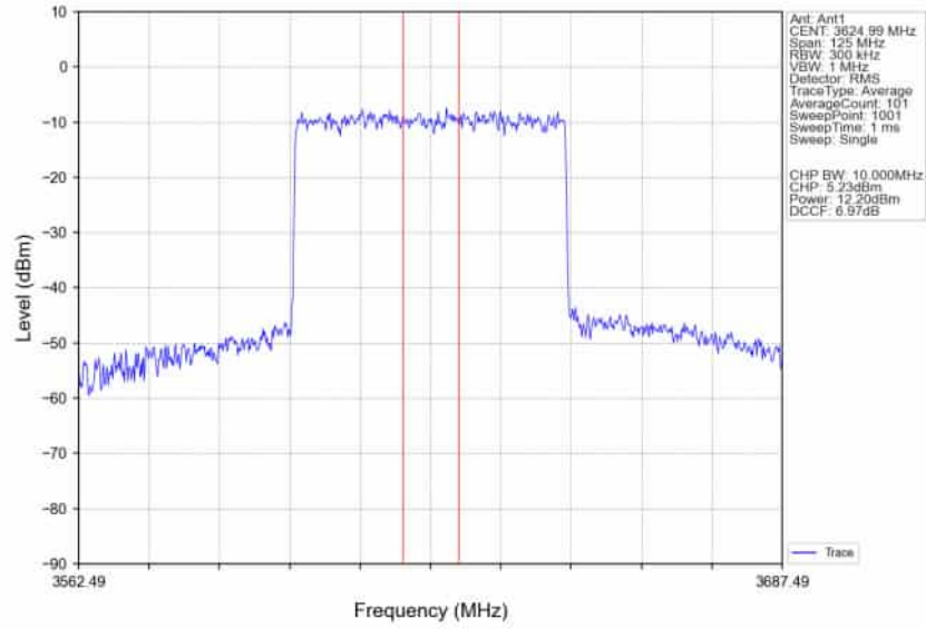
n78d_30kHz_SISO_NTNV_50MHz_CP-OFDM 16 QAM 3624.99MHz_Inner_Full_Ant1
