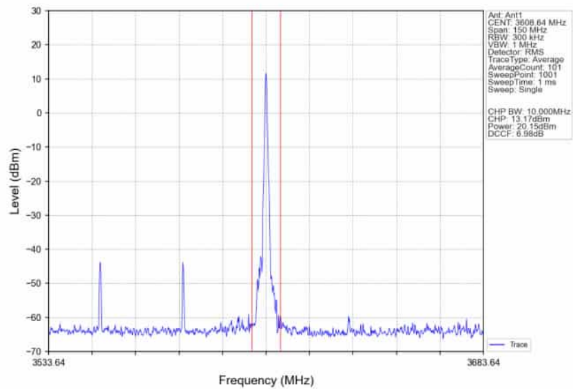
n78d_30kHz_SISO_NTNV_60MHz_DFT-s-OFDM_QPSK_3580.02MHz_Inner_1RB_Right_Ant1
