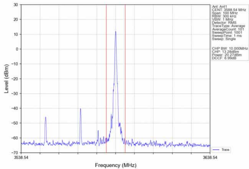
n78d_30kHz_SISO_NTNV_40MHz_CP-OFDM_16_QAM_3570MHz_Inner_1RB_Right_Ant1
