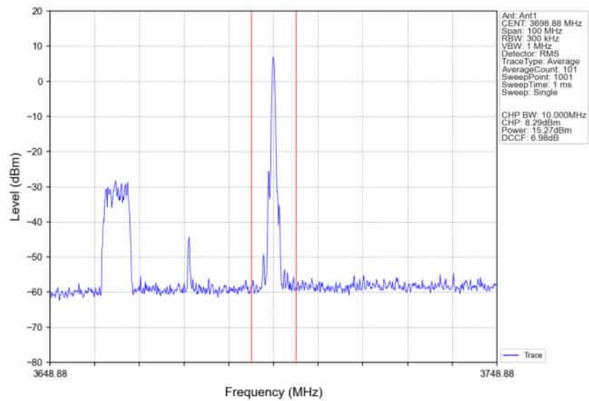
n78d_30kHz_SISO_NTNV_40MHz_CP-OFDM_64_QAM_3679.98MHz_Edge_1RB_Right_Ant1
