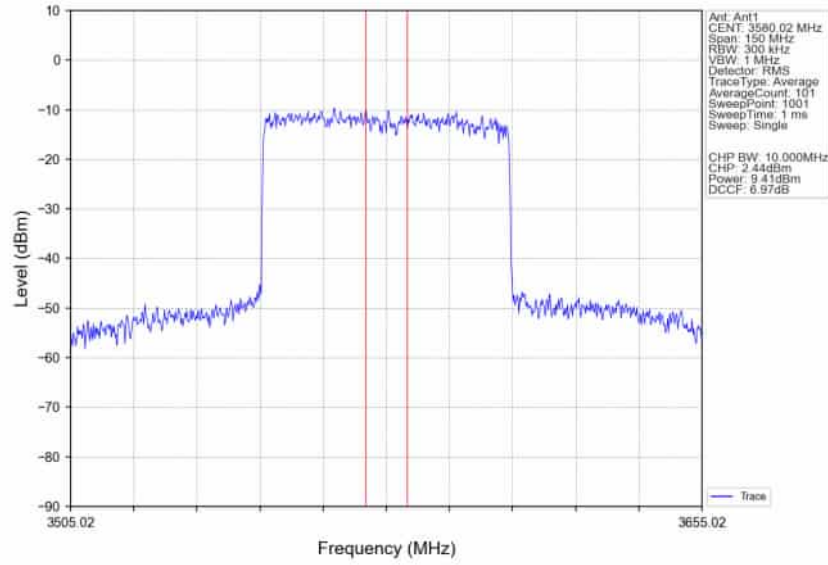
n78d_30kHz_SISO_NTNV_60MHz_CP-OFDM 64 QAM 3580.02MHz_Inner_Full_Ant1
