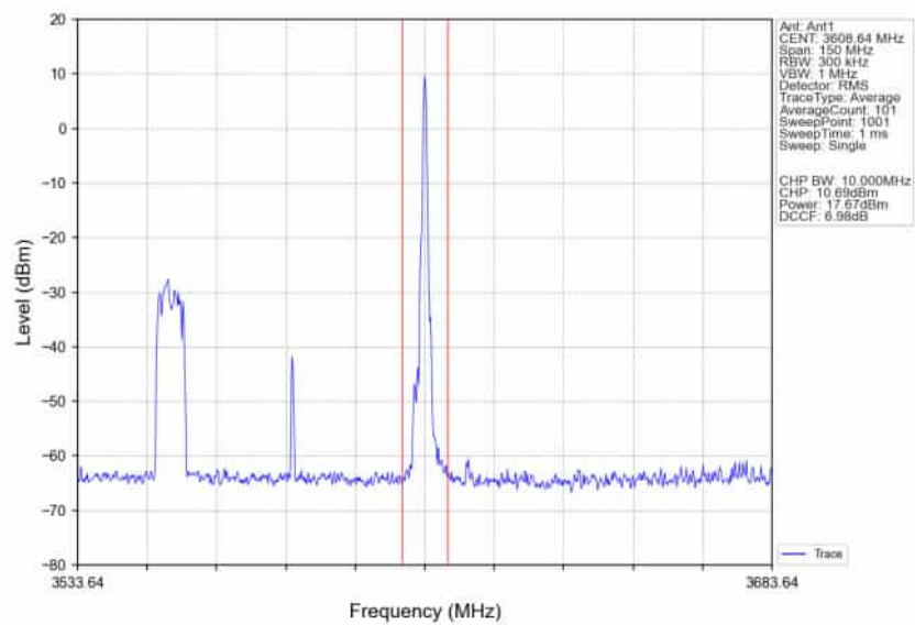
n78d_30kHz_SISO_NTNV_60MHz_DFT-s-OFDM_64_QAM_3580.02MHz_Inner_1RB_Right_Ant1
