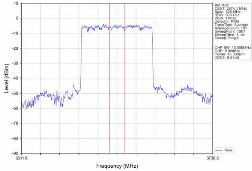
n78d_30kHz_SISO_NTNV_50MHz_DFT-s-OFDM PI/2 BPSK_3675MHz_Inner_Full_Ant1
