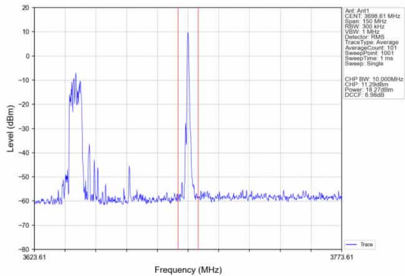
n78d_30kHz_SISO_NTNV_60MHz_DFT-s-OFDM_QPSK_3669.99MHz_Inner_1RB_Right_Ant1
