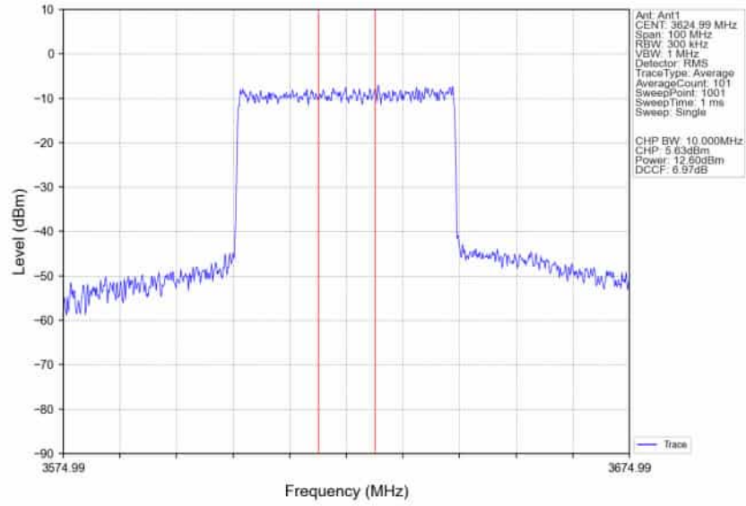
n78d_30kHz_SISO_NTNV_40MHz_CP-OFDM_QPSK_3624.99MHz_Inner_Full_Ant1
