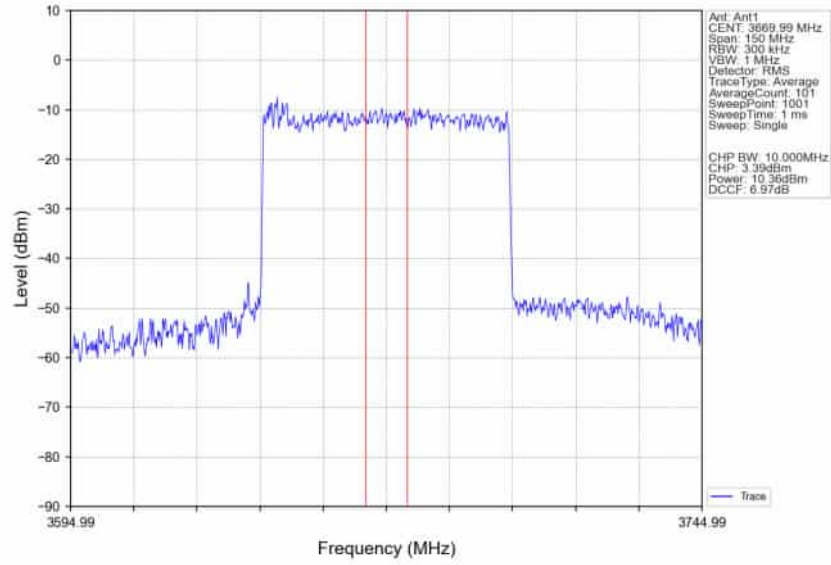
n78d_30kHz_SISO_NTNV_60MHz_CP-OFDM 16 QAM 3669.99MHz_Inner_Full_Ant1
