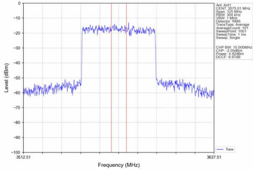
n78d_30kHz_SISO_NTNV_50MHz_CP-OFDM_256_QAM_3575.01MHz_Inner_Full_Ant1
