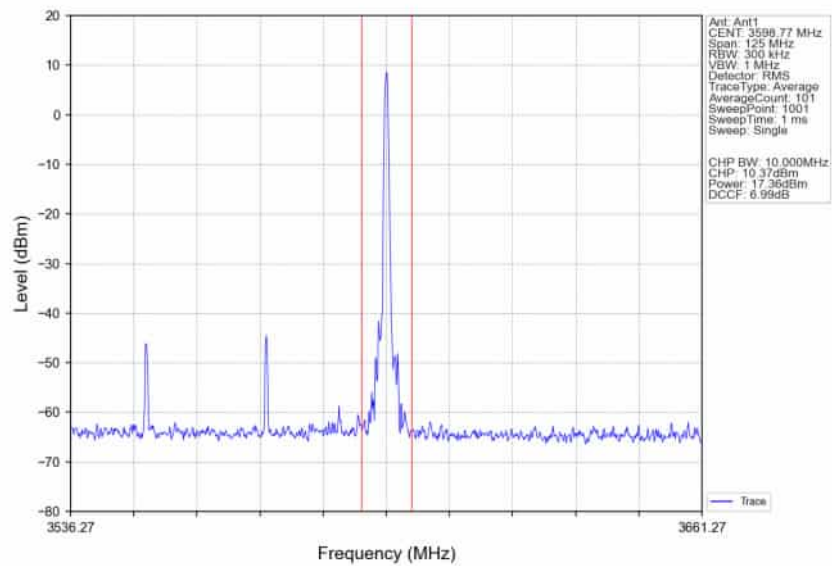
n78d_30kHz_SISO_NTNV_50MHz_DFT-s-OFDM_64_QAM_3575.01MHz_Edge_1RB_Right_Ant1
