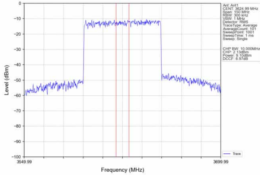
n78d_30kHz_SISO_NTNV_60MHz_CP-OFDM_QPSK_3624.99MHz_Inner_Full_Ant1
