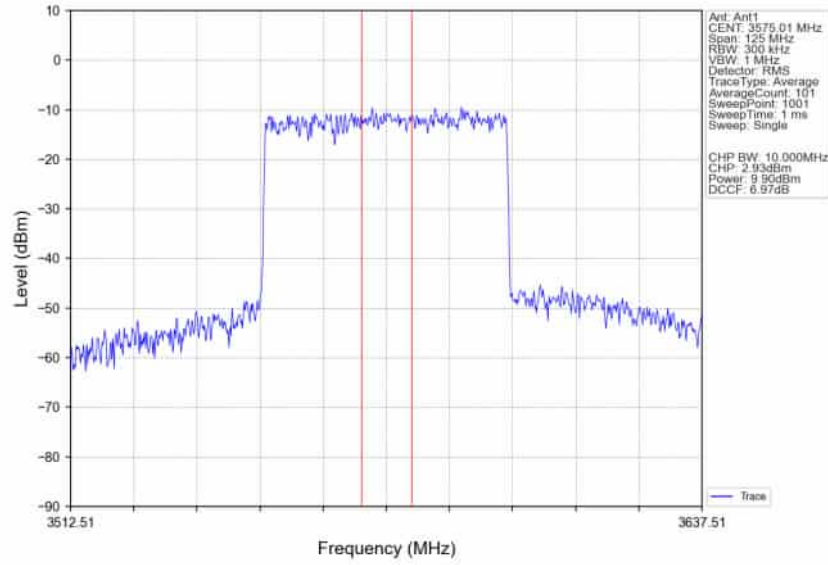
n78d_30kHz_SISO_NTNV_50MHz_CP-OFDM_QPSK_3575.01MHz_Inner_Full_Ant1
