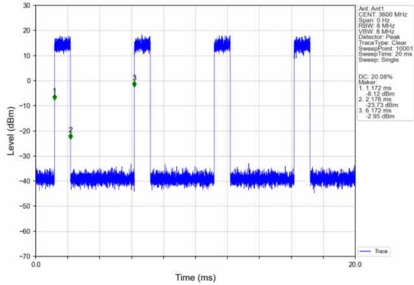
n78d_30kHz_SISO_NTNV_100MHz_CP-OFDM_QPSK_3600MHz_Inner_Full_Ant1
