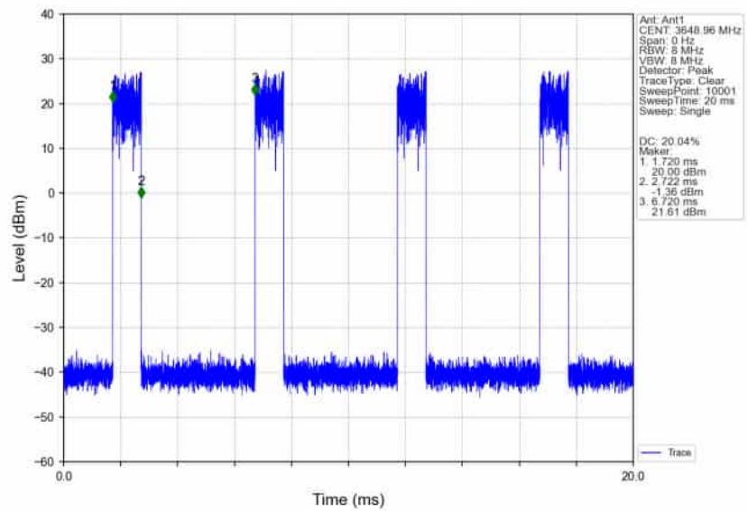
n78d_30kHz_SISO_NTNV_100MHz_CP-OFDM_64_QAM_3600MHz_Edge_1RB_Right_Ant1
