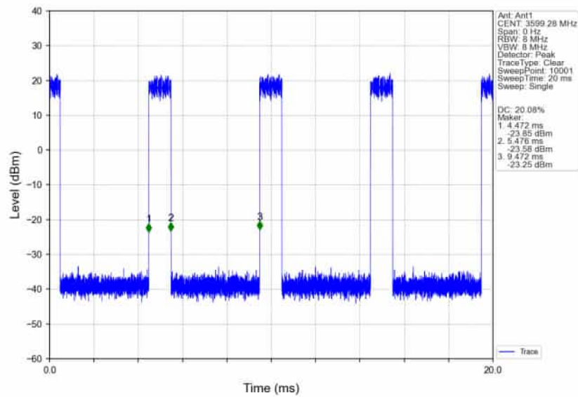
n78d_30kHz_SISO_NTNV_100MHz_DFT-s-OFDM_16_QAM_3600MHz_Inner_Full_Ant1
