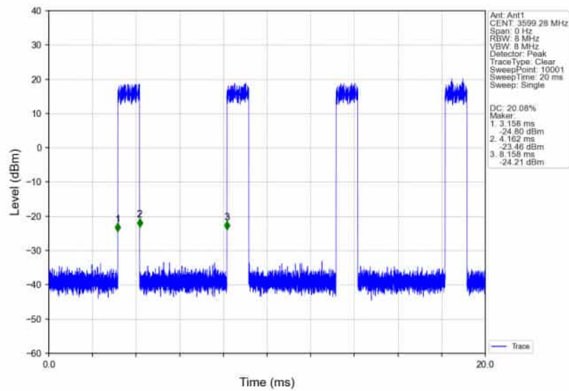
n78d_30kHz_SISO_NTNV_100MHz_DFT-s-OFDM_256_QAM_3600MHz_Inner_Full_Ant1
