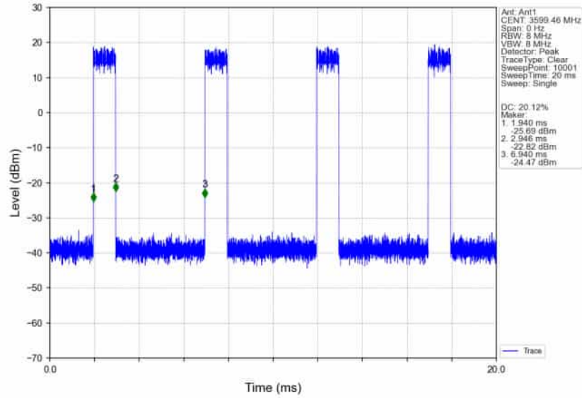
n78d_30kHz_SISO_NTNV_100MHz_DFT-s-OFDM_16_QAM_3600MHz_Inner_Full_Ant1
