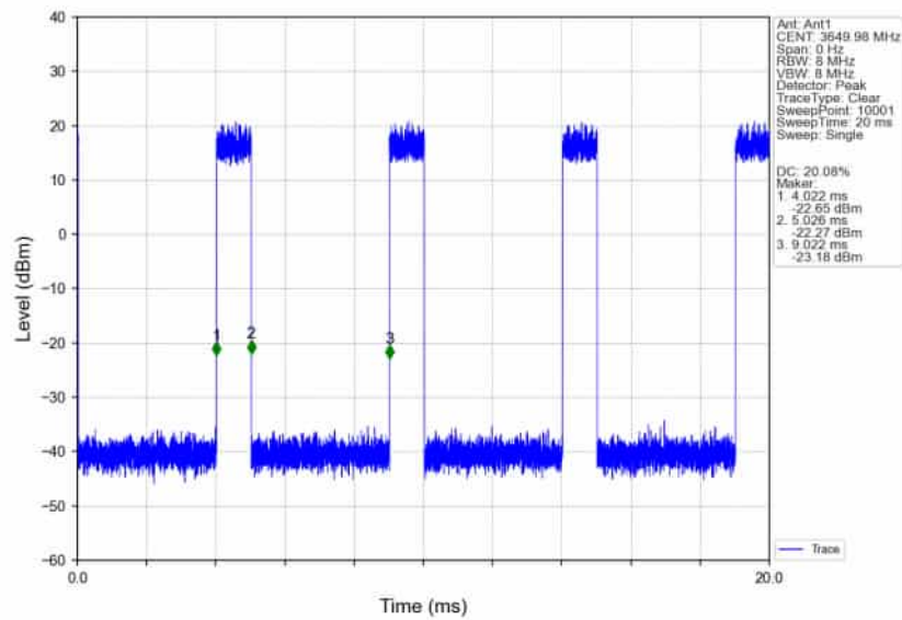
n78d_30kHz_SISO_NTNV_100MHz_CP-OFDM 64 QAM_3649.98MHz_Inner_Full_Ant1
