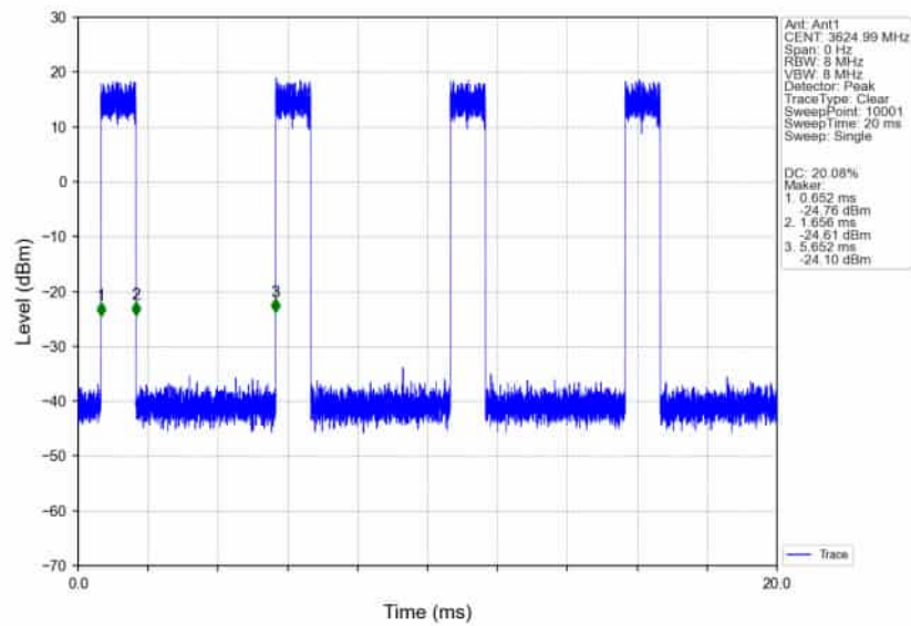
n78d_30kHz_SISO_NTNV_80MHz_CP-OFDM_256_QAM_3624.99MHz_Inner_Full_Ant1
