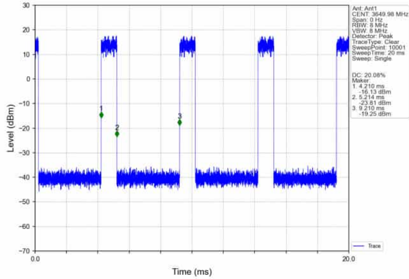
n78d_30kHz_SISO_NTNV_100MHz_CP-OFDM 64 QAM_3649.98MHz_Inner_Full_Ant1
