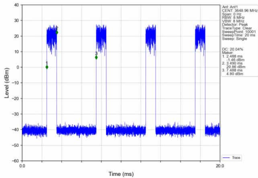
n78d_30kHz_SISO_NTNV_100MHz_CP-OFDM_16_QAM_3600MHz_Edge_1RB_Right_Ant1
