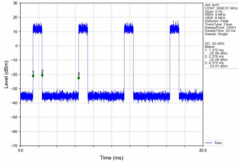
n78d_30kHz_SISO_NTNV_80MHz_CP-OFDM_256_QAM_3590.01MHz_Inner_Full_Ant1
