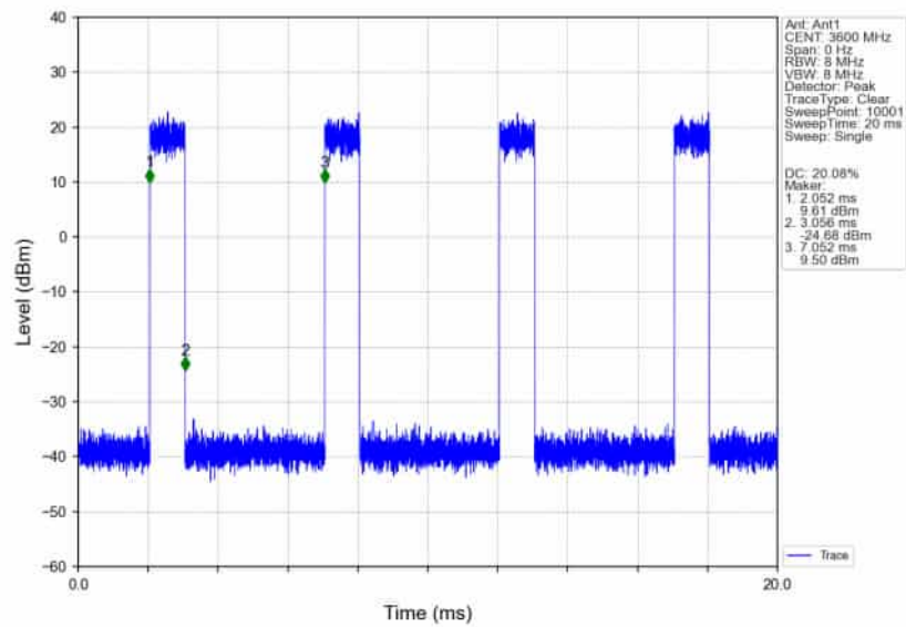
n78d_30kHz_SISO_NTNV_100MHz_CP-OFDM_QPSK_3600MHz_Inner_Full_Ant1
