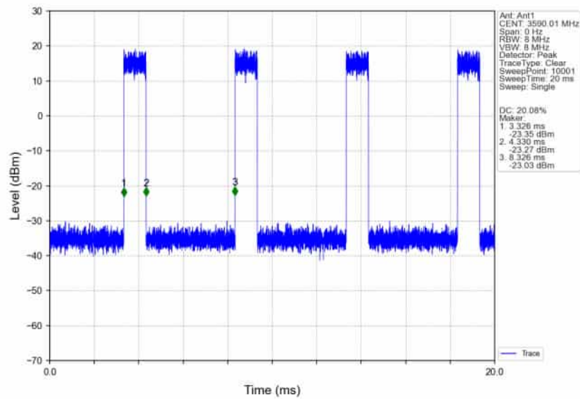
n78d_30kHz_SISO_NTNV_80MHz_CP-OFDM_256_QAM_3590.01MHz_Inner_Full_Ant1
