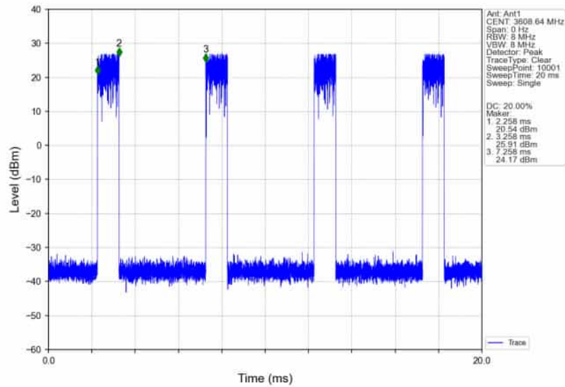
n78d_30kHz_SISO_NTNV_60MHz_CP-OFDM_16_QAM_3580.02MHz_Inner_1RB_Right_Ant1
