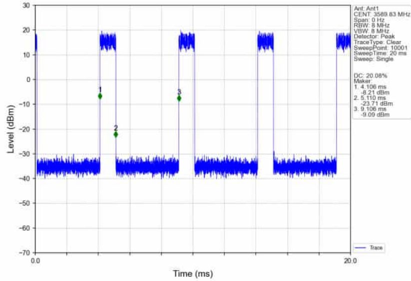
n78d_30kHz_SISO_NTNV_80MHz_DFT-s-OFDM_64_QAM_3590.01MHz_Inner_Full_Ant1
