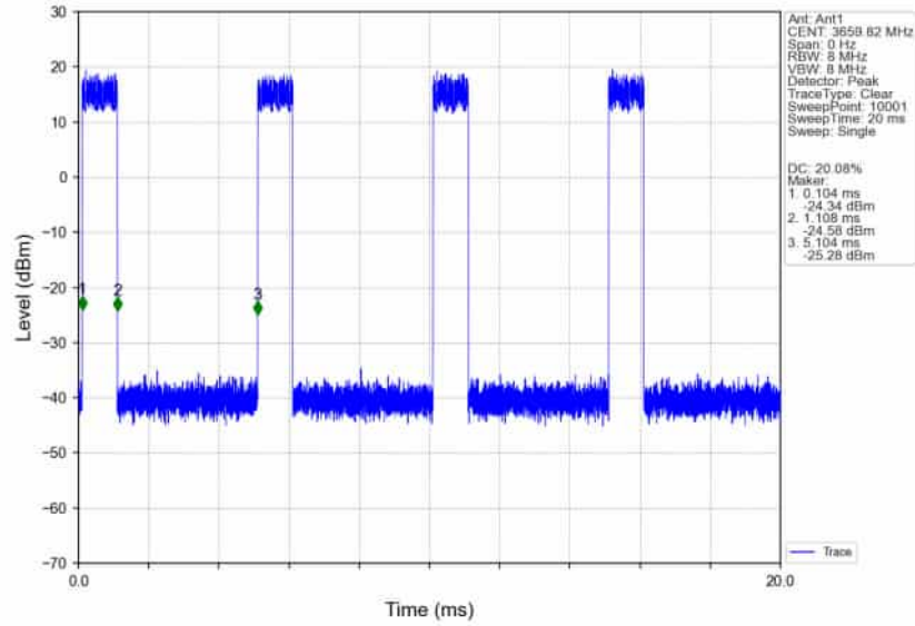
n78d_30kHz_SISO_NTNV_80MHz_DFT-s-OFDM 64 QAM 3660MHz_Inner_Full_Ant1
