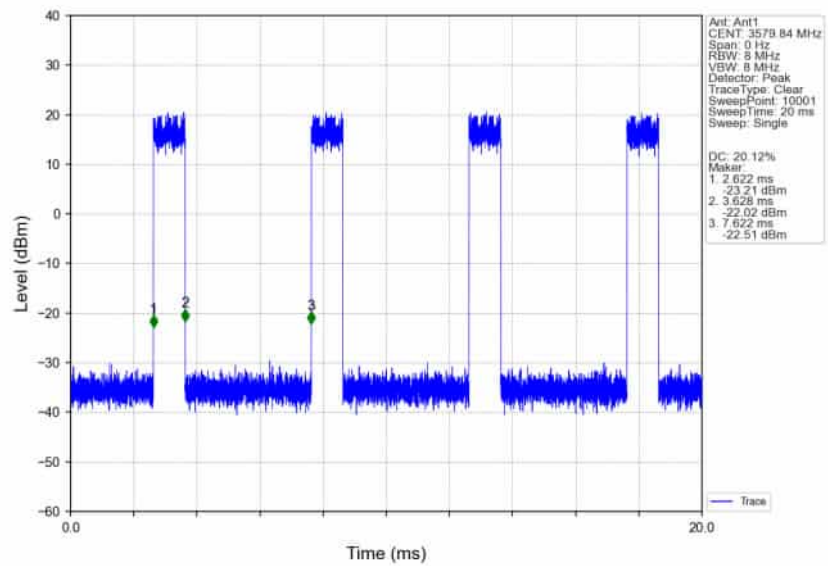
n78d_30kHz_SISO_NTNV_60MHz_CP-OFDM_256_QAM_3580.02MHz_Inner_Full_Ant1
