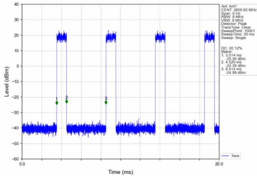
n78d_30kHz_SISO_NTNV_80MHz_DFT-s-OFDM_16_QAM_3660MHz_Inner_Full_Ant1
