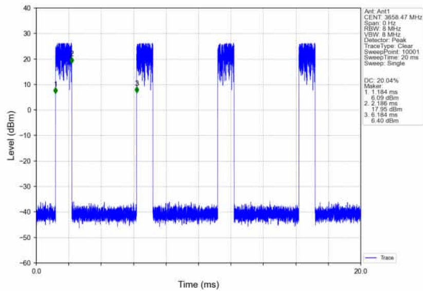
n78d_30kHz_SISO_NTNV_70MHz_CP-OFDM_16_QAM_3624.99MHz_Inner_1RB_Right_Ant1
