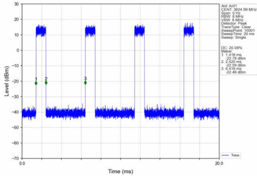
n78d_30kHz_SISO_NTNV_60MHz_CP-OFDM_256_QAM_3624.99MHz_Inner_Full_Ant1
