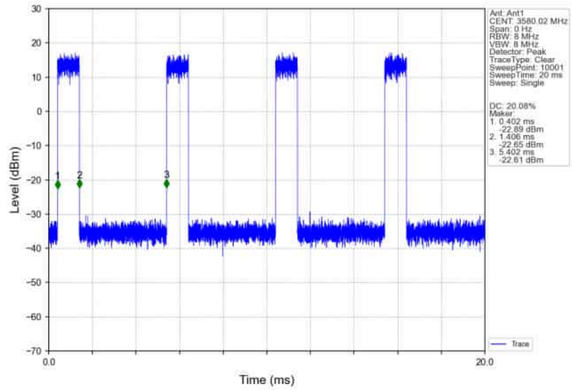
n78d_30kHz_SISO_NTNV_60MHz_CP-OFDM_256_QAM_3580.02MHz_Inner_Full_Ant1
