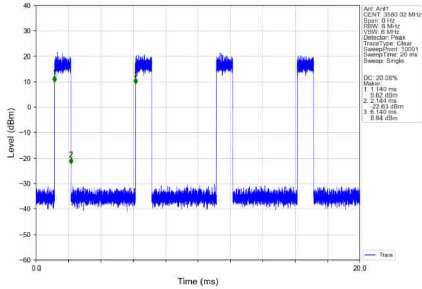
n78d_30kHz_SISO_NTNV_60MHz_CP-OFDM_QPSK_3580.02MHz_Inner_Full_Ant1
