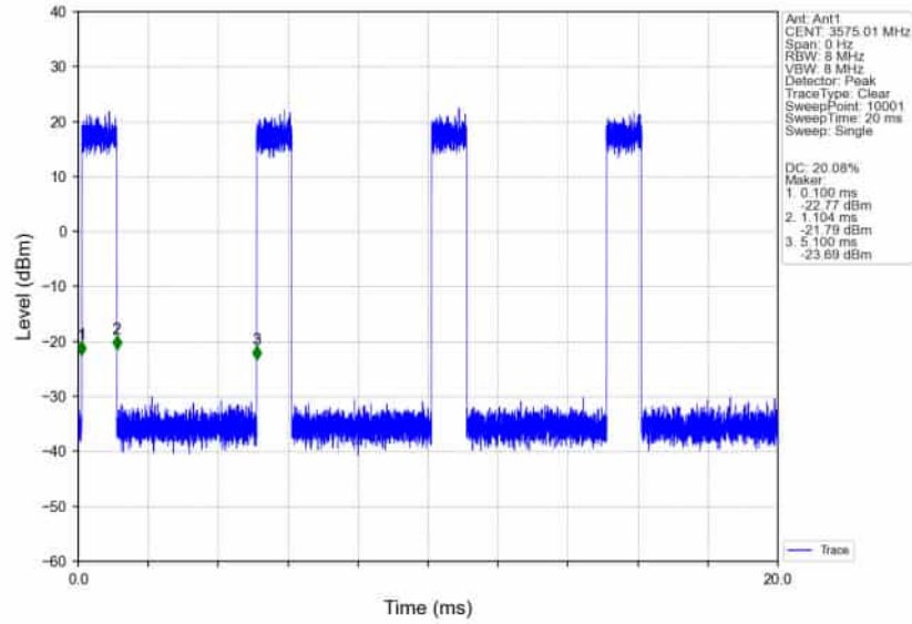
n78d_30kHz_SISO_NTNV_50MHz_CP-OFDM_QPSK_3575.01MHz_Inner_Full_Ant1
