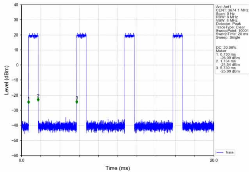
n78d_30kHz_SISO_NTNV_50MHz_DFT-s-OFDM_PI/2_BPSK_3675MHz_Inner_Full_Ant1
