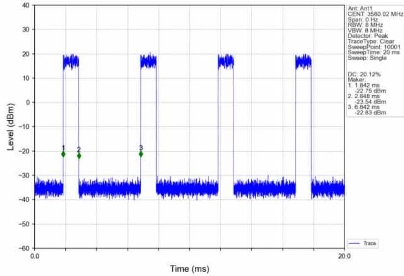
n78d_30kHz_SISO_NTNV_60MHz_DFT-s-OFDM_PI/2_BPSK_3580.02MHz_Inner_Full_Ant1
