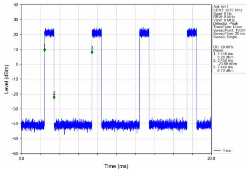
n78d_30kHz_SISO_NTNV_50MHz_CP-OFDM_16_QAM_3675MHz_Inner_Full_Ant1
