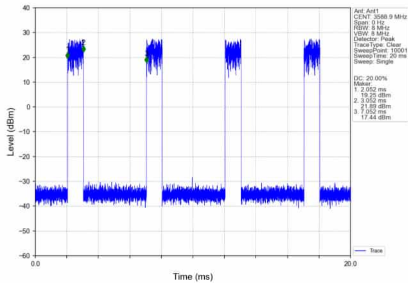
n78d_30kHz_SISO_NTNV_40MHz_DFT-s-OFDM_16_QAM_3570MHz_Edge_1RB_Right_Ant1
