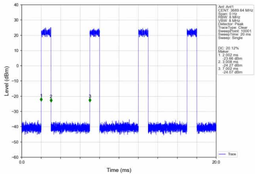
n78d_30kHz_SISO_NTNV_20MHz_DFT-s-OFDM_256_QAM_3690MHz_Inner_Full_Ant1
