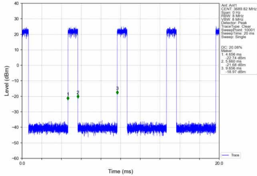
n78d_30kHz_SISO_NTNV_20MHz_DFT-s-OFDM_16_QAM_3690MHz_Inner_Full_Ant1
