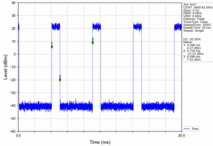
n78d_30kHz_SISO_NTNV_20MHz_DFT-s-OFDM 64 QAM 3690MHz_Inner_Full_Ant1
