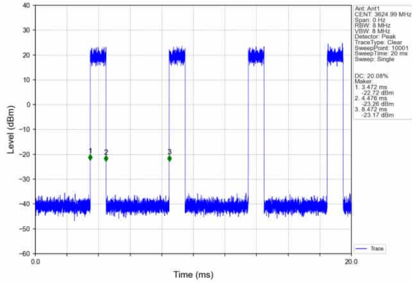
n78d_30kHz_SISO_NTNV_30MHz_CP-OFDM 16 QAM 3624.99MHz_Inner_Full_Ant1
