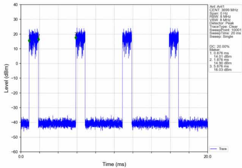
n78d_30kHz_SISO_NTNV_20MHz_CP-OFDM_256_QAM_3690MHz_Edge_1RB_Right_Ant1
