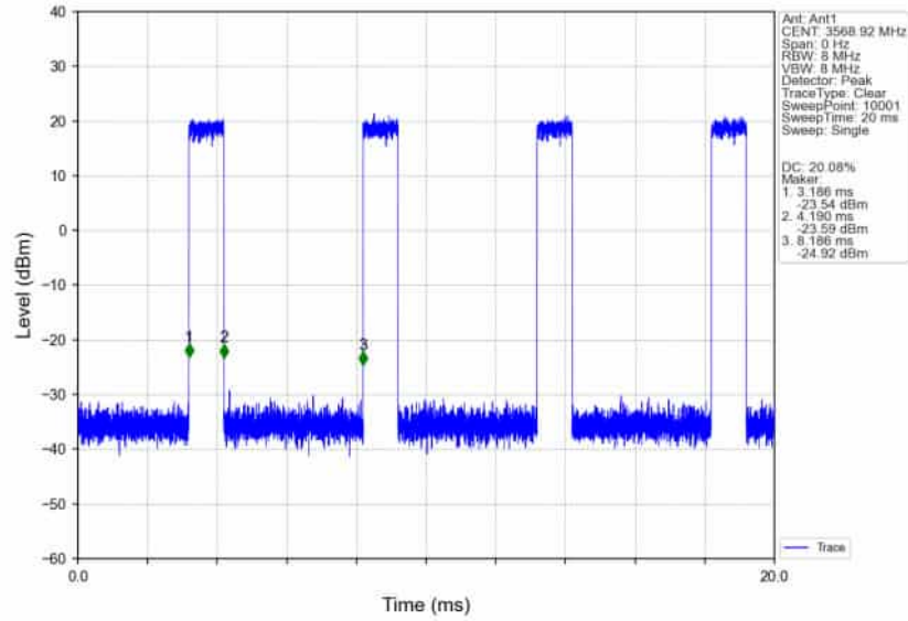
n78d_30kHz_SISO_NTNV_40MHz_DFT-s-OFDM_PI/2_BPSK_3570MHz_Inner_Full_Ant1
