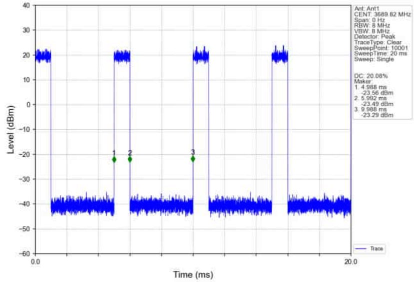
n78d_30kHz_SISO_NTNV_20MHz_DFT-s-OFDM_256_QAM_3690MHz_Inner_Full_Ant1
