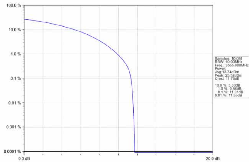
n48_30kHz_SISO_NTNV_10MHz_CP-OFDM_64_QAM_3555MHz_Outer_Full
