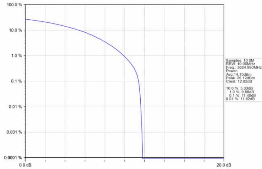
n48_30kHz_SISO_NTNV_10MHz_CP-OFDM_64_QAM_3624.99MHz_Outer_Full
