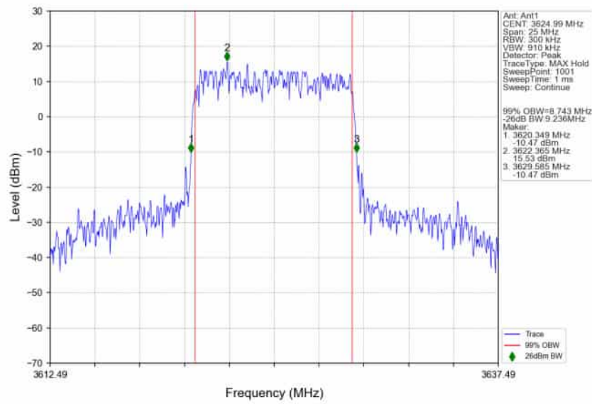
n48_30kHz_SISO_NTNV_10MHz_DFT-s-OFDM_16_QAM_3624.99MHz_Outer_Full
