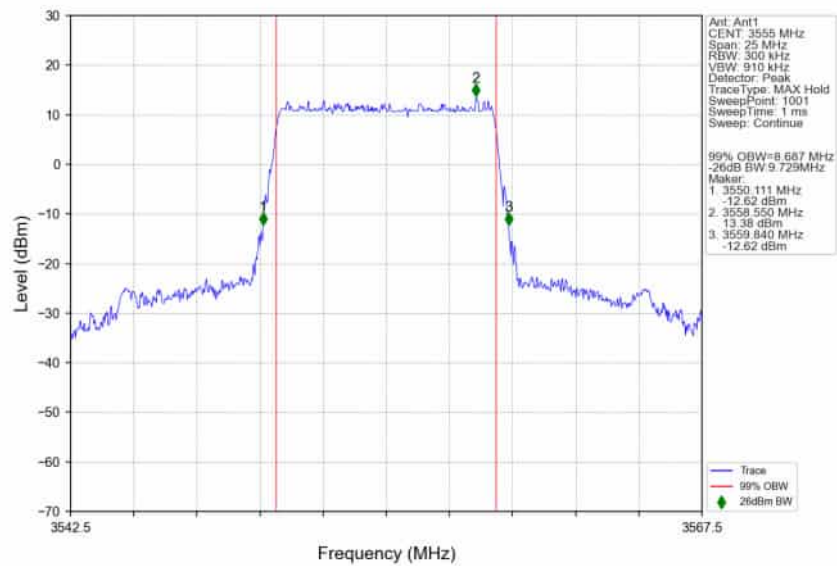
n48 30kHz SISO NTN 10MHz DFT-s-OFDM 64 QAM 3555MHz Outer Full
