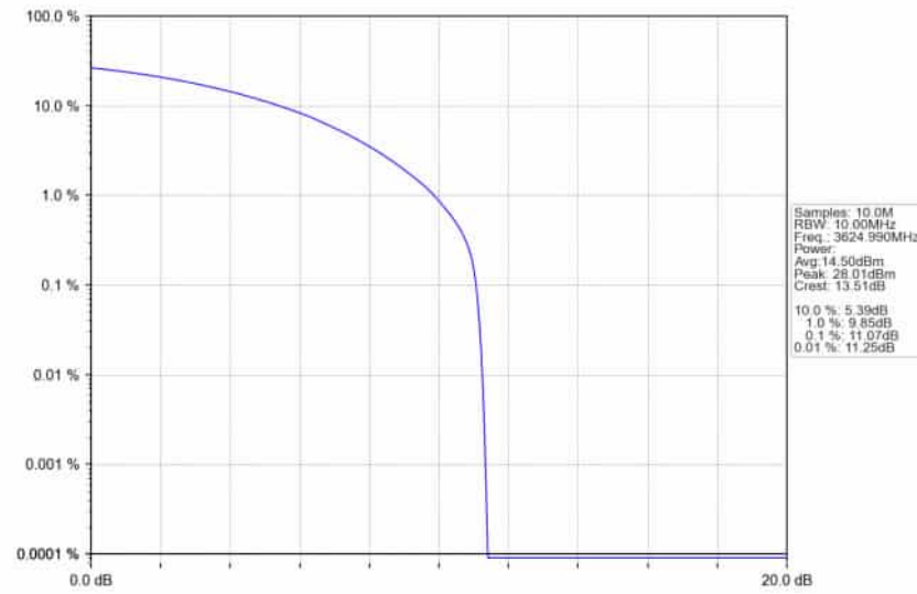
n48_30kHz_SISO_NTNV_10MHz_CP-OFDM_QPSK_3624.99MHz_Outer_Full
