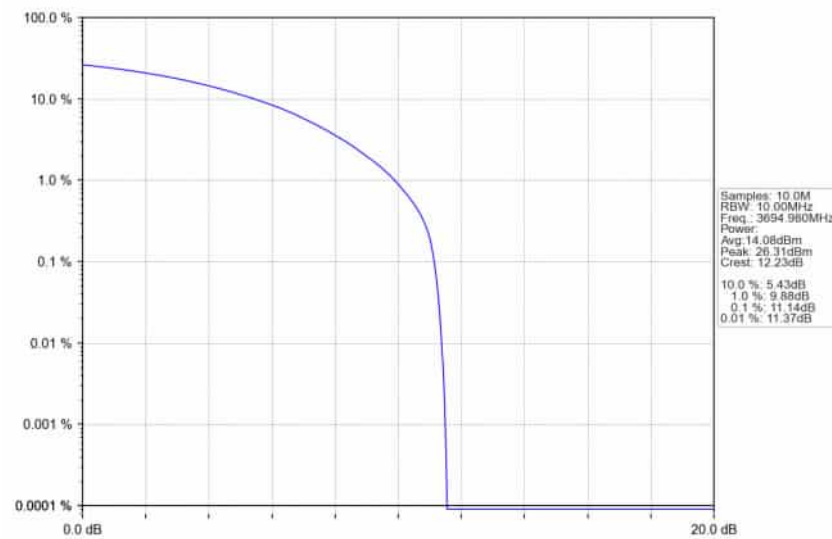
n48_30kHz_SISO_NTNV_10MHz_CP-OFDM_QPSK_3694.98MHz_Outer_Full
