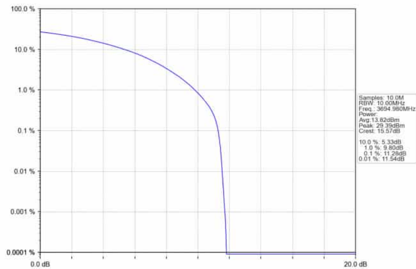
n48_30kHz_SISO_NTNV_10MHz_CP-OFDM_64_QAM_3694.98MHz_Outer_Full
