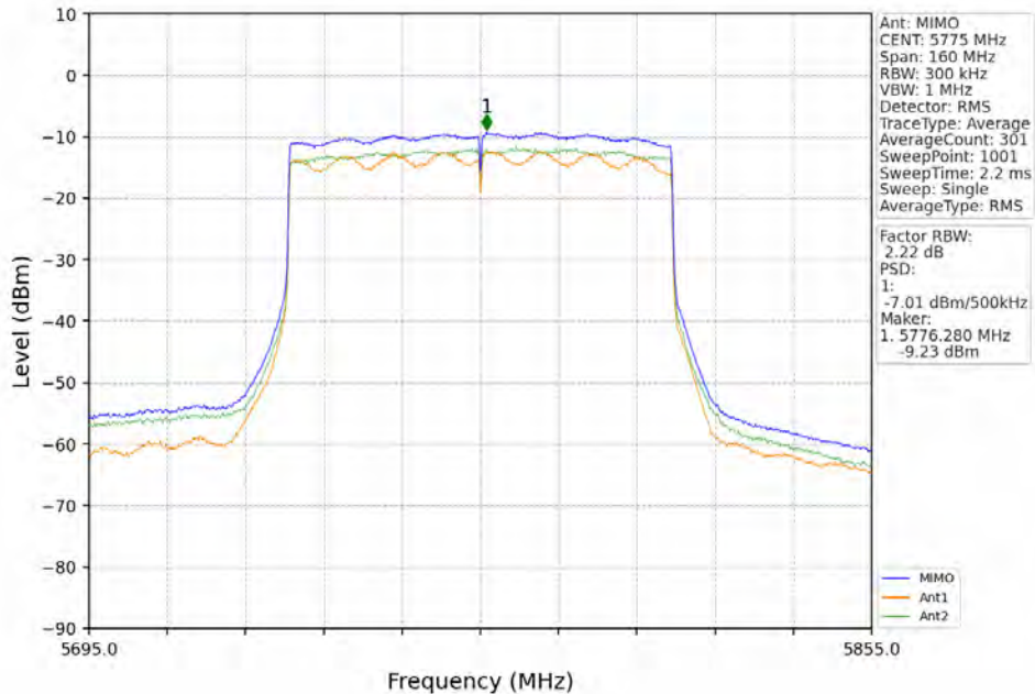
802.11ax(HEW80)_MCH_5775MHz_RU996_Left_MIMO_NTNV
