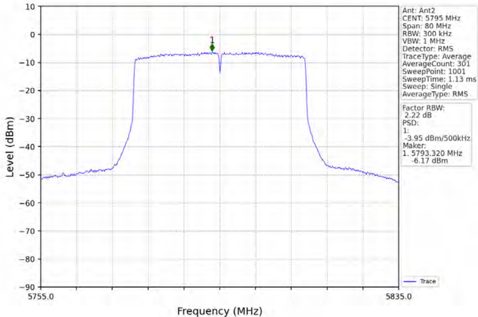
802.11ax(HEW40)_HCH_5795MHz_RU484_Left_MIMO_NTNV
