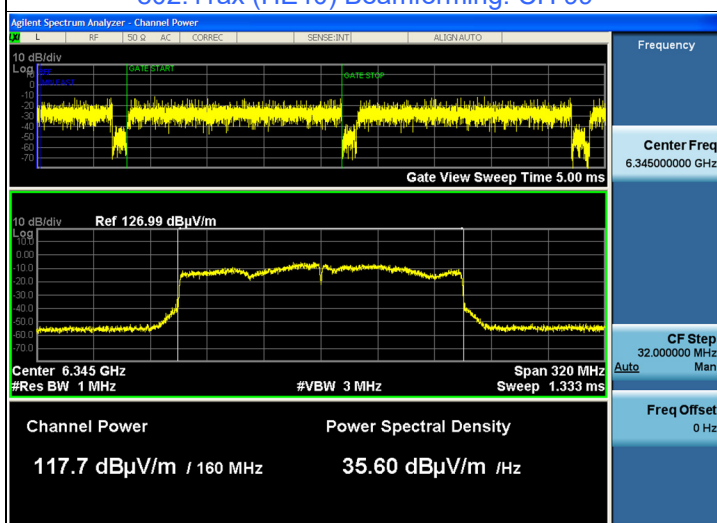
802.11ax (HE160) Beamforming: CH 79
