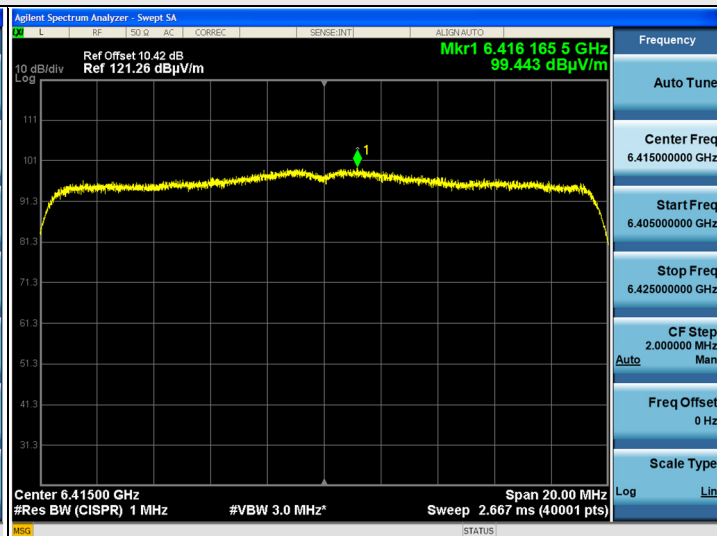
802.11ax (HE20) Beamforming: CH 93
