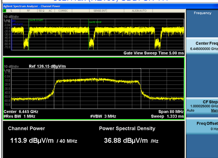
802.11ax (HE40) Beamforming: CH 99
