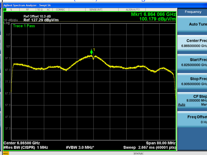
802.11ax (HE80) Beamforming: CH 183
