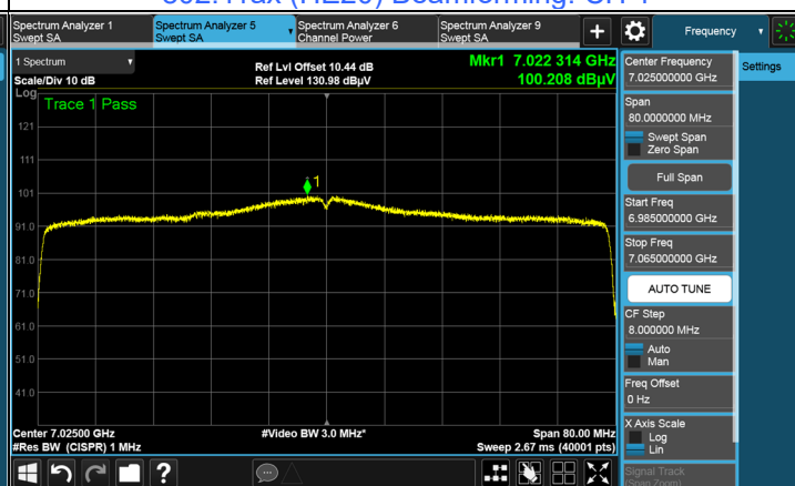
802.11ax (HE80) Beamforming: CH 215
