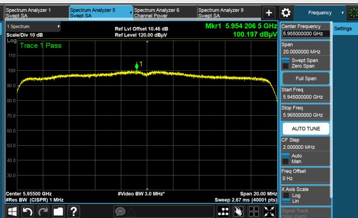
802.11ax (HE20) Beamforming: CH 1
