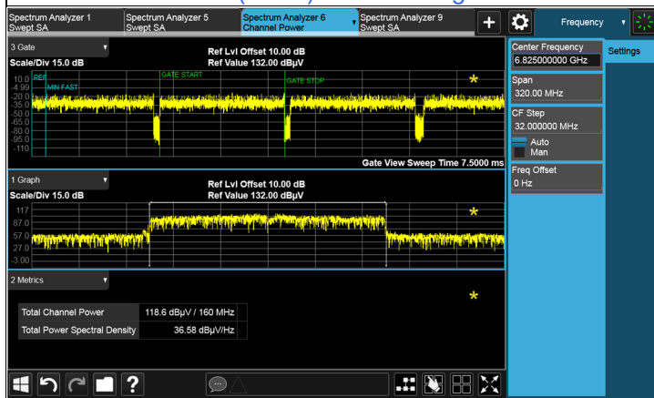
802.11ax (HE160) Beamforming: CH 175
