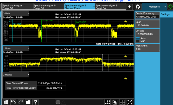
802.11ax (HE80) Beamforming: CH 119
