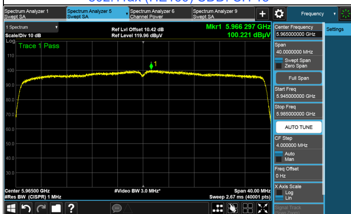
802.11ax (HE40) Beamforming: CH 3
