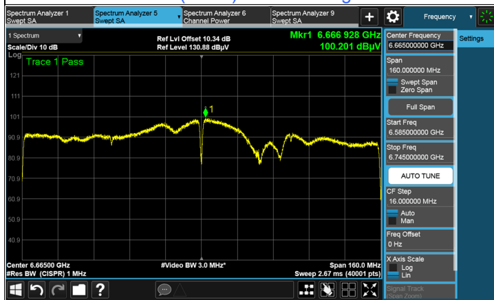
802.11ax (HE160) Beamforming: CH 143
