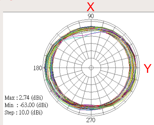
H plane
