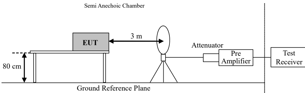
Figure 4: Test Setup
