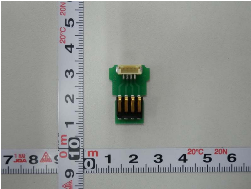
Board2 (Top)
