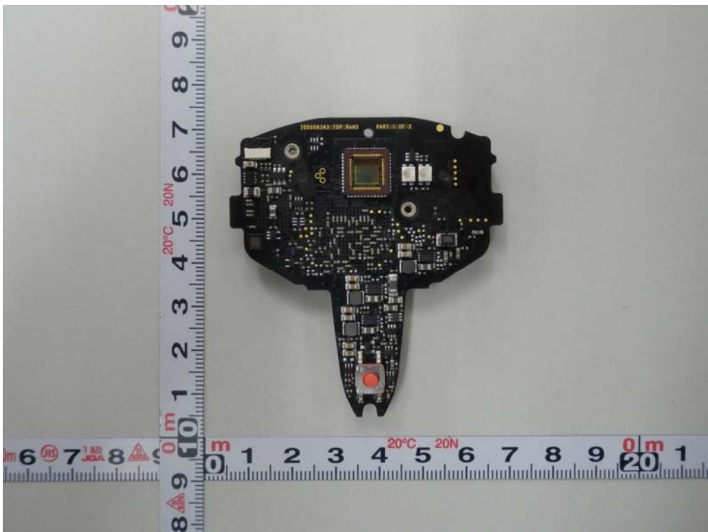
Board1 (Bottom)
