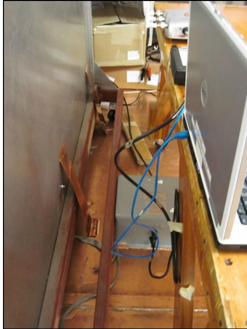
Photograph 3. Conducted Emissions, Test Setup 2
