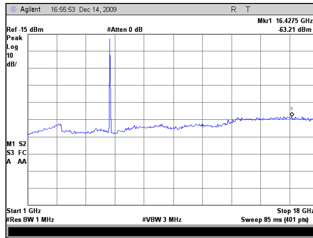
Plot 118. Radiated Spurious, 802.11n 20MHz, 5785 MHz, 1 GHz – 18 GHz, 9 dBi Omni
