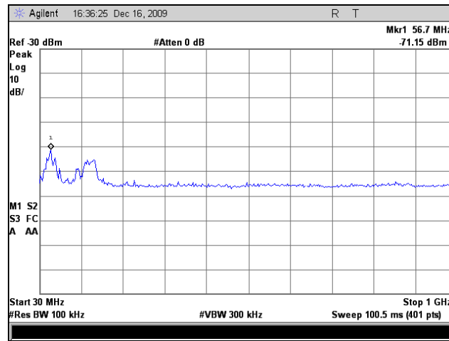
Plot 121. Radiated Spurious, 802.11n 20MHz, 5745 MHz, 30 MHz – 1 GHz, 16 dBi Sector
