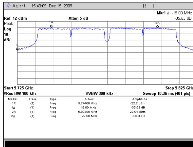
Plot 208. Frequency Stability, 802.11n 40MHz Bandwidth, -40C, 108 VAC
