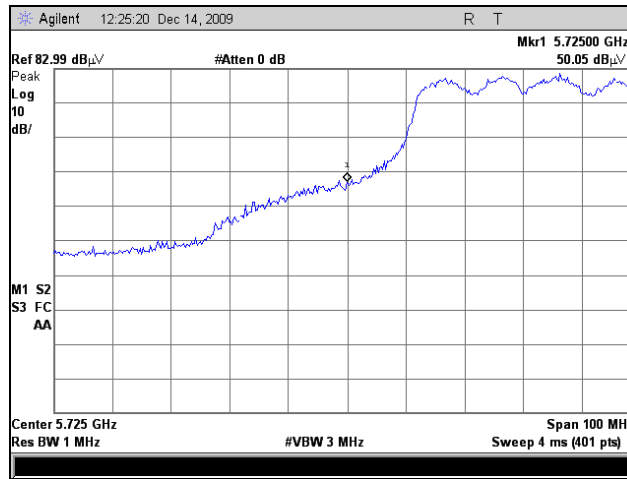
Plot 174. EIRP, 802.11n 40MHz, Low Channel, 5755 MHz, 5 dBi Omni
