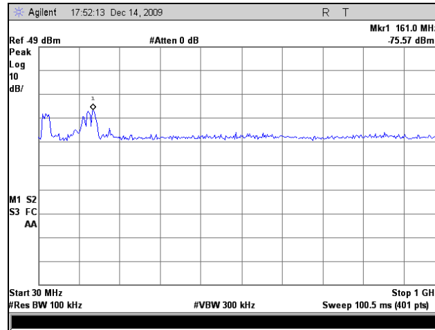
Plot 133. Radiated Spurious, 802.11n 40MHz, 5755 MHz, 30 MHz – 1 GHz, 5 dBi Omni
