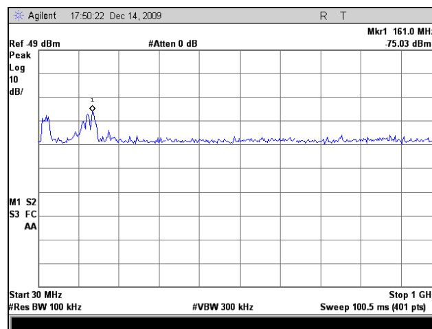
Plot 111. Radiated Spurious, 802.11n 20MHz, 5785 MHz, 30 MHz – 1 GHz, 5 dBi Omni
