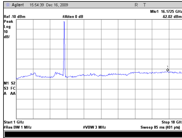
Plot 148. Radiated Spurious, 802.11n 40MHz, 5795 MHz, 1 GHz – 18 GHz, 19 dBi Panel
