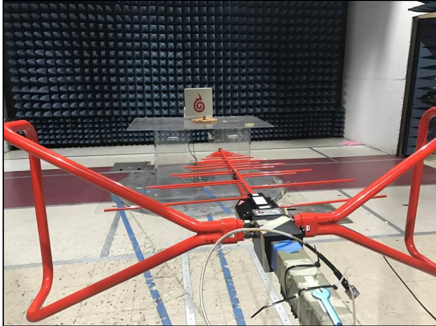
Photograph 5. Radiated Spurious Emissions, Test Setup, 30 MHz – 1 GHz, 19 dBi Antenna
