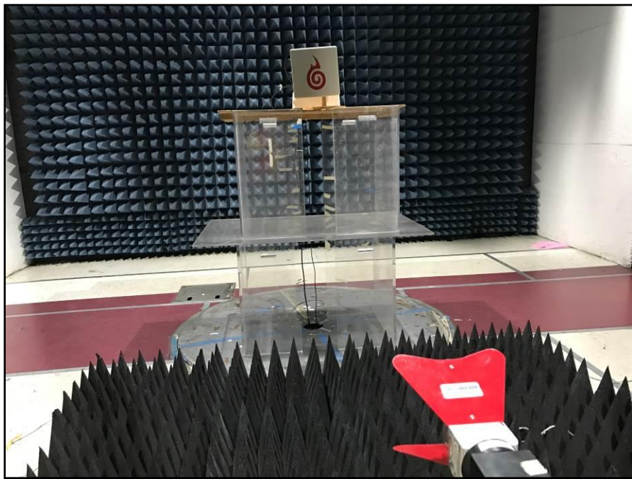
Photograph 6. Radiated Spurious Emissions, Test Setup, Above 1 GHz, 19 dBi Antenna
