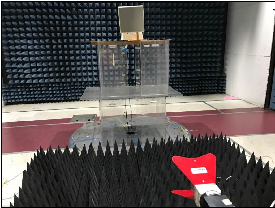
Photograph 4. Radiated Spurious Emissions, Test Setup, Above 1 GHz, 16 dBi Antenna
