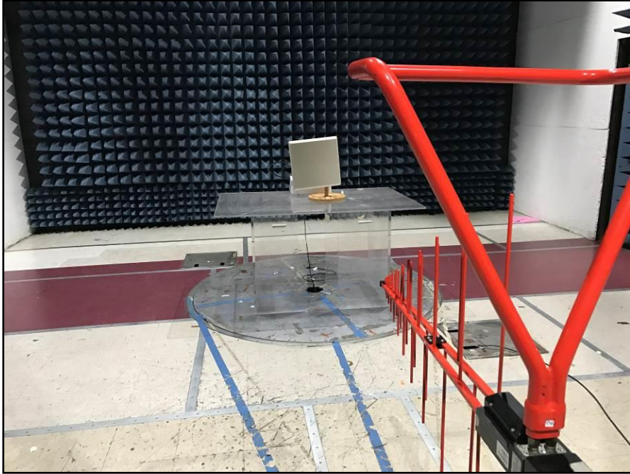
Photograph 3. Radiated Spurious Emissions, Test Setup, 30 MHz – 1 GHz, 16 dBi Antenna
