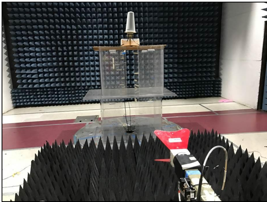
Photograph 2. Radiated Spurious Emissions, Test Setup, Above 1 GHz, 9 dBi Antenna
