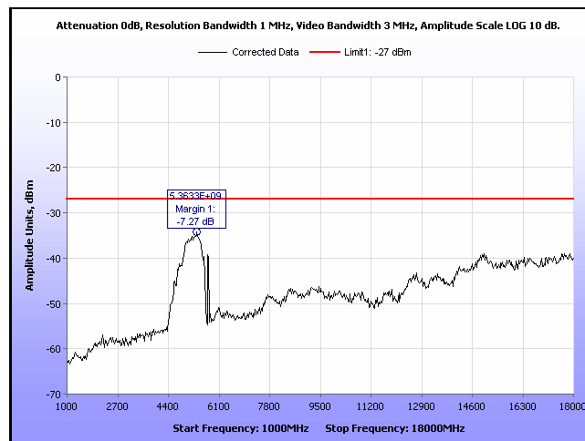
Plot 31. Radio Spurious Emission, 1 GHz - 18 GHz -27 dBm, Bandwidth 20M, Ch. 5745M, a mode, 19 dB
