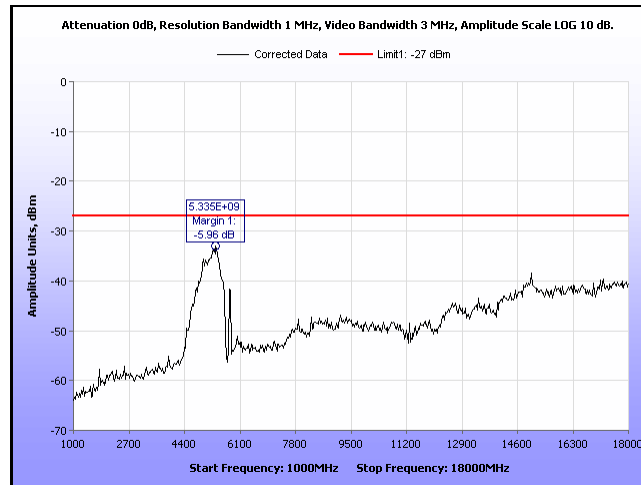
Plot 26. Radio Spurious Emission, 1 GHz - 18 GHz -27 dBm, Bandwidth 20M, Ch.5805M, n mode, 19 dBm
