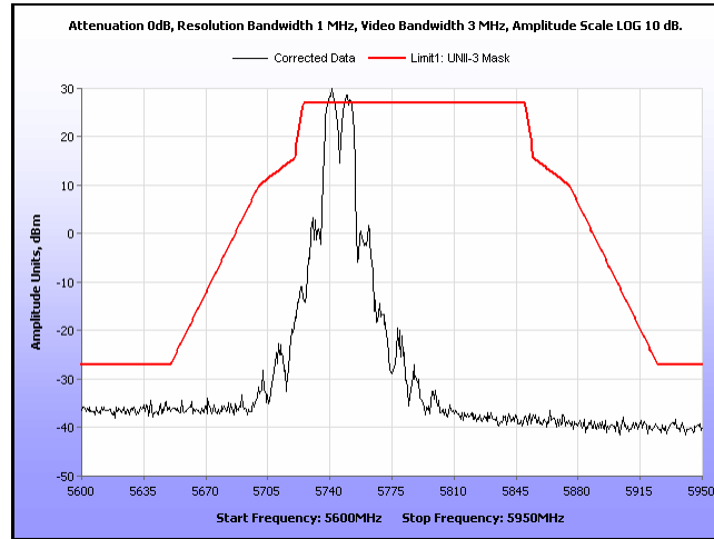
Plot 47. UNII-3 Mask, 11a, 20 MHz, 5745 MHz, 16 dB
