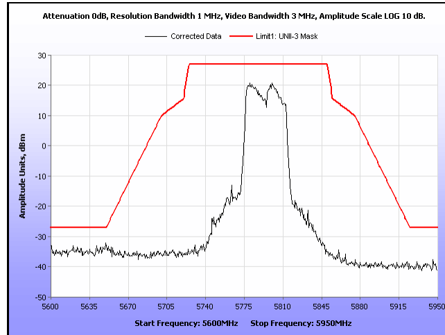
Plot 48. UNII-3 Mask, 11n, 40 MHz, 5795 MHz, 19 dB
