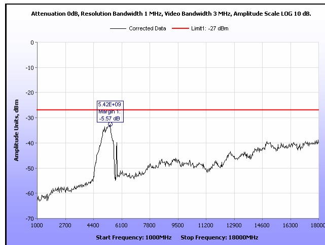
Plot 27. Radio Spurious Emission, 1 GHz - 18 GHz -27 dBm, Bandwidth 20M, Ch. 5805M, a mode, 19 dBm
