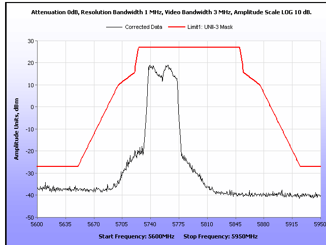
Plot 49. UNII-3 Mask, 11n, 40 MHz, 5755 MHz, 19 dB
