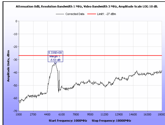
Plot 29. Radio Spurious Emission, 1 GHz - 18 GHz -27 dBm, Bandwidth 20M, Ch. 5785M, a mode, 19 dB
