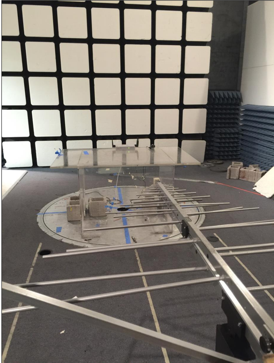
Photograph 1. Radiated Spurious Emissions, Test Setup, 30 MHz -1 GHz
