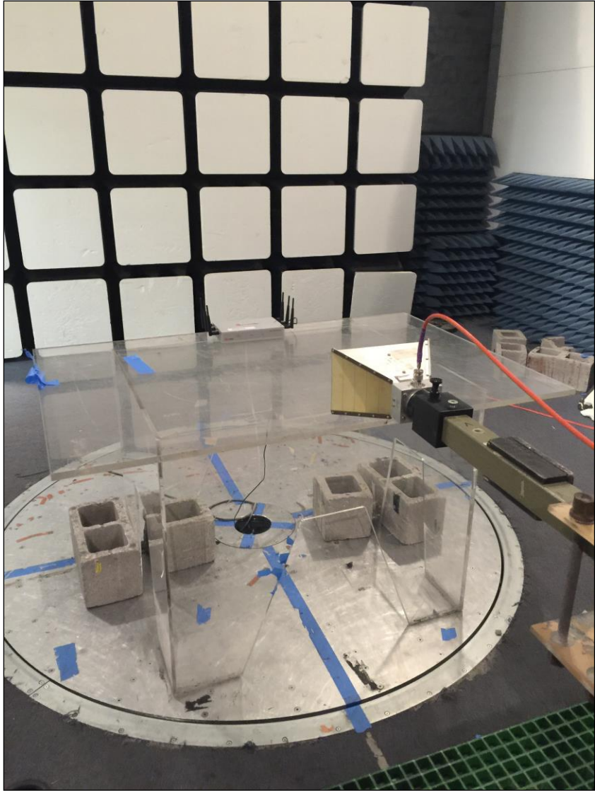
Photograph 2. Radiated Spurious Emissions, Test Setup, 1 GHz -18 GHz
