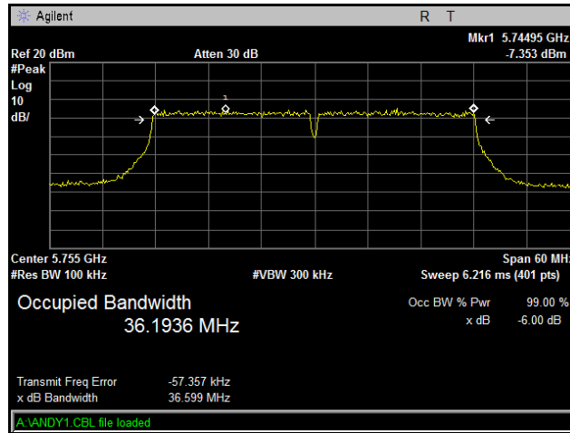
Plot 77. Occupied Band Width, Low Channel, 802.11n 40 MHz, Port R23
