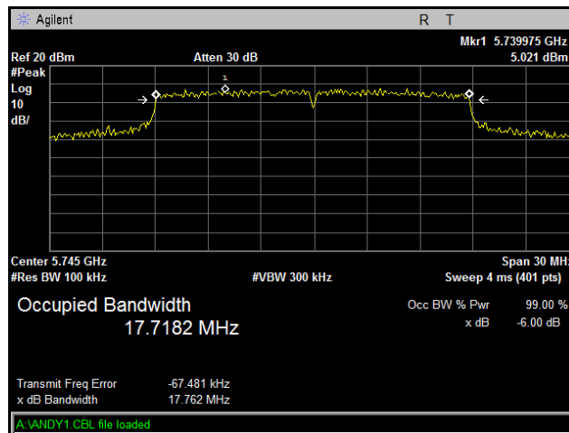
Plot 60. Occupied Band Width, Low Channel, 802.11n 20 MHz, Port R22
