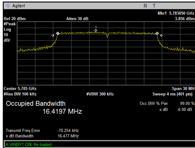
Plot 50. Occupied Band Width, Mid Channel, 802.11a 20 MHz, Port R13
