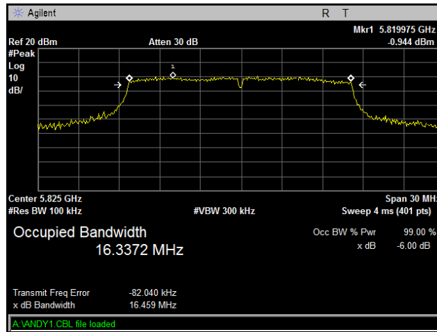
Plot 53. Occupied Band Width, High Channel, 802.11a 20 MHz, Port R23
