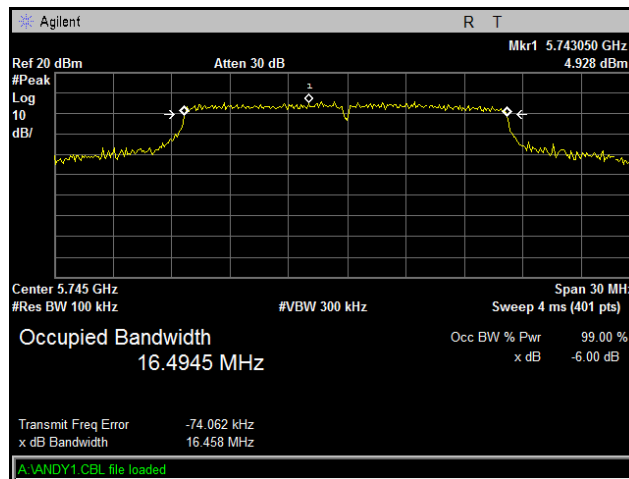
Plot 42. Occupied Band Width, Low Channel, 802.11a 20 MHz, Port R13
