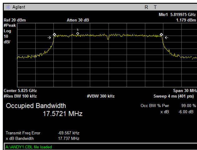
Plot 76. Occupied Band Width, High Channel, 802.11n 20 MHz, Port R13
