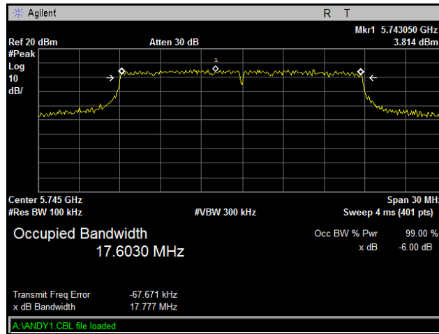
Plot 62. Occupied Band Width, Low Channel, 802.11n 20 MHz, Port R13
