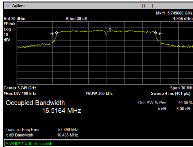
Plot 44. Occupied Band Width, Low Channel, 802.11a 20 MHz, Port R11
