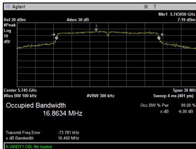
Plot 43. Occupied Band Width, Low Channel, 802.11a 20 MHz, Port R12
