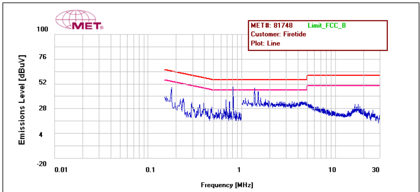
Plot 39. Conducted Emissions, Phase Line
