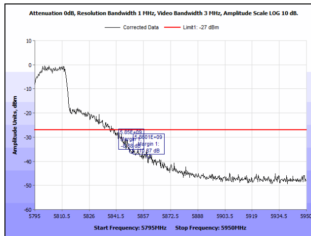
Plot 38. Restricted band of operation, 802.11n, 40 MHz, 5795Mhz
