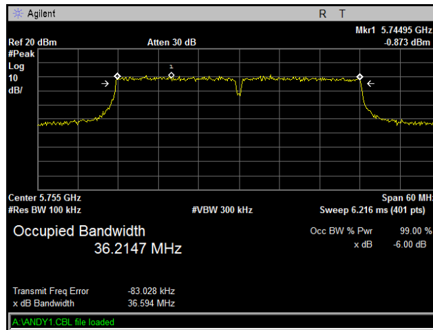
Plot 78. Occupied Band Width, Low Channel, 802.11n 40 MHz, Port R22
