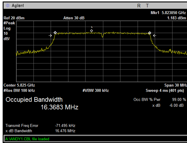
Plot 56. Occupied Band Width, High Channel, 802.11a 20 MHz, Port R13
