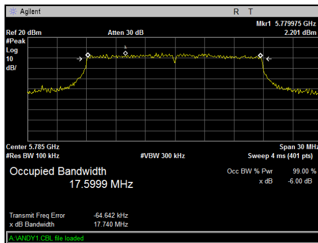
Plot 70. Occupied Band Width, Mid Channel, 802.11n 20 MHz, Port R11
