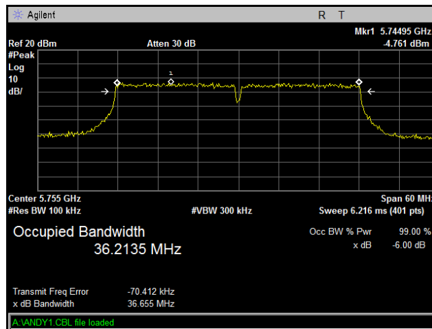
Plot 79. Occupied Band Width, Low Channel, 802.11n 40 MHz, Port R21
