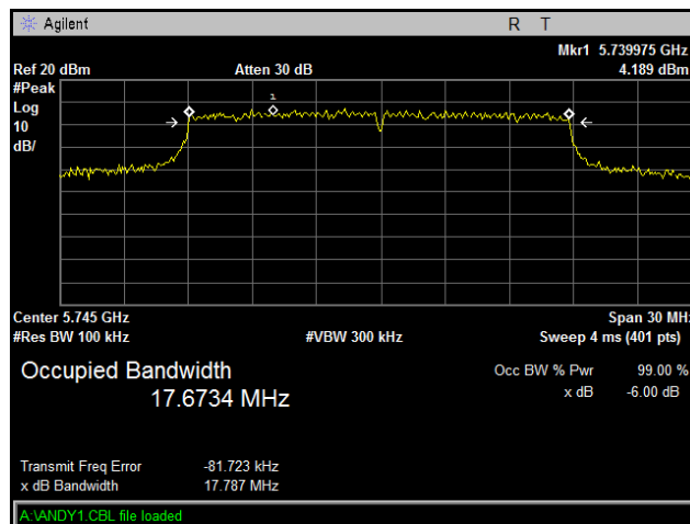
Plot 61. Occupied Band Width, Low Channel, 802.11n 20 MHz, Port R21
