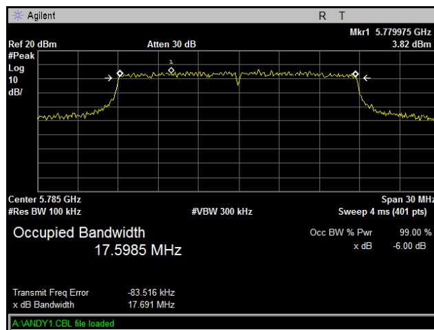
Plot 67. Occupied Band Width, Mid Channel, 802.11n 20 MHz, Port R21
