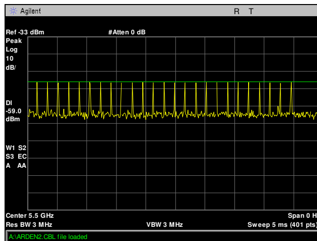
Plot 7. DFS Calibration, Radar Type 2, 5500 MHz
