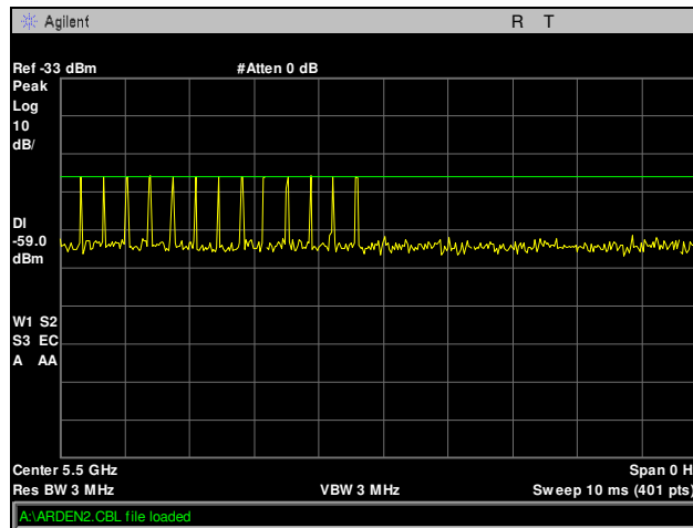
Plot 9. DFS Calibration, Radar Type 4, 5500 MHz
