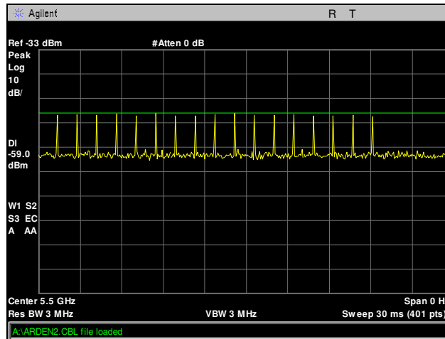
Plot 5. DFS Calibration, Radar Type 0, 5500 MHz
