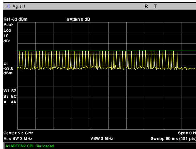
Plot 6. DFS Calibration, Radar Type 1, 5500 MHz
