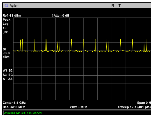
Plot 10. DFS Calibration, Radar Type 5, 5500 MHz
