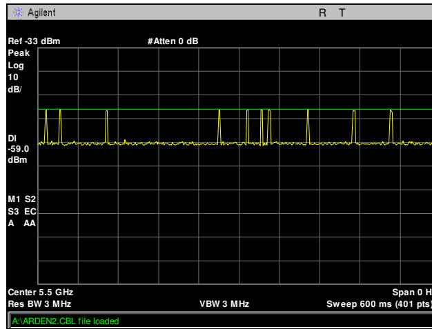
Plot 11. DFS Calibration, Radar Type 6, 5500 MHz
