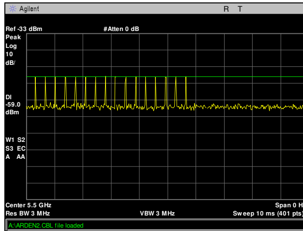
Plot 8. DFS Calibration, Radar Type 3, 5500 MHz
