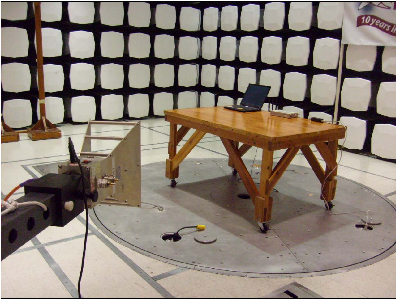
Radiated Emission, Test Setup, 1 GHz – 6 GHz
