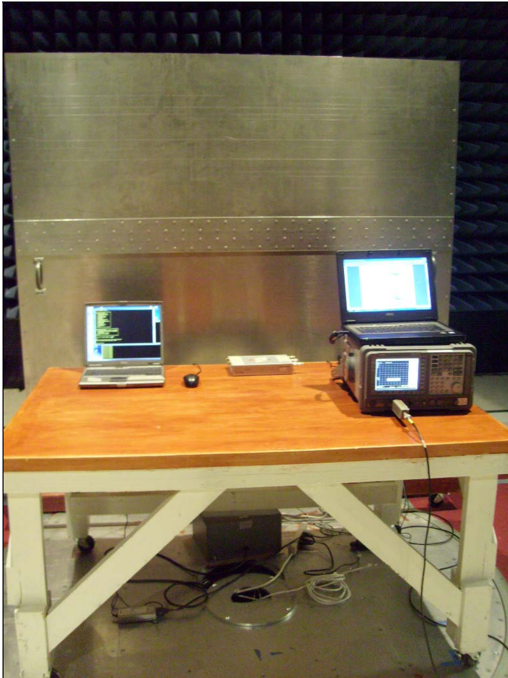
Conducted Emissions, Test Setup. Front View
