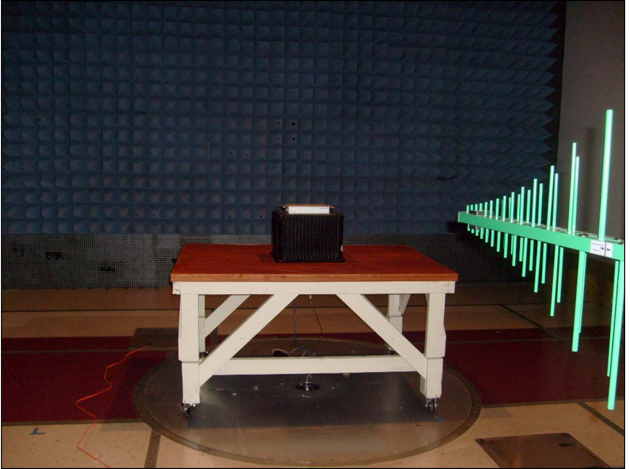
Photograph 2. Radiated Emission Spurious Test Setup, 2
