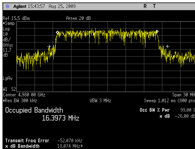
Plot 32. Occupied Bandwidth, 802.11a, High Channel, 20 MHz
