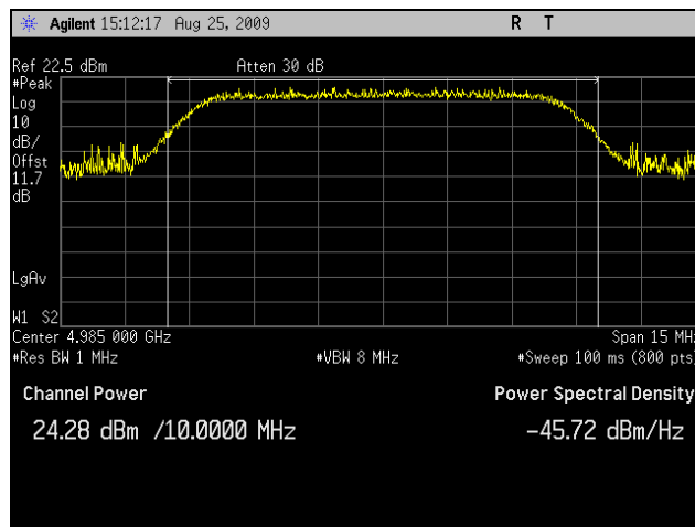
Plot 6. RF Power Output, Mid Channel, 802.11a, High Channel, 10 MHz
