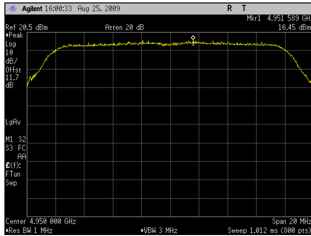
Plot 15. Peak Spectral Density, 802.11a, Low Channel, 20 MHz
