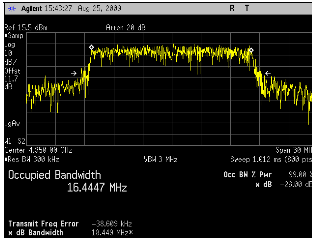
Plot 31. Occupied Bandwidth, 802.11a, Low Channel, 20 MHz
