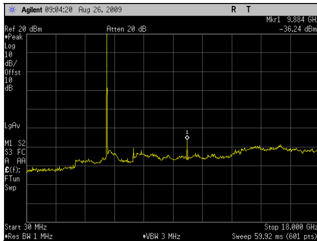
Plot 33. Conducted Spurious Emissions, Low Channel, 5 MHz (30 MHz – 18 GHz)
