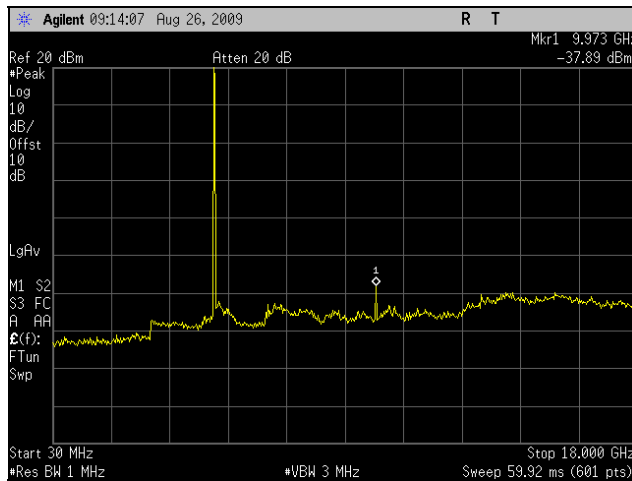
Plot 39. Conducted Spurious Emissions, High Channel, 5 MHz (30 MHz - 18GHz)
