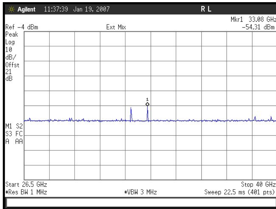
Plot 28. Conducted Spurious Emissions 5 MHz Low Ch (26.5 GHz – 40 GHz)
