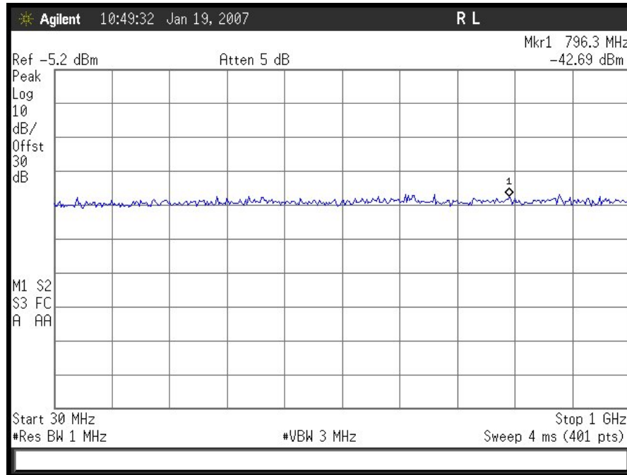
Plot 32. Conducted Spurious Emissions 5 MHz Hi Ch (30 MHz - 1GHz)
