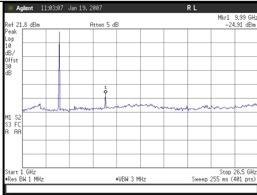
Plot 42. Conducted Spurious Emissions 10 MHz Hi Ch (1 GHz – 26.5 GHz)
