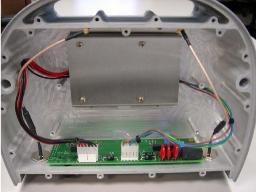
Top View with Motherboard, Daughtercard Removed
