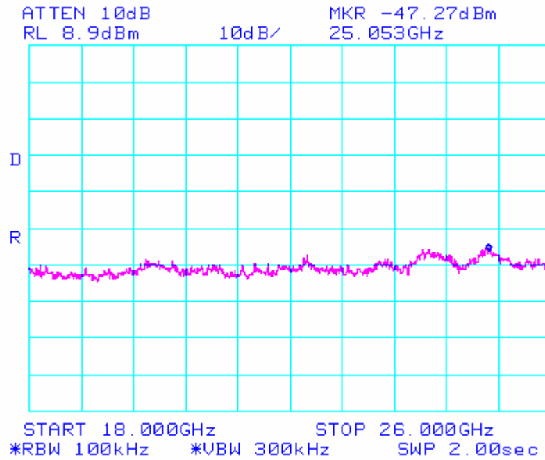
802.11/b – High Channel Conducted Emissions 18-26GHz
