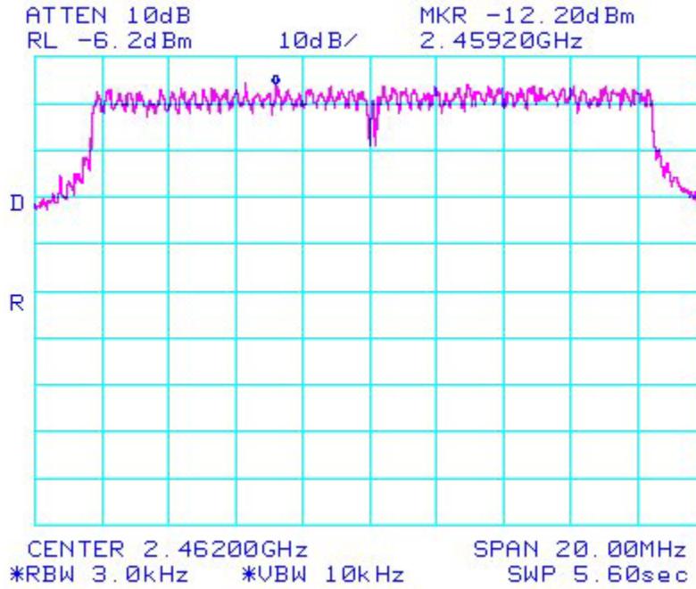
802.11/g – High Ch Peak Power Spectral Density
