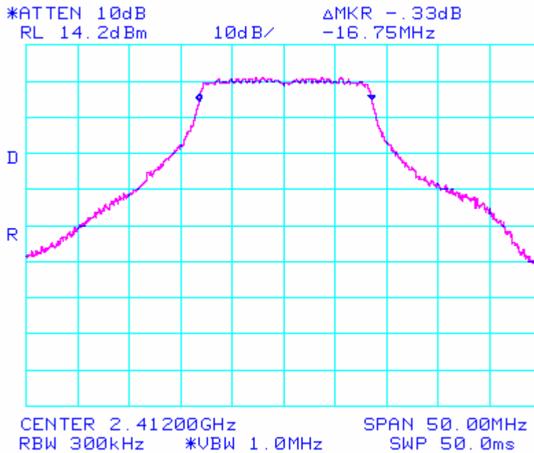
802.11/g Low Ch Occupied Band Width
