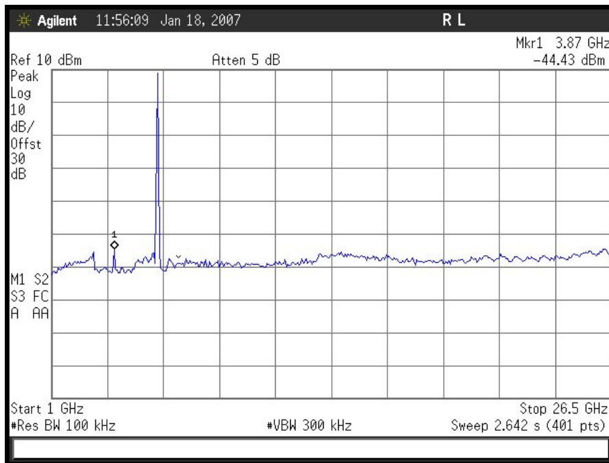
802.11/a – High Channel Conducted Emissions 1-26.5GHz
