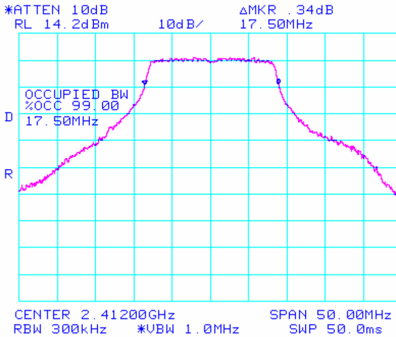
802.11/g Low Ch Occupied Band Width 99%
