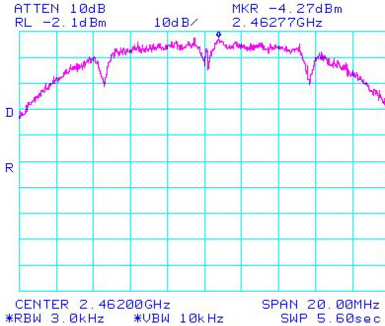
802.11/b – High Ch Peak Power Spectral Density
