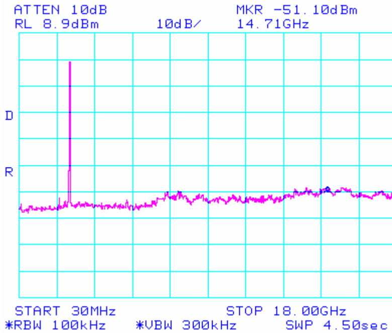
802.11/g – High Channel Conducted Emissions 30MHz- 18GHz
