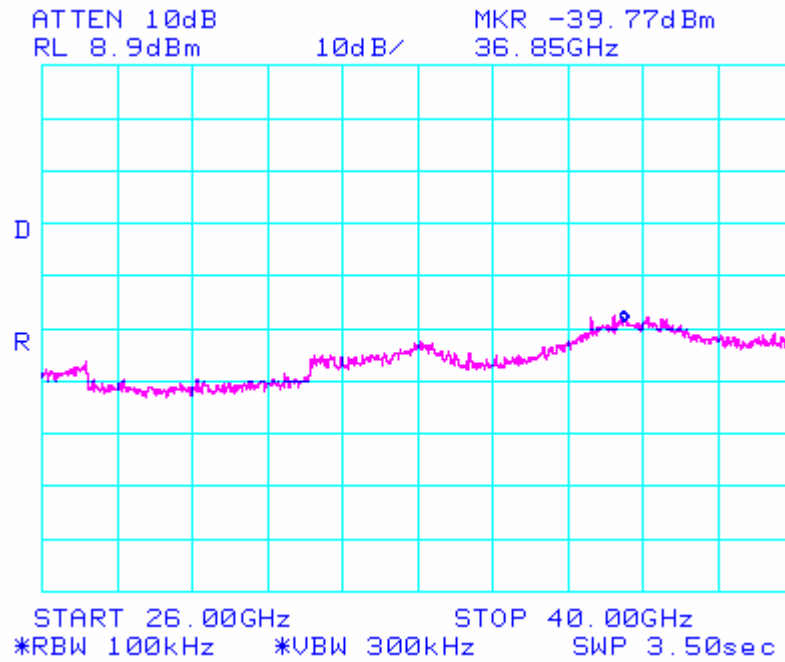
802.11/b – High Channel Conducted Emissions 26-40GHz
