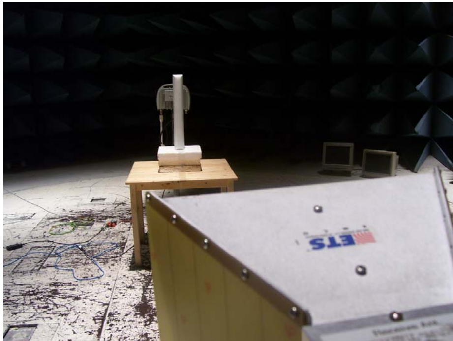
Photograph 7. Test Equipment and setup for various Radiated Measurements
