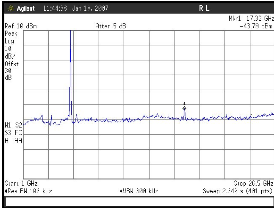
802.11/a – Mid Channel Conducted Emissions 1-26.5GHz
