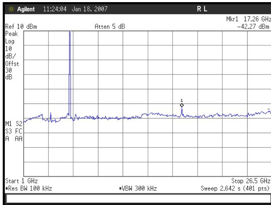
802.11/a – Low Channel Conducted Emissions 1-26.5GHz
