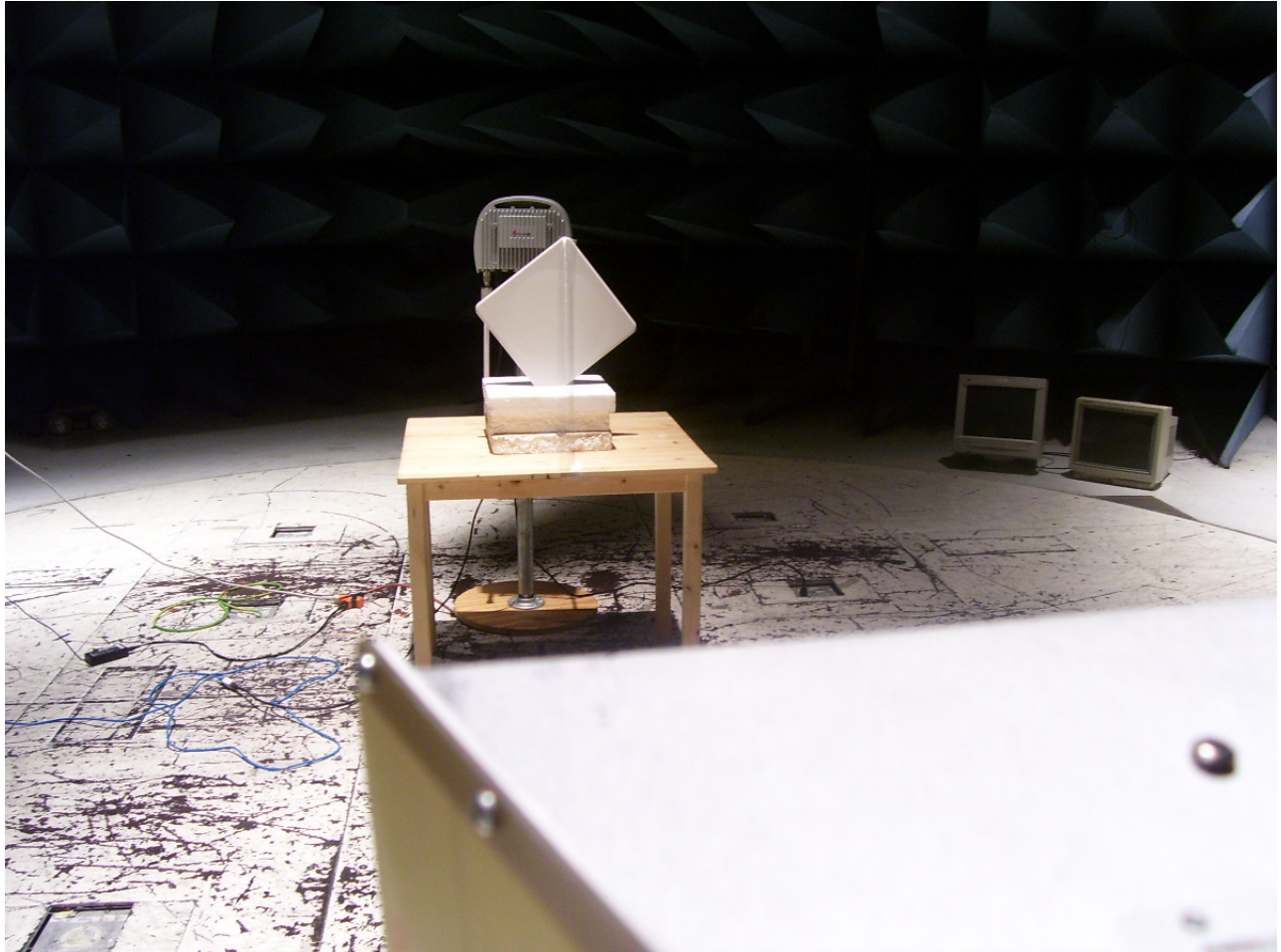
Photograph 8. Test Equipment and setup for various Radiated Measurements
