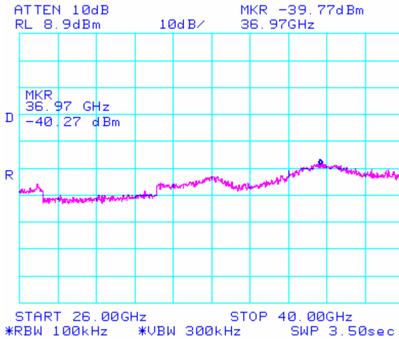
802.11/g – Low Channel Conducted Emissions 26-40GHz
