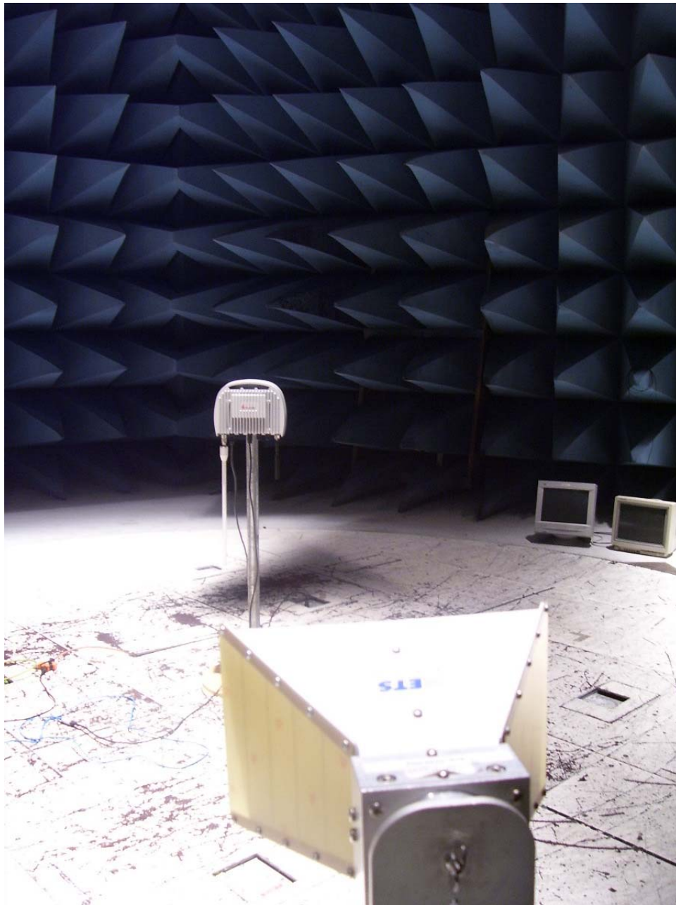
Photograph 1. Test Equipment and setup for various Radiated Measurements 5dbi Omni
