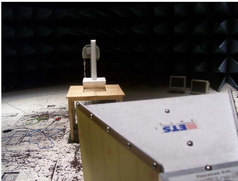
Photograph 3. Test Equipment and setup for various Radiated Measurements 16dbi Sector
