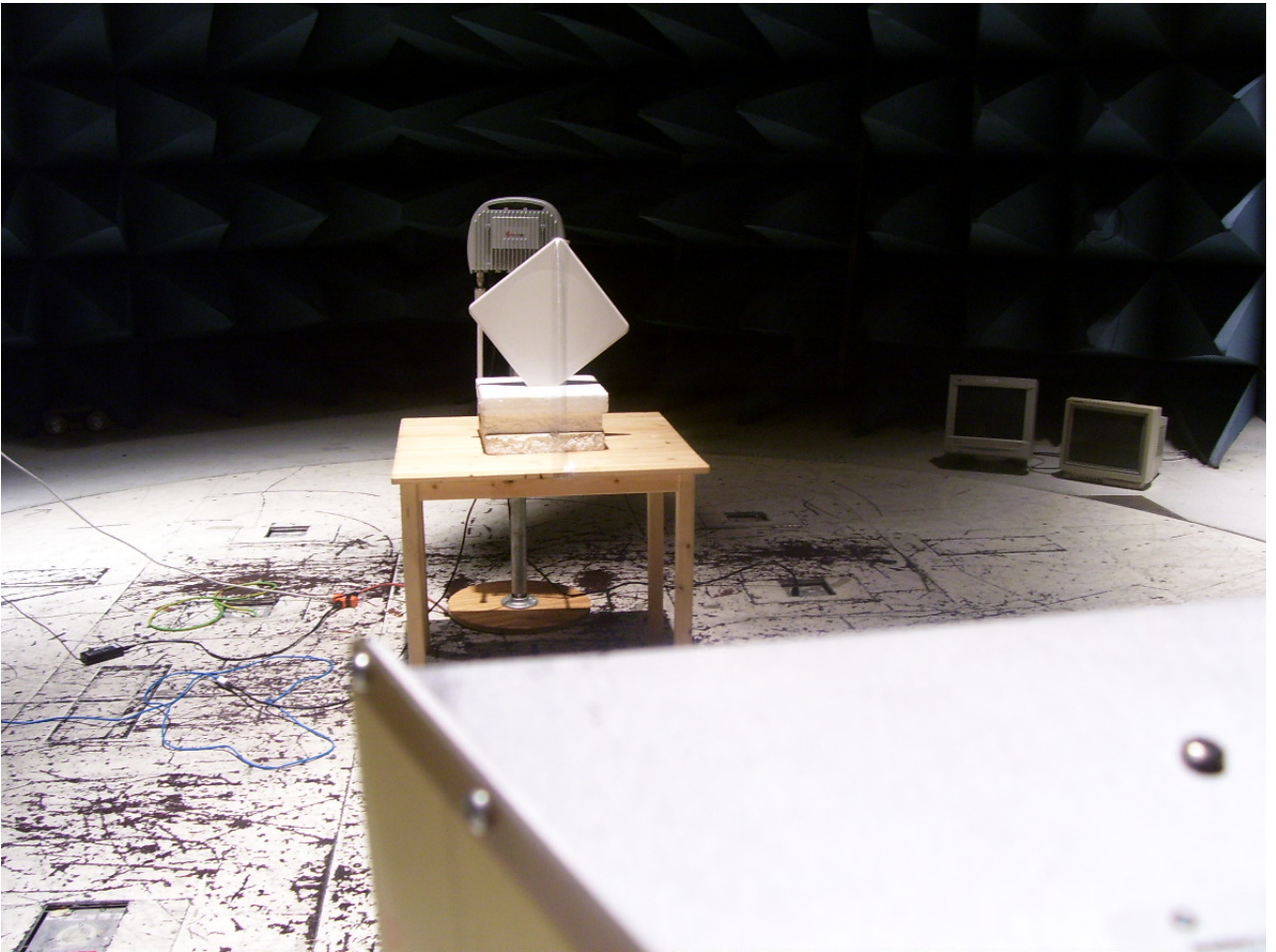
Photograph 4. Test Equipment and setup for various Radiated Measurements 23dBi Panel
