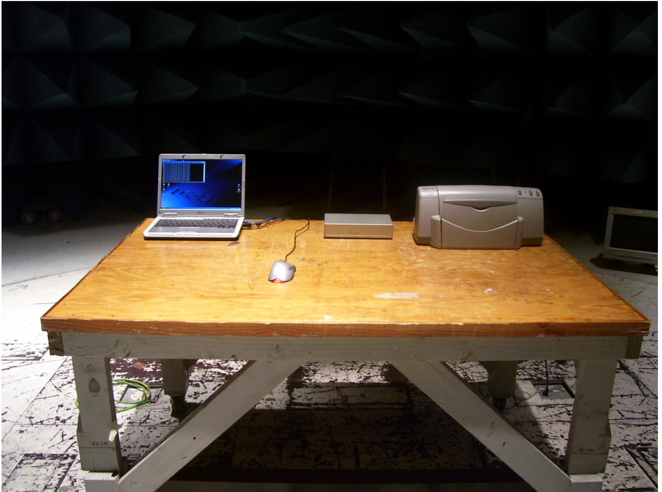
Radiated Emission Test Setup 30 MHz - 1 GHz
