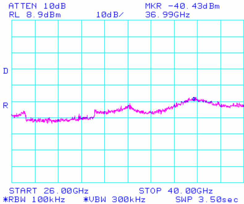
802.11/b – Low Channel Conducted Emissions 26 – 40GHz
