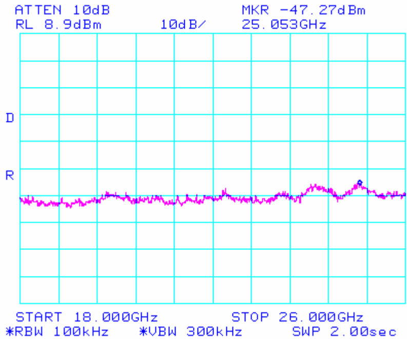
802.11/b – High Channel Conducted Emissions 18-26GHz
