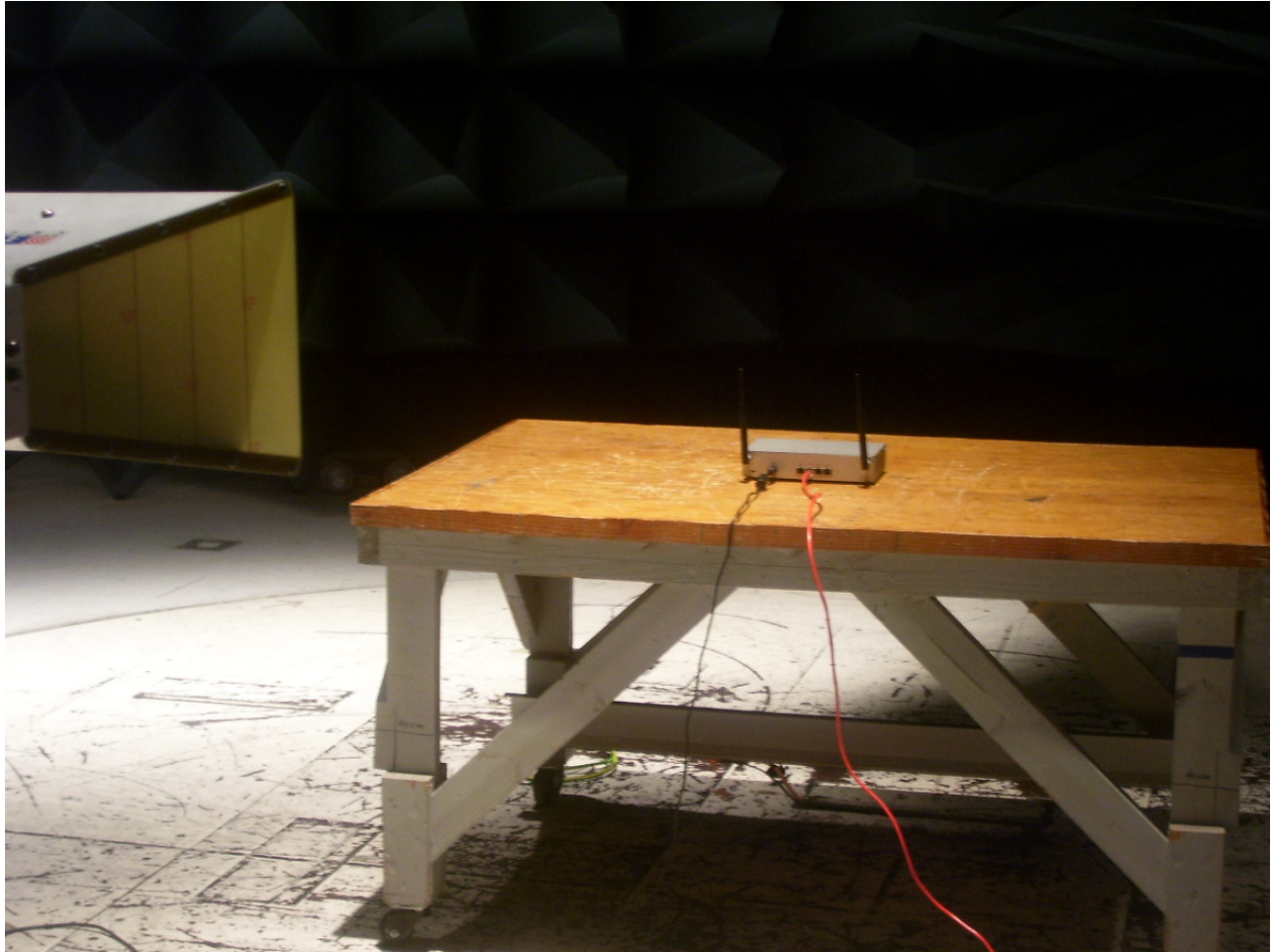
Photograph 5. Test Equipment and setup for various Radiated Measurements (5dbi Omni Antenna)
