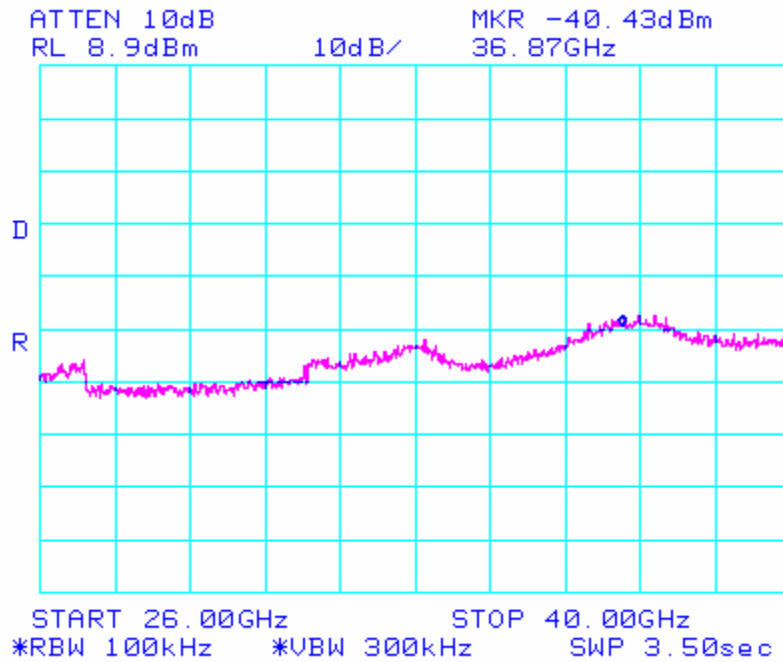
802.11/g – High Channel Conducted Emissions 26 – 40GHz
