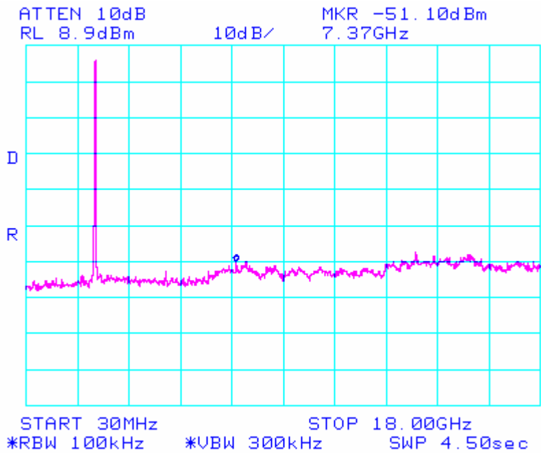
802.11/b – High Channel Conducted Emissions 30MHz- 18GHz
