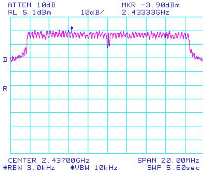
802.11/g – Mid Ch Peak Power Spectral Density
