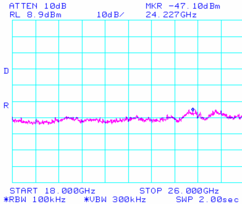
802.11/g – High Channel Conducted Emissions 18-26GHz
