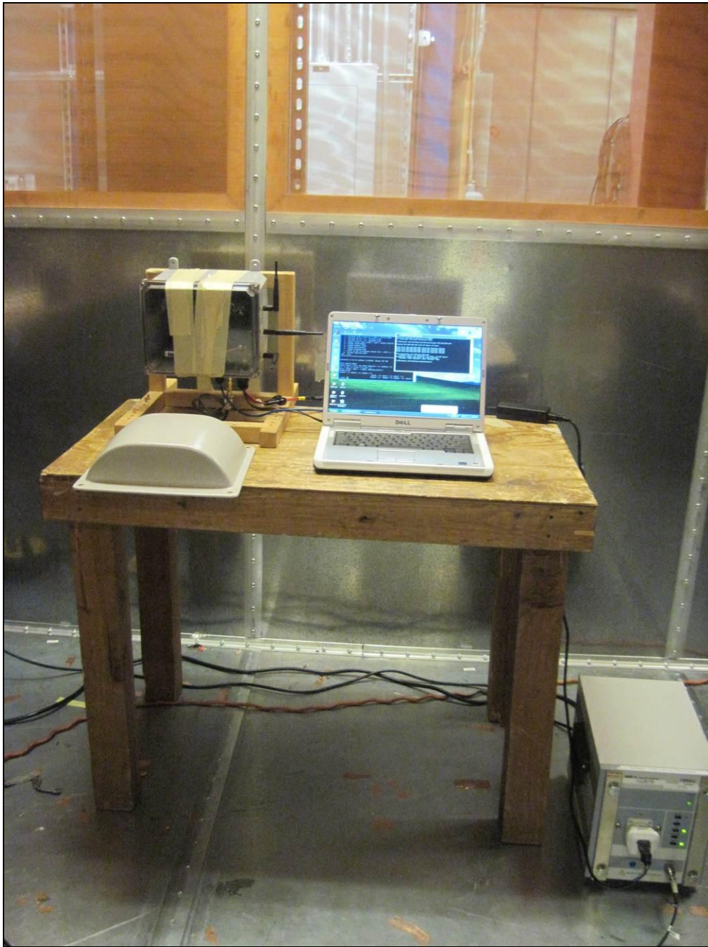
Photograph 4. Conducted Emissions, 15.207(a), Test Setup, 2.4 GHz
