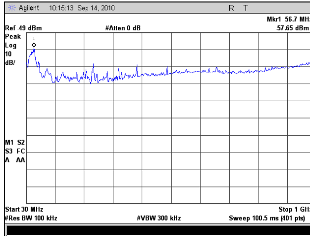
Plot 65. Radiated Spurious Emissions, Low Channel, 5 MHz (30 MHz – 1 GHz)
