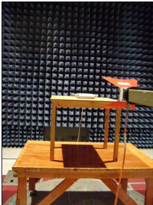
Photograph 3 Radiated Emission Spurious Test Setup, 1 GHz – 18 GHz
