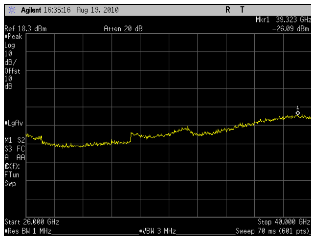
Plot 52. Conducted Spurious Emissions, Mid Channel, 10 MHz (26 GHz – 40 GHz)
