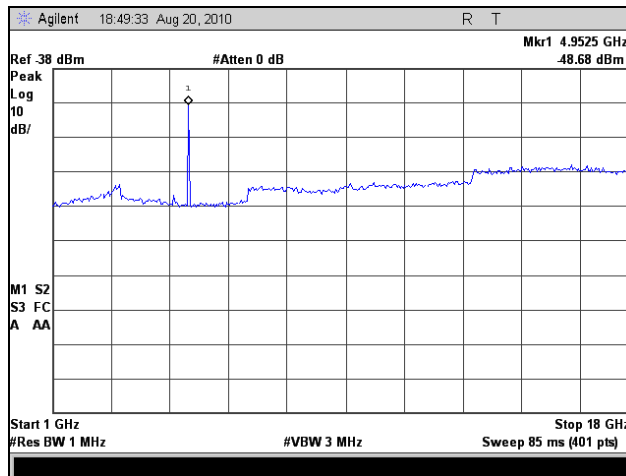
Plot 66. Radiated Spurious Emissions, Low Channel, 5 MHz (1 GHz – 18 GHz)
