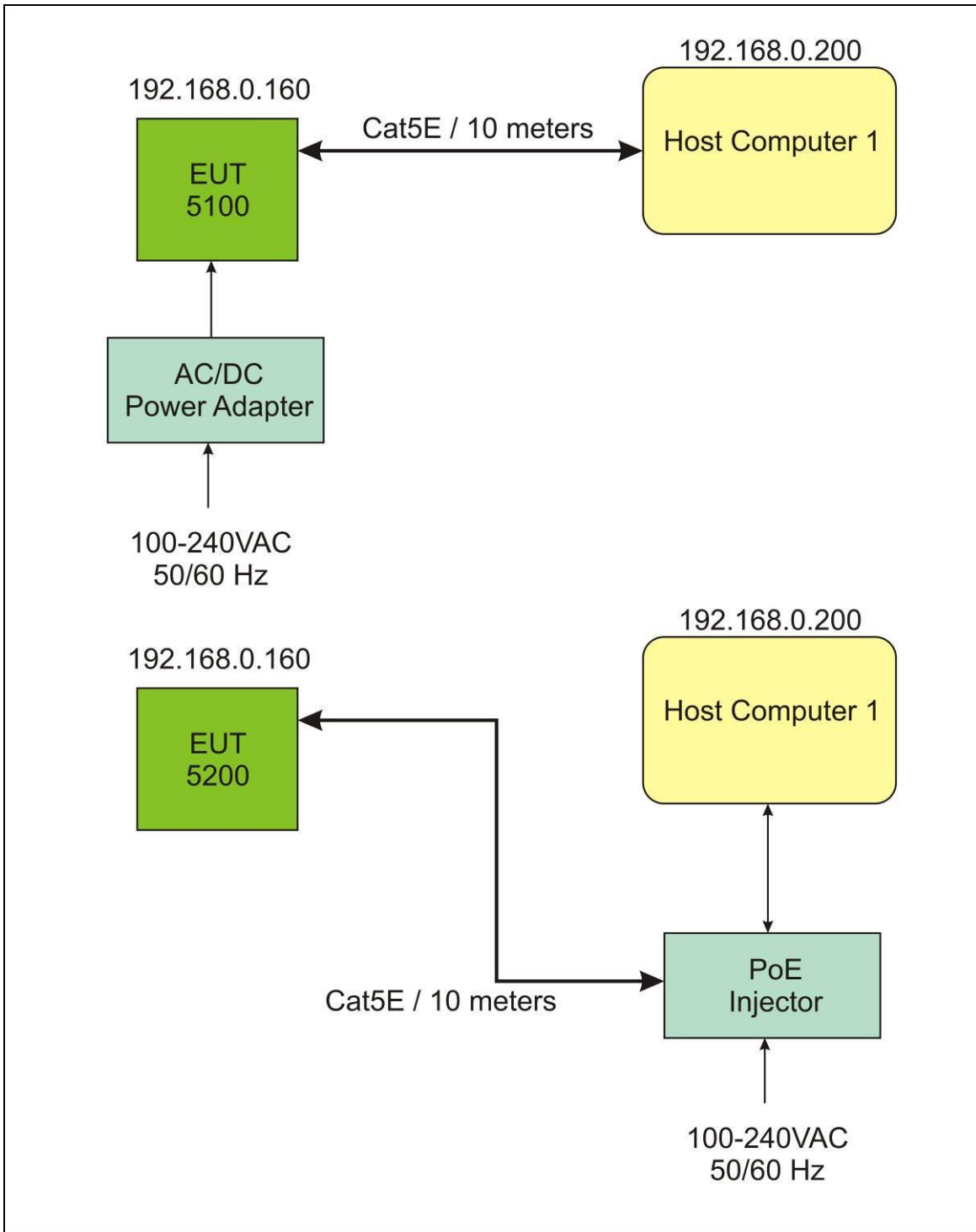
Figure 2. Setup Block Diagram
