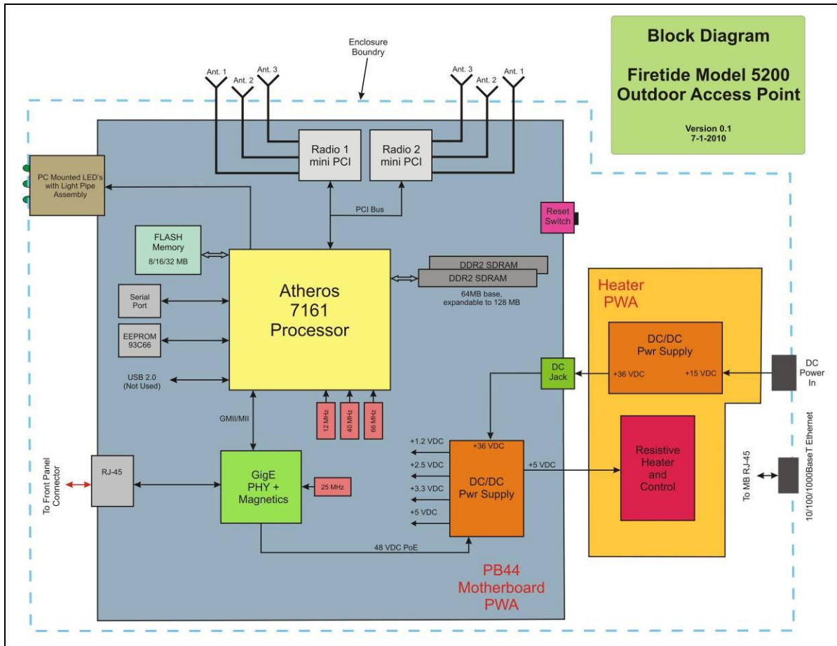
Figure 1. Block Diagram of Equipment Configuration
