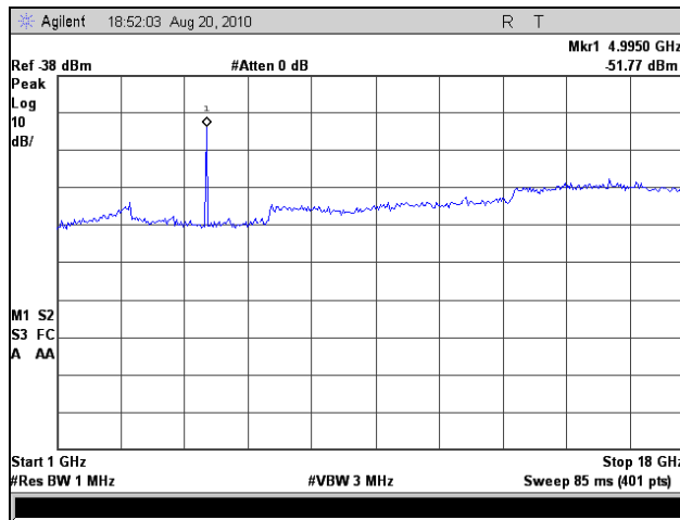
Plot 74. Radiated Spurious Emissions, Mid Channel, 10 MHz (1 GHz – 18 GHz)
