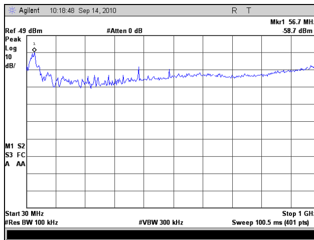
Plot 69. Radiated Spurious Emissions, High Channel, 5 MHz (30 MHz – 1 GHz)
