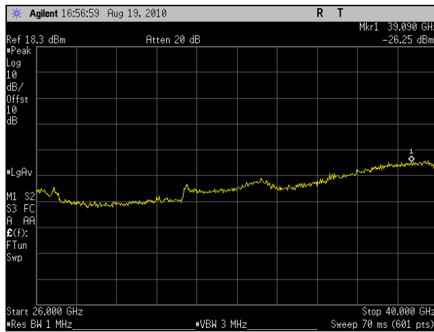
Plot 64. Conducted Spurious Emissions, High Channel, 20 MHz (26 GHz – 40 GHz)
