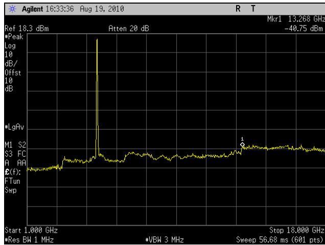
Plot 54. Conducted Spurious Emissions, High Channel, 10 MHz (1 GHz – 18 GHz)
