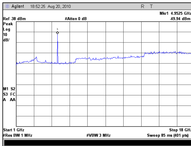
Plot 72. Radiated Spurious Emissions, Low Channel, 10 MHz (1 GHz – 18 GHz)
