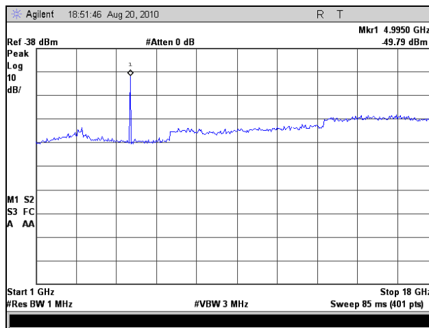
Plot 76. Radiated Spurious Emissions, High Channel, 10 MHz (1 GHz – 18 GHz)
