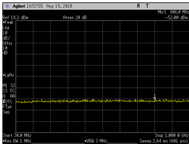
Plot 61. Conducted Spurious Emissions, High Channel, 20 MHz (30 MHz – 1 GHz)
