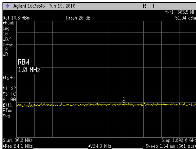
Plot 37. Conducted Spurious Emissions, Mid Channel, 5 MHz (30 MHz – 1 GHz)
