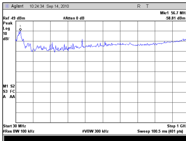
Plot 79. Radiated Spurious Emissions, High Channel, 20 MHz (30 MHz – 1 GHz)
