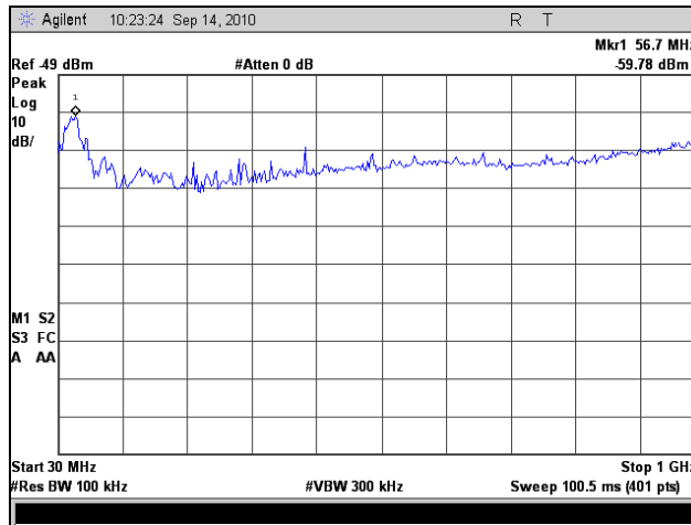
Plot 77. Radiated Spurious Emissions, Low Channel, 20 MHz (30 MHz – 1 GHz)
