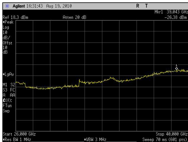
Plot 44. Conducted Spurious Emissions, High Channel, 5 MHz (26 GHz – 40 GHz)
