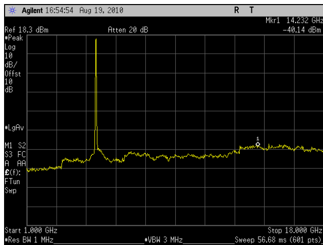
Plot 58. Conducted Spurious Emissions, Low Channel, 20 MHz (1 GHz – 18 GHz)
