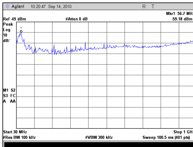
Plot 73. Radiated Spurious Emissions, Mid Channel, 10 MHz (30 MHz – 1 GHz)
