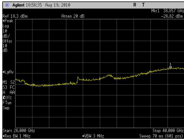
Plot 60. Conducted Spurious Emissions, Low Channel, 20 MHz (26 GHz – 40 GHz)
