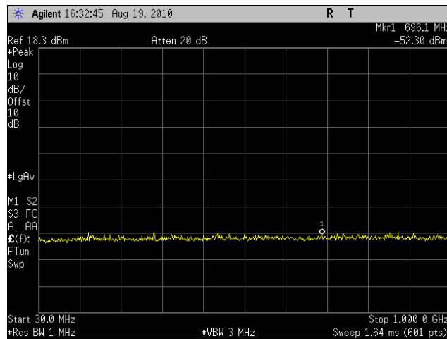
Plot 41. Conducted Spurious Emissions, High Channel, 5 MHz (30 MHz – 1 GHz)
