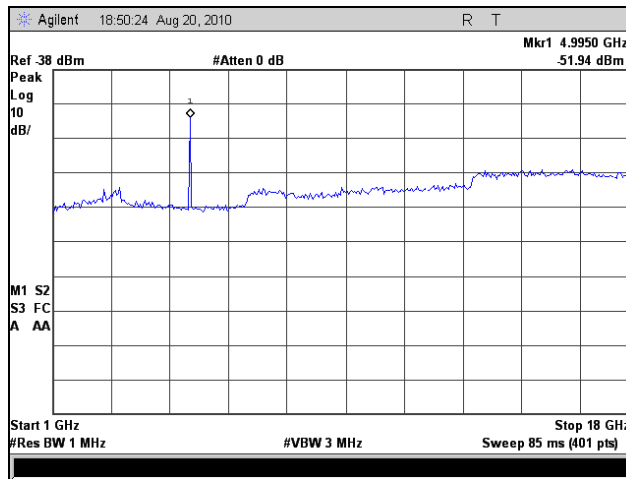
Plot 68. Radiated Spurious Emissions, Mid Channel, 5 MHz (1 GHz – 18 GHz)
