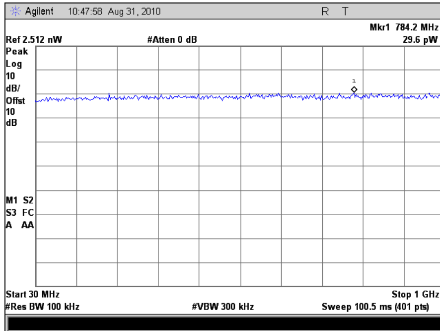
Plot 81. Conducted Receiver Spurious Emissions, 30 MHz – 1 GHz
