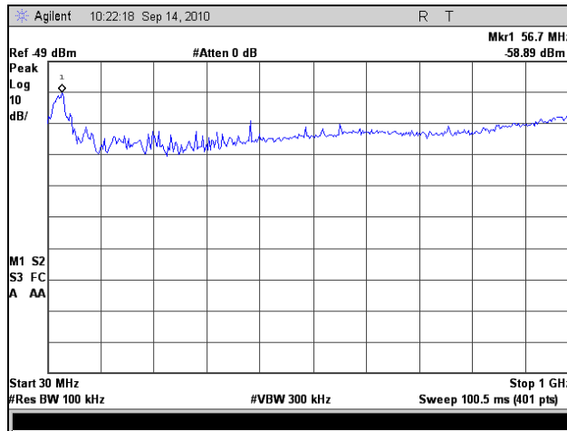
Plot 71. Radiated Spurious Emissions, Low Channel, 10 MHz (30 MHz – 1 GHz)
