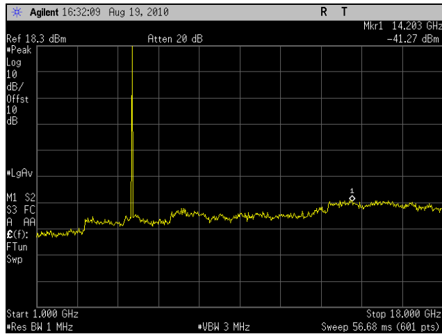
Plot 42. Conducted Spurious Emissions, High Channel, 5 MHz (1 GHz – 18 GHz)
