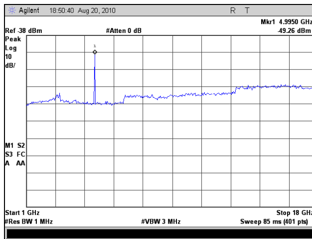
Plot 70. Radiated Spurious Emissions, High Channel, 5 MHz (1 GHz – 18 GHz)
