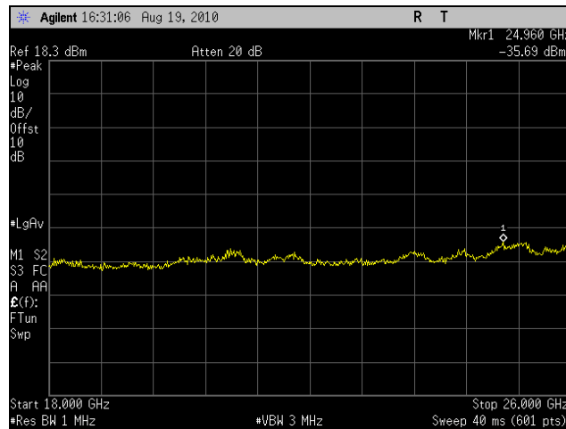
Plot 39. Conducted Spurious Emissions, Mid Channel, 5 MHz (18 GHz – 26 GHz)
