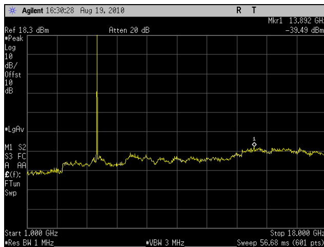
Plot 38. Conducted Spurious Emissions, Mid Channel, 5 MHz (1 GHz – 18 GHz)
