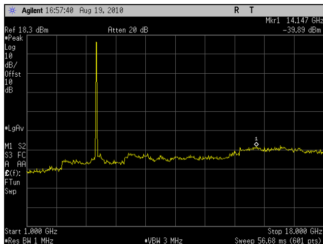
Plot 62. Conducted Spurious Emissions, High Channel, 20 MHz (1 GHz – 18 GHz)
