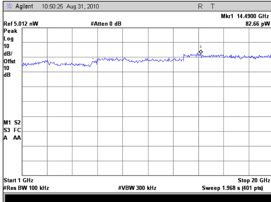
Plot 82. Conducted Receiver Spurious Emissions, 1 GHz – 20 GHz
