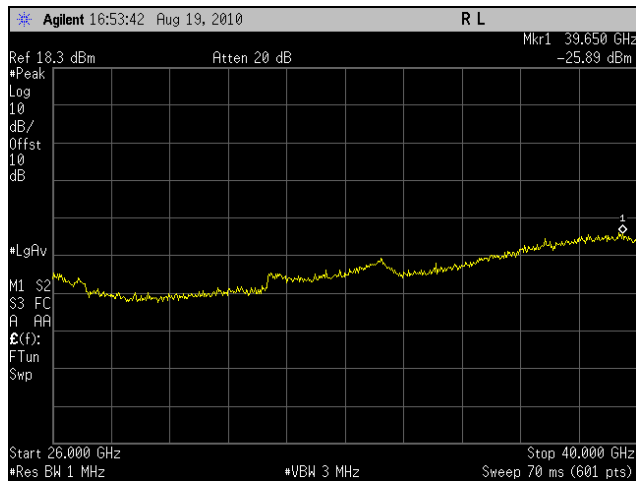
Plot 48. Conducted Spurious Emissions, Low Channel, 10 MHz (26 GHz – 40 GHz)
