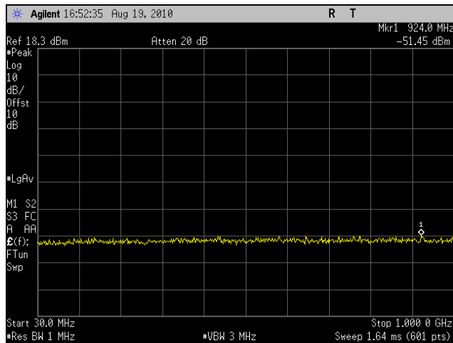
Plot 45. Conducted Spurious Emissions, Low Channel, 10 MHz (30 MHz – 1 GHz)
