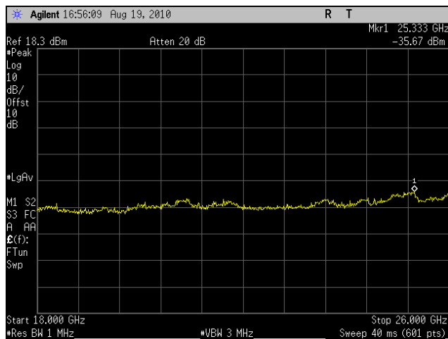
Plot 59. Conducted Spurious Emissions, Low Channel, 20 MHz (18 GHz – 26 GHz)
