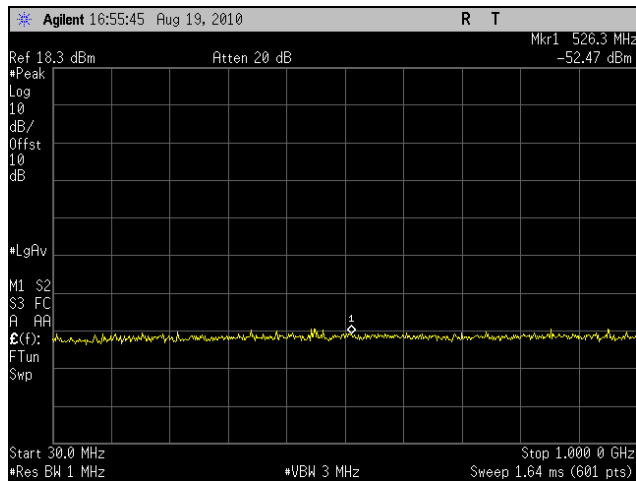
Plot 57. Conducted Spurious Emissions, Low Channel, 20 MHz (30 MHz – 1 GHz)
