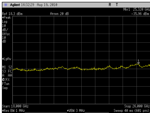
Plot 43. Conducted Spurious Emissions, High Channel, 5 MHz (18 GHz – 26 GHz)
