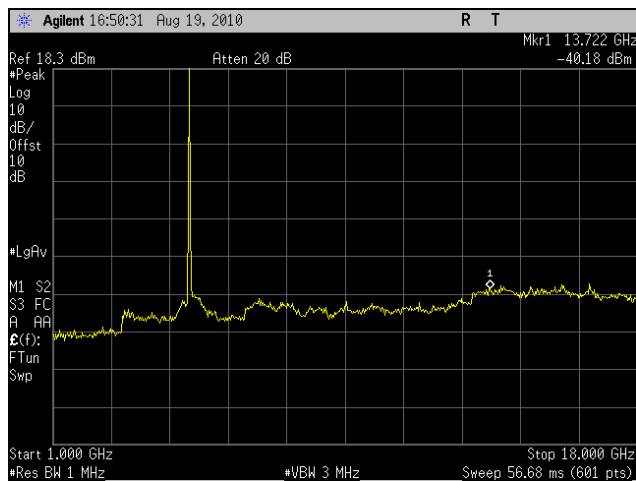
Plot 50. Conducted Spurious Emissions, Mid Channel, 10 MHz (1 GHz – 18 GHz)
