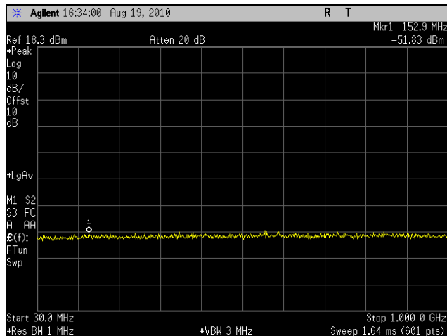
Plot 53. Conducted Spurious Emissions, High Channel, 10 MHz (30 MHz – 1 GHz)
