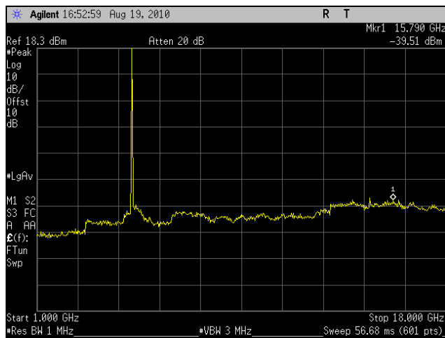
Plot 46. Conducted Spurious Emissions, Low Channel, 10 MHz (1 GHz – 18 GHz)
