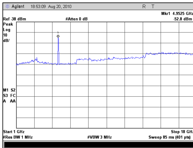
Plot 78. Radiated Spurious Emissions, Low Channel, 20 MHz (1 GHz – 18 GHz)
