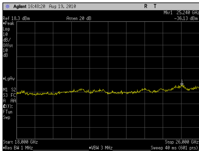
Plot 55. Conducted Spurious Emissions, High Channel, 10 MHz (18 GHz – 26 GHz)
