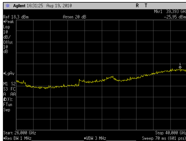
Plot 40. Conducted Spurious Emissions, Mid Channel, 5 MHz (26 GHz – 40 GHz)
