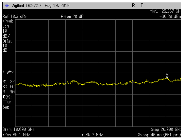
Plot 63. Conducted Spurious Emissions, High Channel, 20 MHz (18 GHz – 26 GHz)
