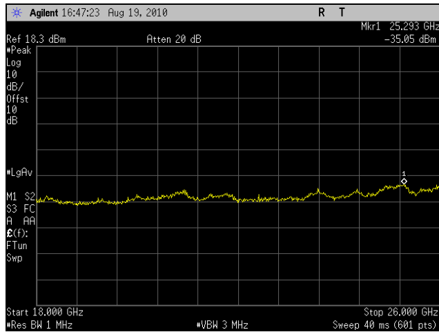
Plot 51. Conducted Spurious Emissions, Mid Channel, 10 MHz (18 GHz – 26 GHz)
