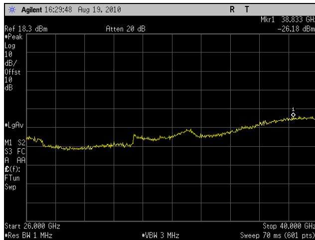
Plot 36. Conducted Spurious Emissions, Low Channel, 5 MHz (26 GHz – 40 GHz)
