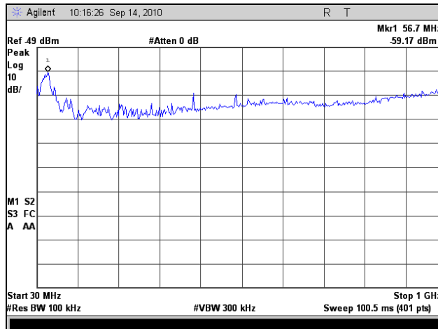
Plot 67. Radiated Spurious Emissions, Mid Channel, 5 MHz (30 MHz – 1 GHz)
