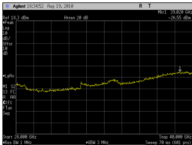
Plot 56. Conducted Spurious Emissions, High Channel, 10 MHz (26 GHz – 40 GHz)
