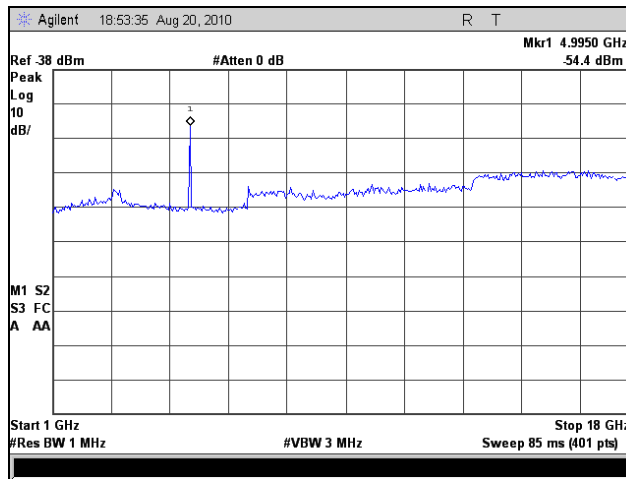
Plot 80. Radiated Spurious Emissions, High Channel, 20 MHz (1 GHz – 18 GHz)
