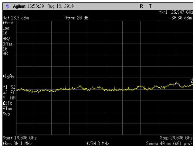
Plot 47. Conducted Spurious Emissions, Low Channel, 10 MHz (18 GHz – 26 GHz)
