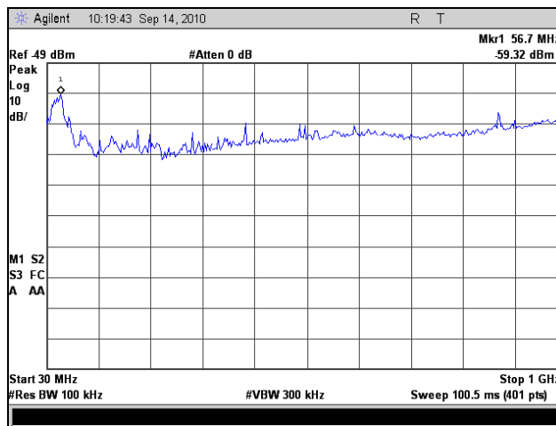
Plot 75. Radiated Spurious Emissions, High Channel, 10 MHz (30 MHz – 1 GHz)
