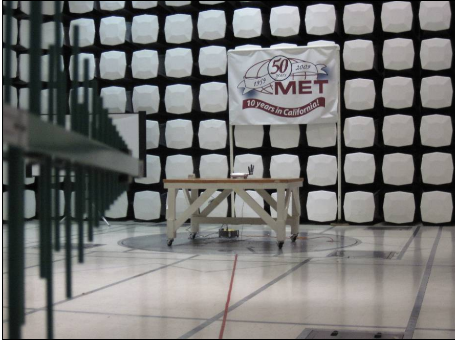
Photograph 7. Radiated Emission, Test Setup, 30 MHz – 1 GHz
