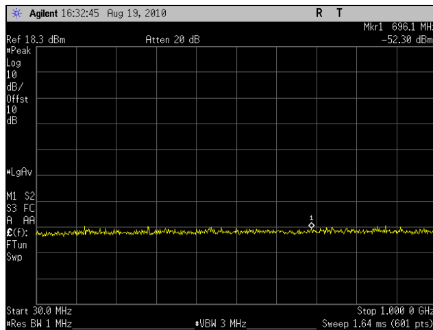
Plot 41. Conducted Spurious Emissions, High Channel, 5 MHz (30 MHz – 1 GHz)
