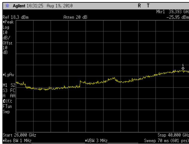
Plot 40. Conducted Spurious Emissions, Mid Channel, 5 MHz (26 GHz – 40 GHz)
