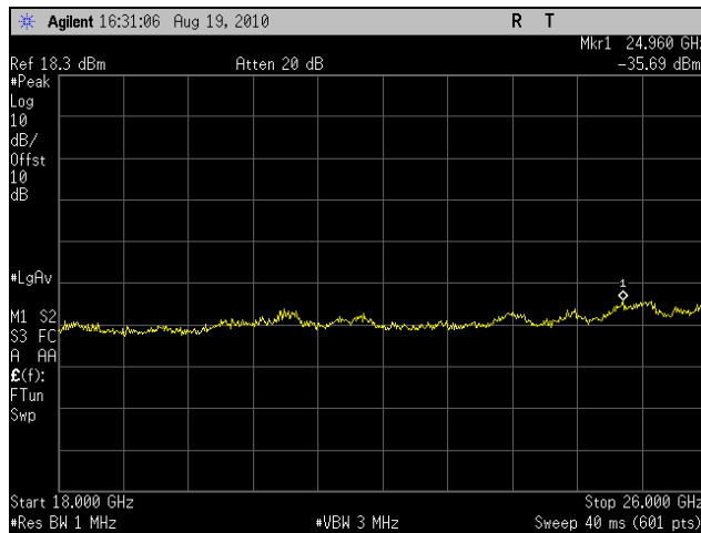
Plot 39. Conducted Spurious Emissions, Mid Channel, 5 MHz (18 GHz – 26 GHz)
