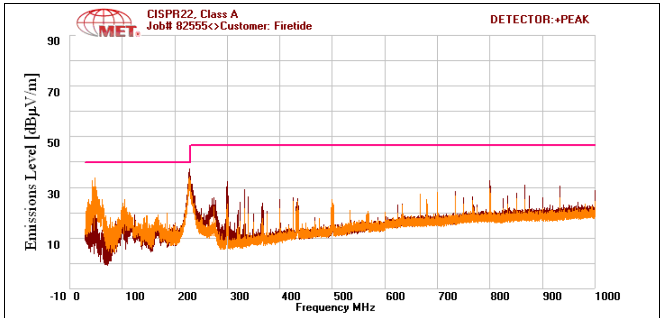
Plot 10. Radiated Emissions, ICES-003 Limits PoE30U-560
