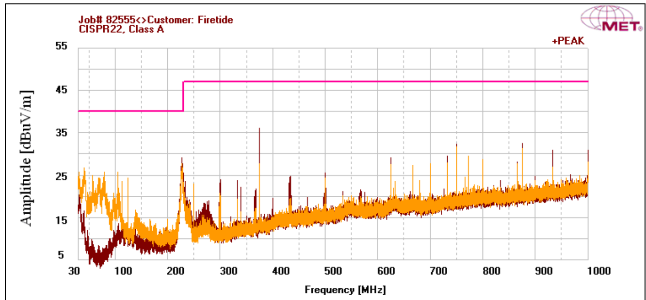
Plot 9. Radiated Emissions, ICES-003 Limits, FSP040-DGAA5
