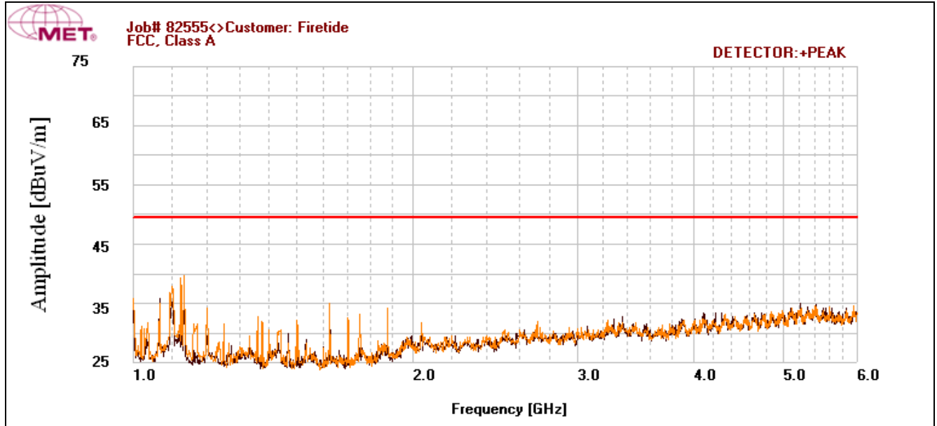
Plot 6. Radiated Emissions, 1 GHz – 6 GHz, FCC Limits, FSP040-DGAA5
