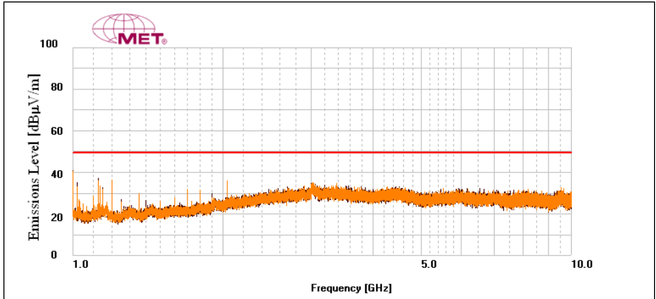
Plot 8. Radiated Emissions, 1 GHz – 10 GHz, FCC Limits, PoE30U-560
