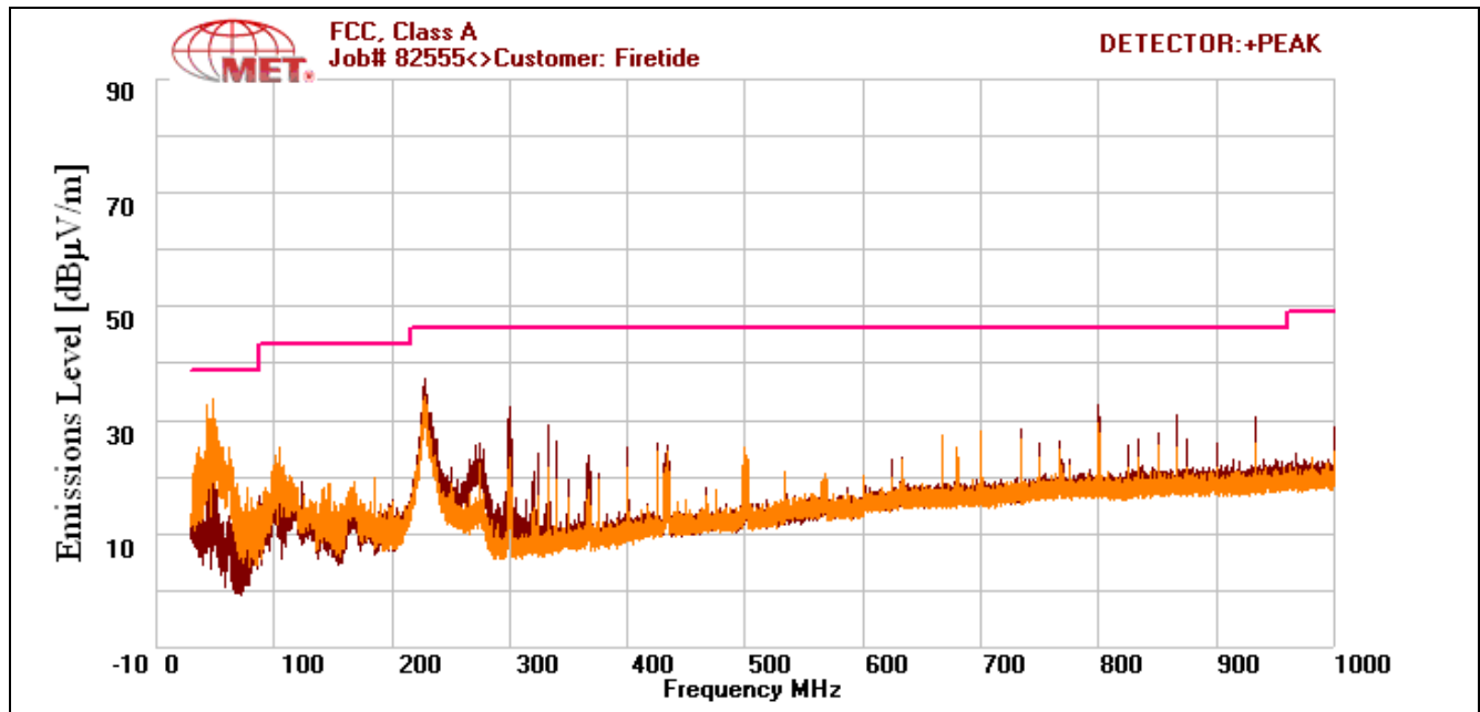
Plot 7. Radiated Emissions, 30 MHz - 1 GHz, FCC Limits, PoE30U-560
