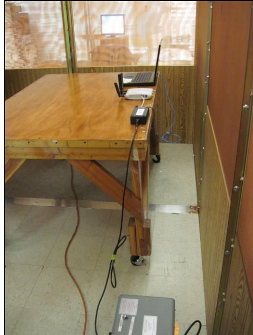
Photograph 5. Conducted Emissions, PoE30U-560, Test Setup 2
