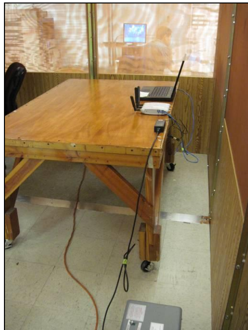
Photograph 3. Conducted Emissions, FSP040-DGAA5, Test Setup 2
