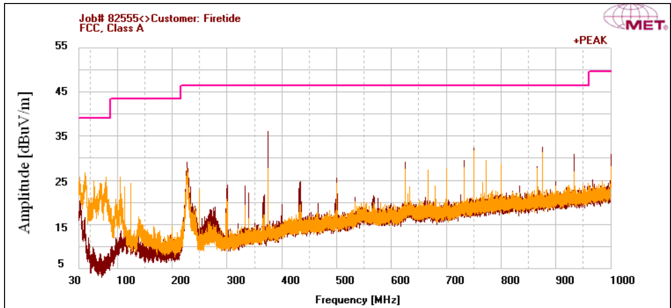
Plot 5. Radiated Emissions, 30 MHz - 1 GHz, FCC Limits, FSP040-DGAA5
